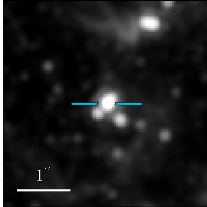
JWST/NIRCam F430M
