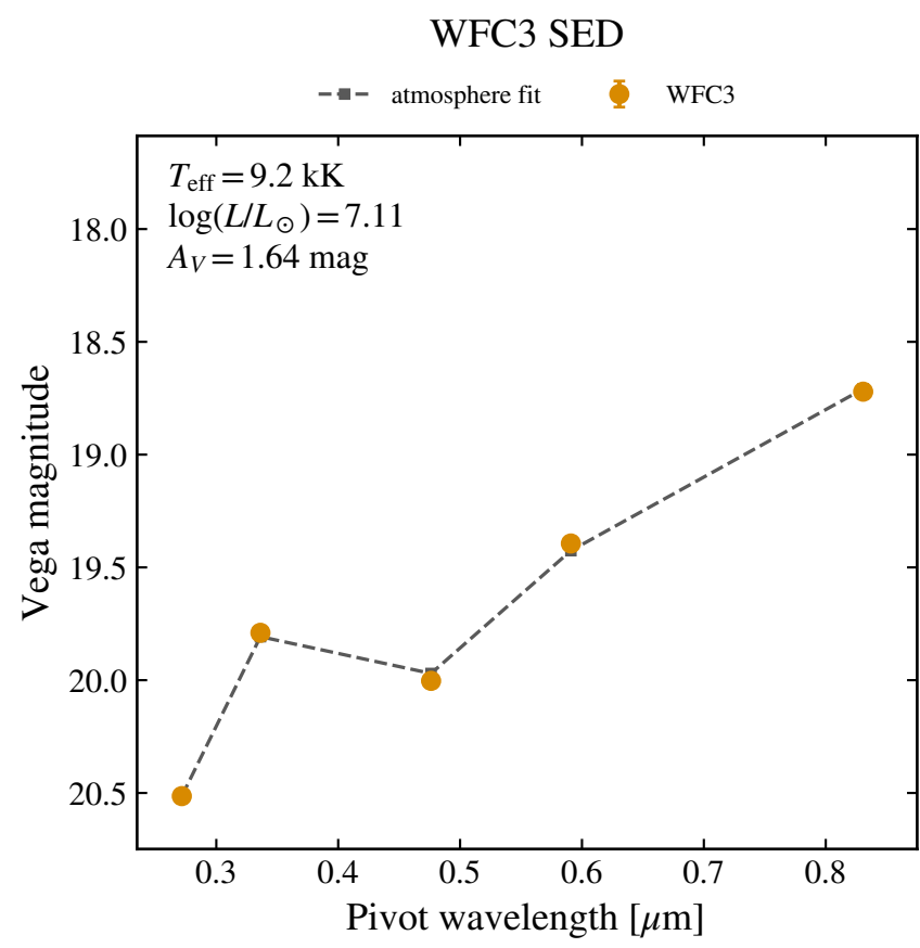
WFC3 F606W 19.394 ± 0.008
