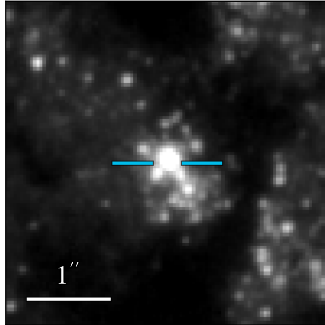
WFC3 F475W 20.003 ± 0.008
