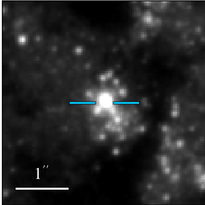
WFC3 F606W 19.394 ± 0.008
