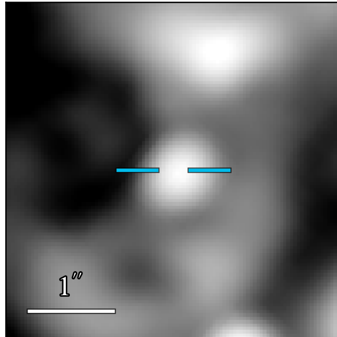
JWST/MIRI F1500W
