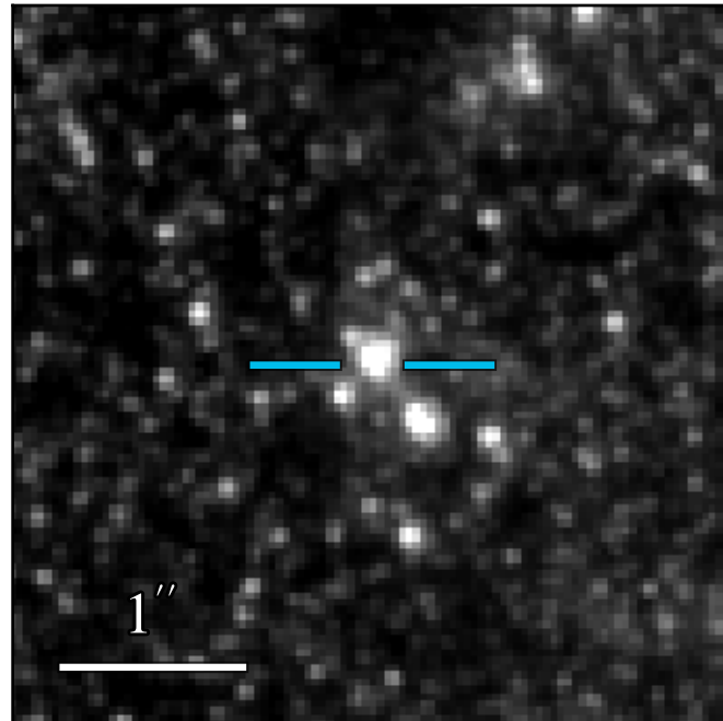
JWST/NIRCam F182M
