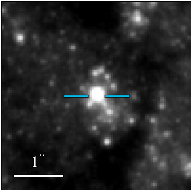
WFC3 F814W 18.721 ± 0.006
