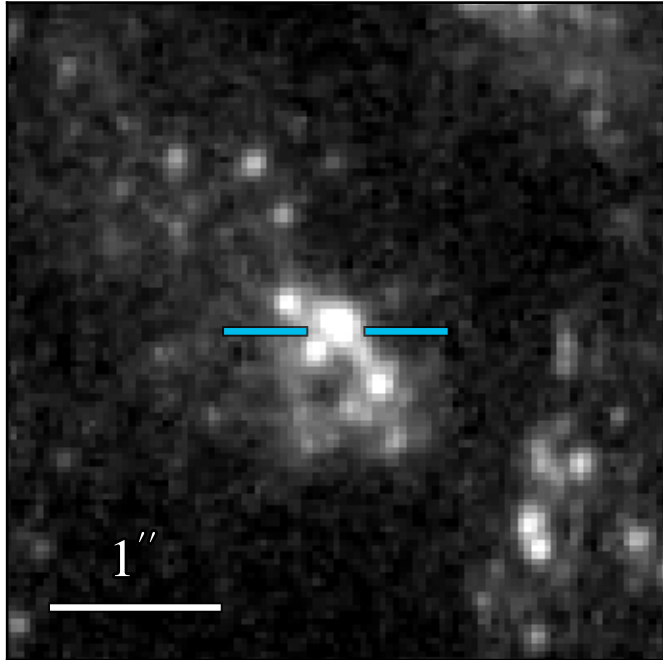
WFC3 F275W 20.514 ± 0.016
