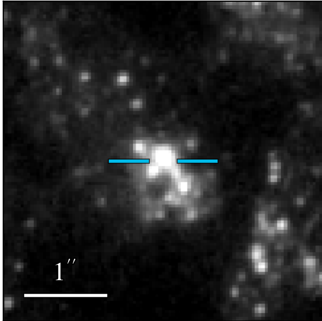
WFC3 F336W 19.790 ± 0.010
