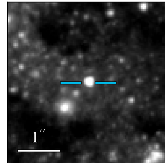
WFC3 F606W 20.439 \pm 0.002
