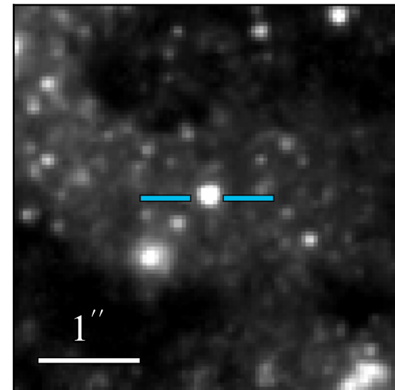
WFC3 F475W 21.035 \pm 0.003
