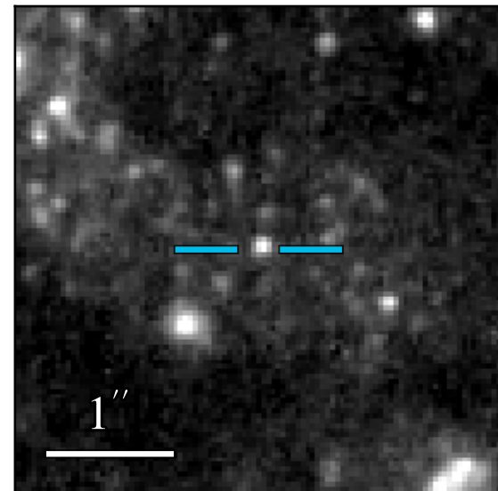
WFC3 F336W 22.507 \pm 0.027
