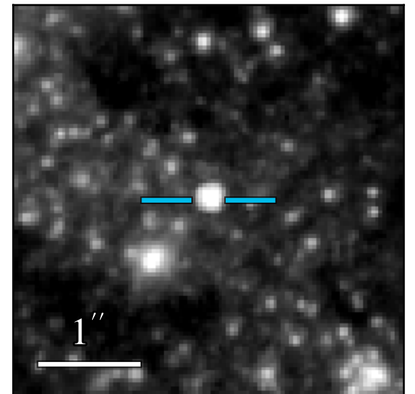
WFC3 F814W 19.846 \pm 0.004
