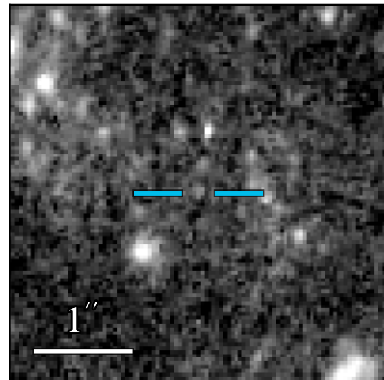
WFC3 F275W 25.049 \pm 0.287 (flagged)
