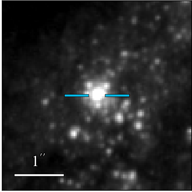
WFC3 F475W 21.507 ± 0.017
