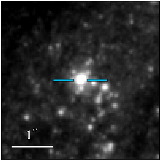
WFC3 F814W 20.321 ± 0.016
