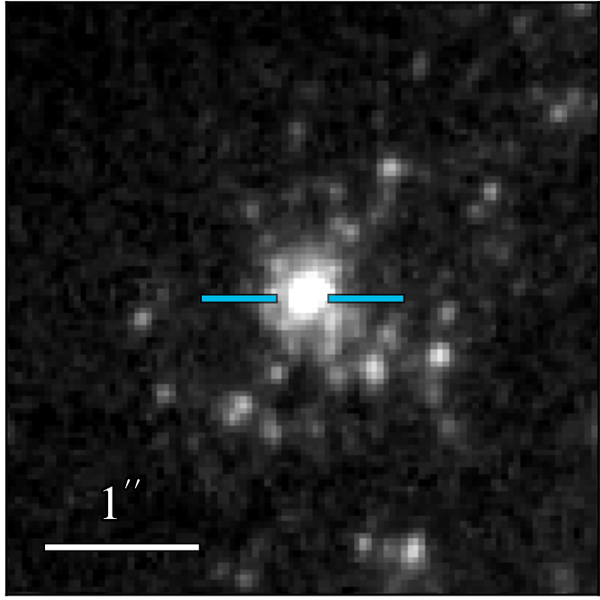
WFC3 F275W 20.512 ± 0.023
