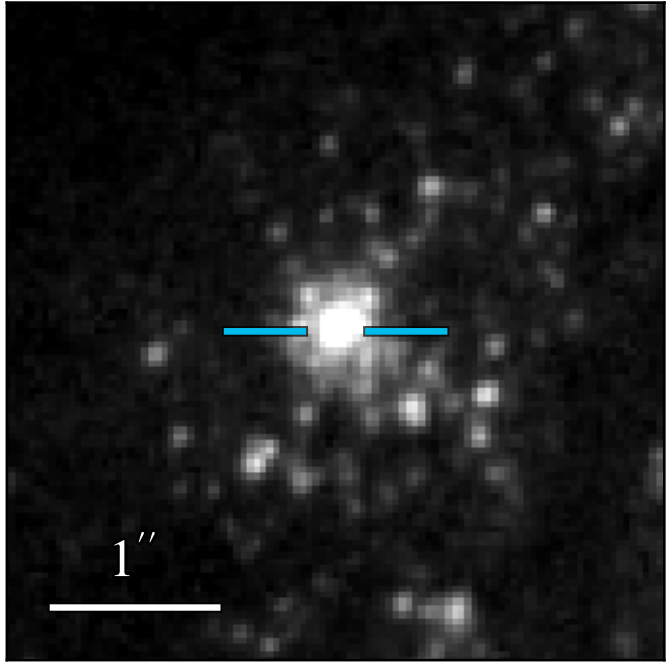
WFC3 F336W 20.566 ± 0.018
