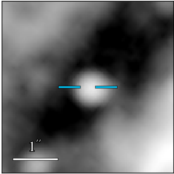
JWST/MIRI F1500W
