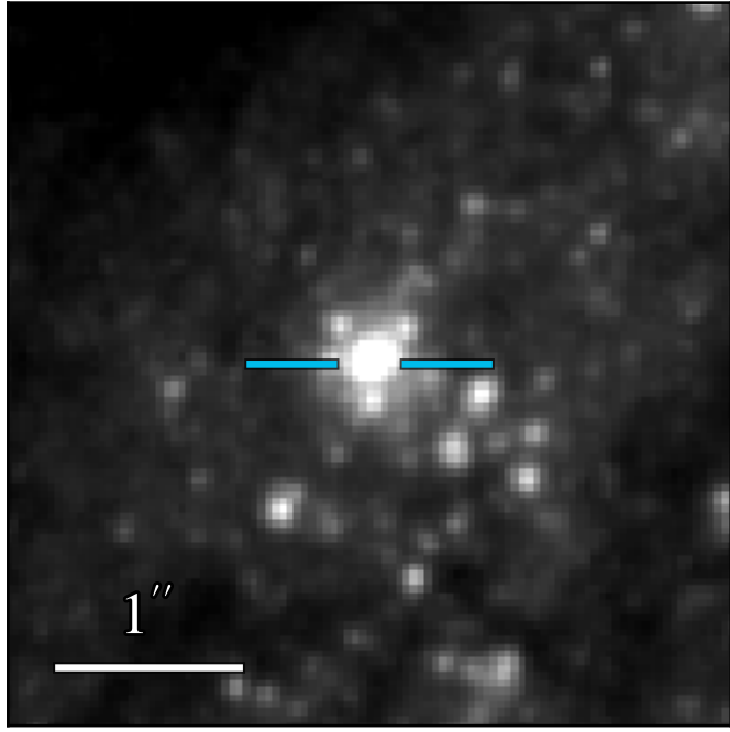
WFC3 F606W 21.191 ± 0.018
