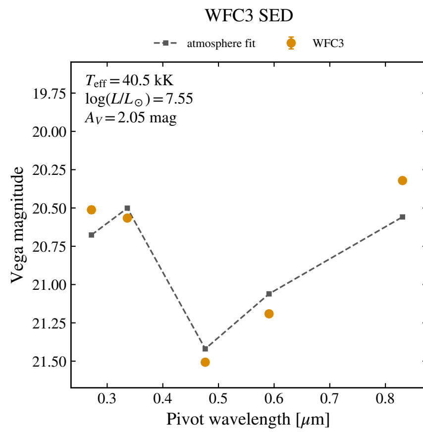
WFC3 F606W 21.191 ± 0.018
