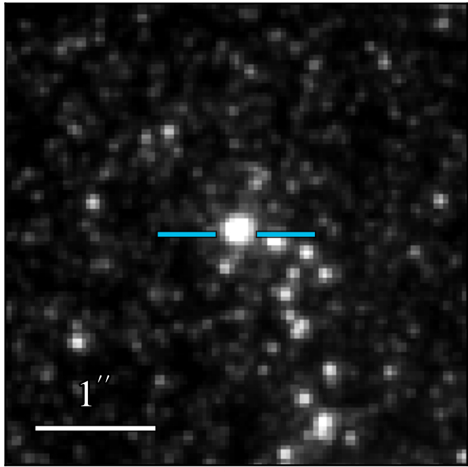
JWST/NIRCam F182M
