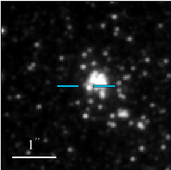
JWST/NIRCam F210M
