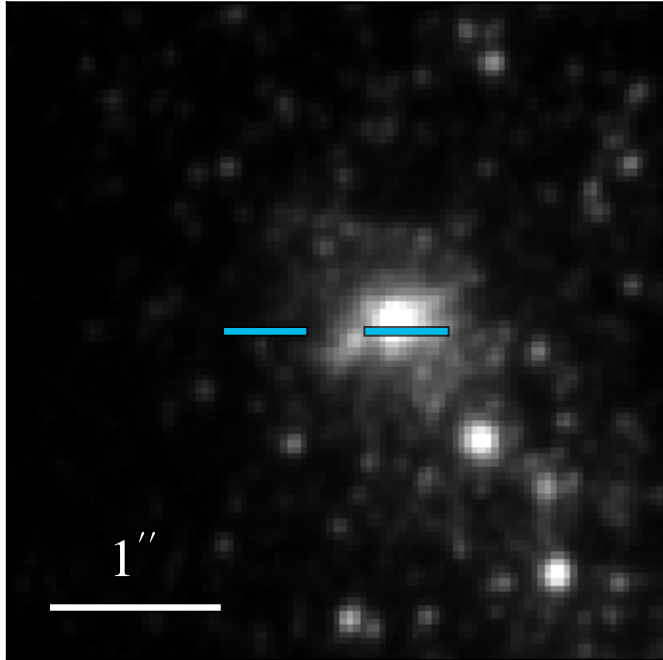
WFC3 F275W 21.662 ± 0.065 (flagged)
