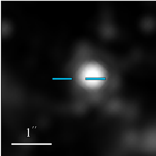
JWST/MIRI F1000W
