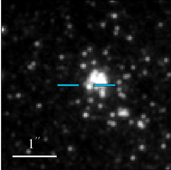
JWST/NIRCam F212N
