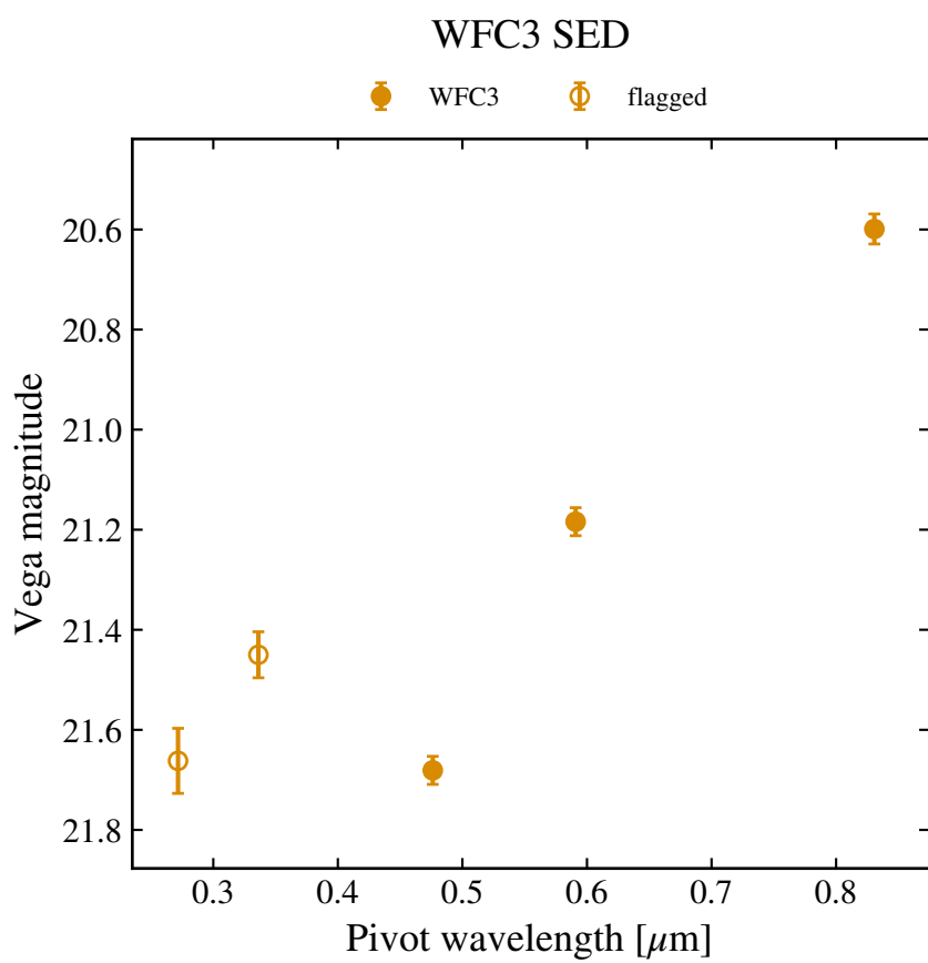
WFC3 F606W 21.184 ± 0.028
