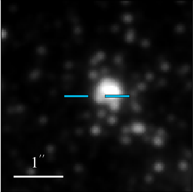
JWST/NIRCam F360M
