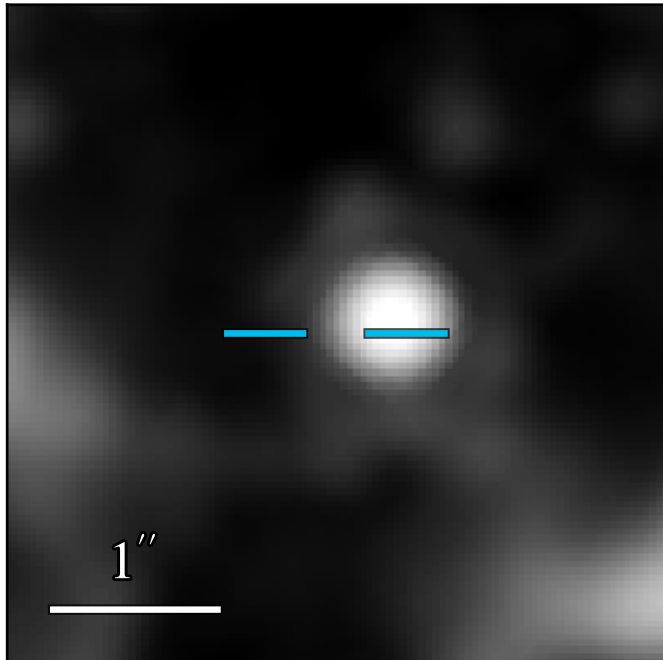
JWST/MIRI F1130W
