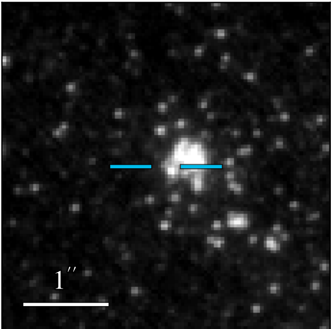
JWST/NIRCam F164N
