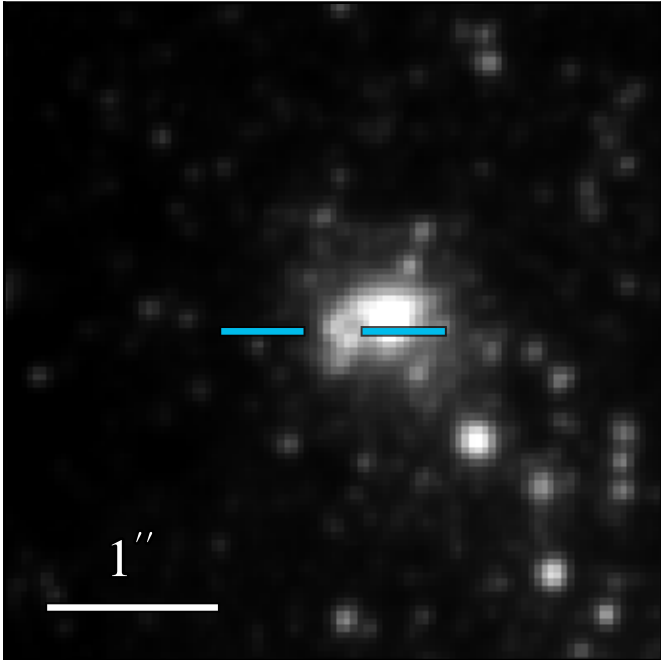
WFC3 F606W 21.184 ± 0.028
