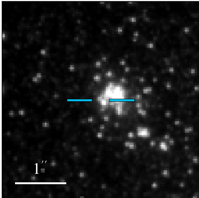
JWST/NIRCam F140M
