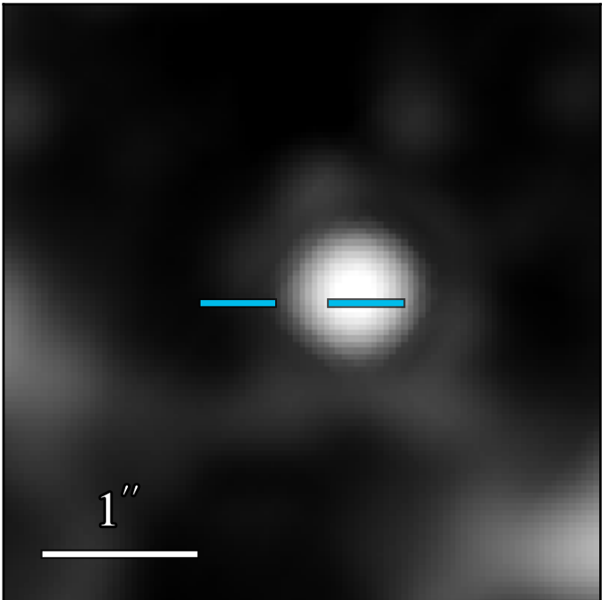
JWST/MIRI F1280W
