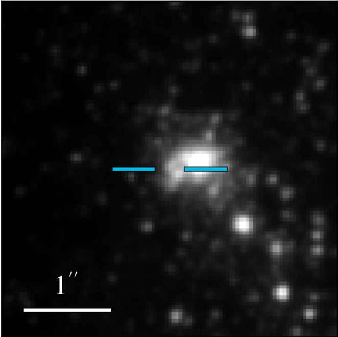
WFC3 F475W 21.681 ± 0.028
