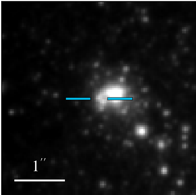
WFC3 F814W 20.599 ± 0.030
