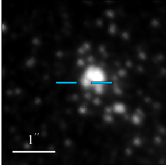
JWST/NIRCam F250M
