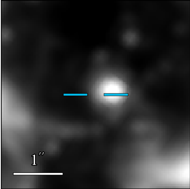
JWST/MIRI F770W
