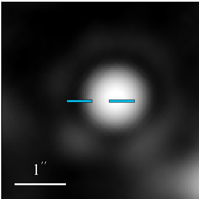
JWST/MIRI F2100W
