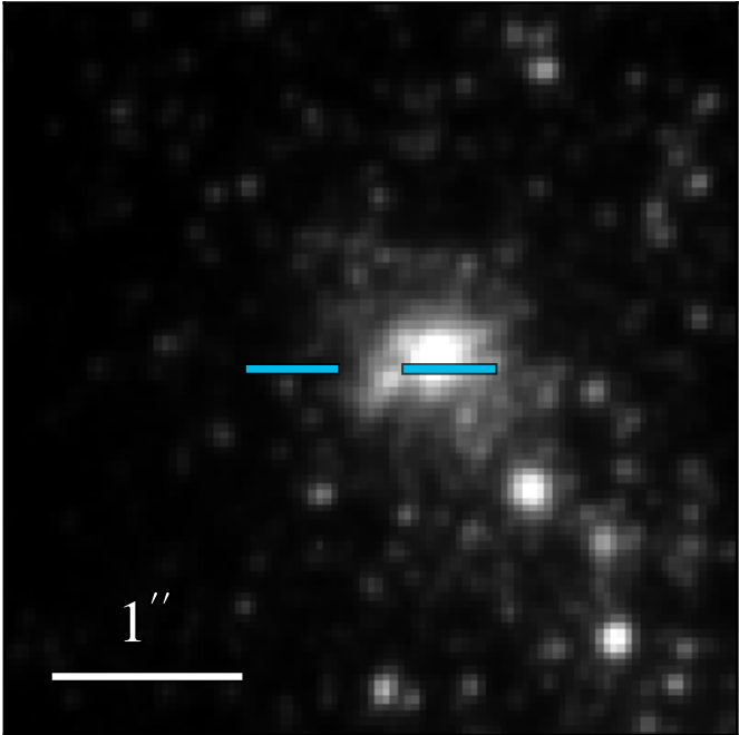
WFC3 F336W 21.450 ± 0.046 (flagged)
