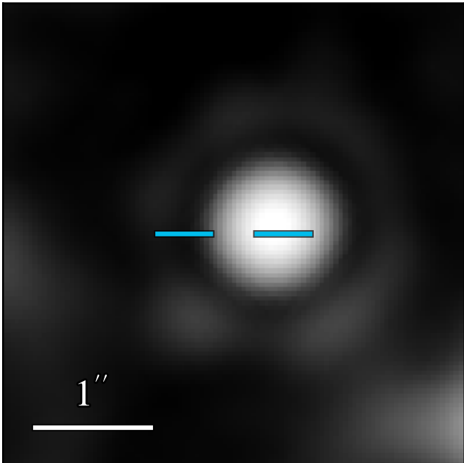
JWST/MIRI F1800W
