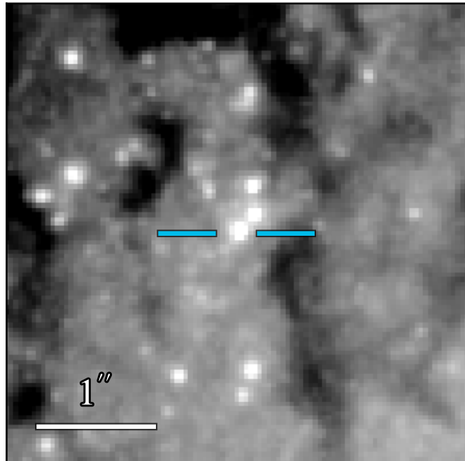
WFC3 F814W 20.744 ± 0.008
