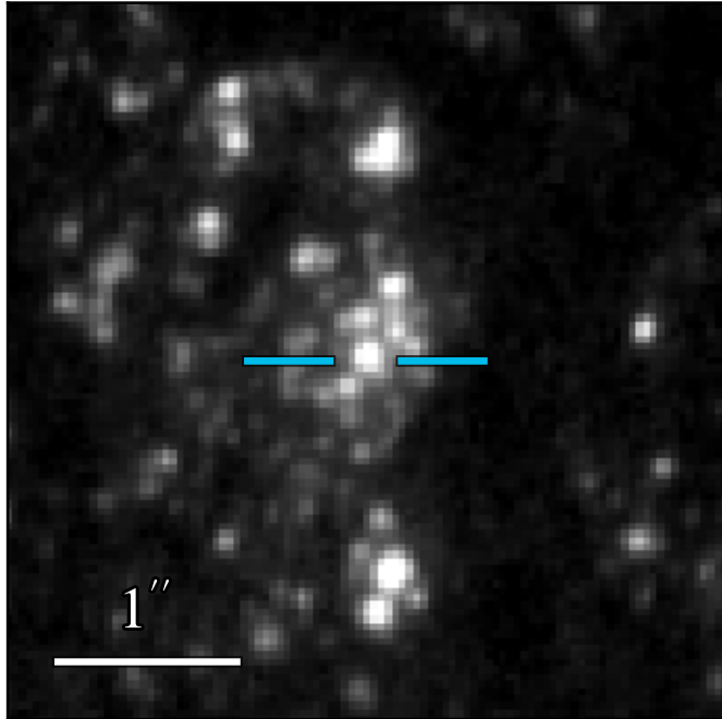
WFC3 F275W 20.311 ± 0.012
