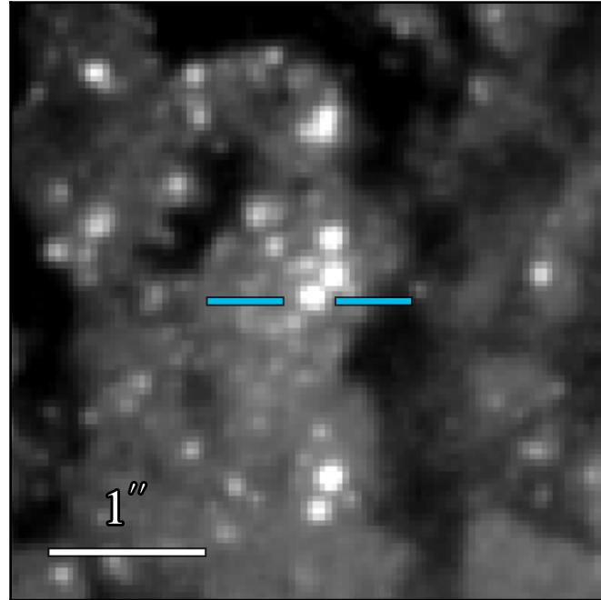
WFC3 F475W 21.371 ± 0.006
