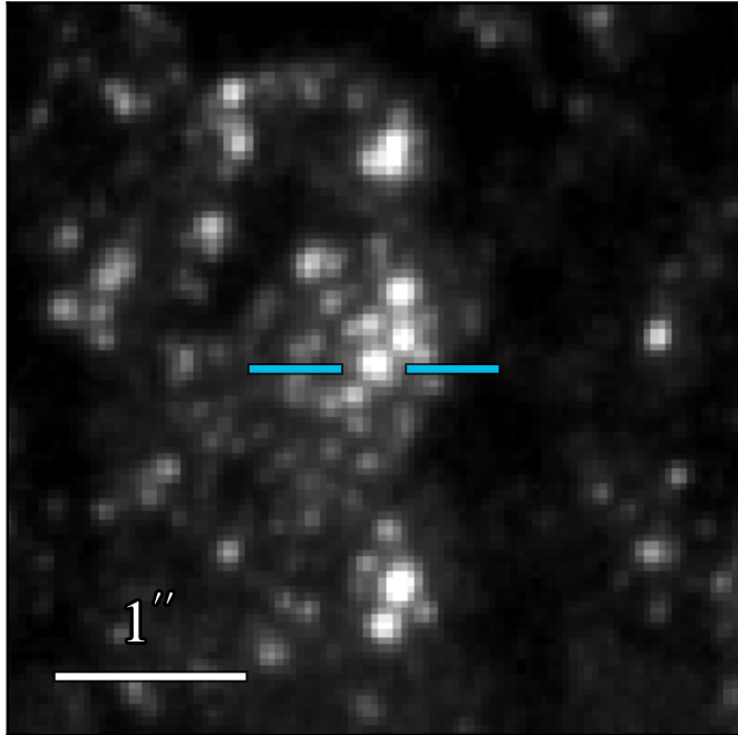
WFC3 F336W 20.545 ± 0.009
