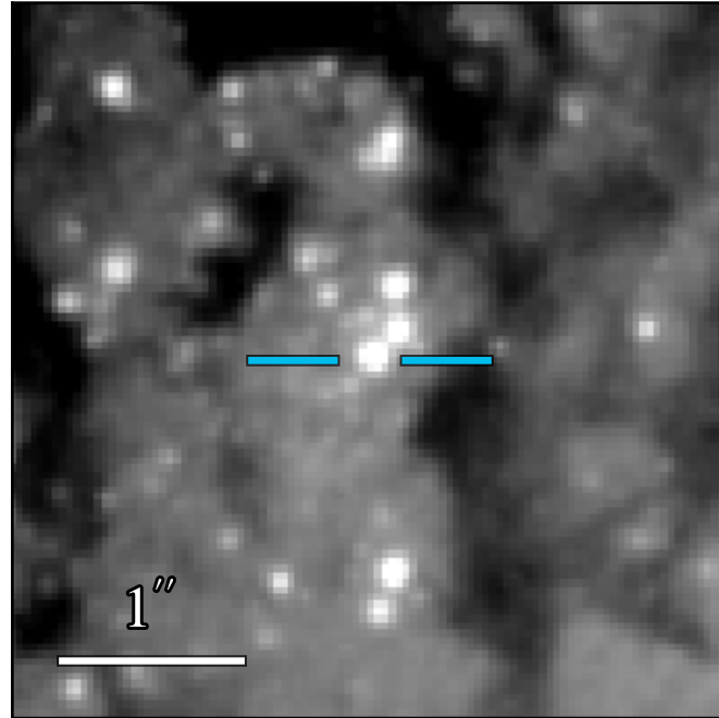
WFC3 F606W 21.084 ± 0.005
