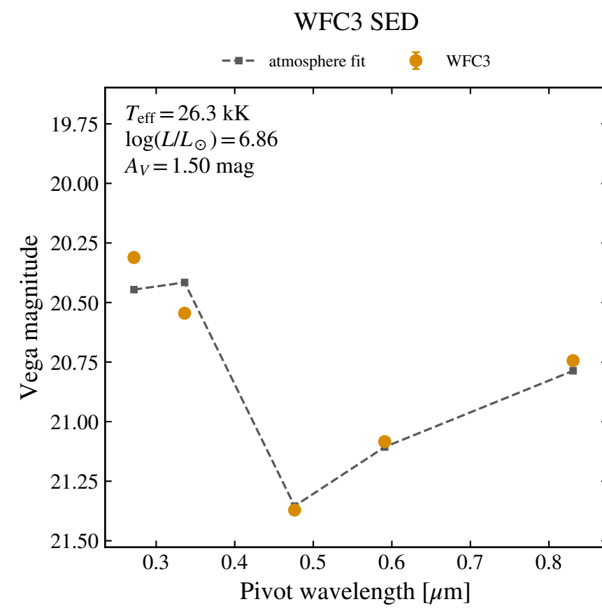
WFC3 F606W 21.084 ± 0.005
