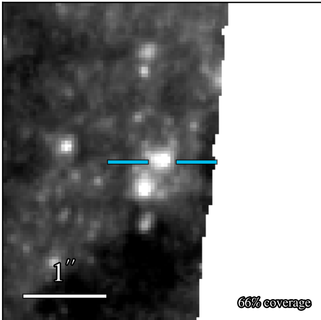
WFC3 F814W 20.619 ± 0.009
