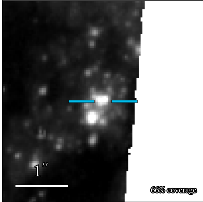
WFC3 F475W 21.228 ± 0.007
