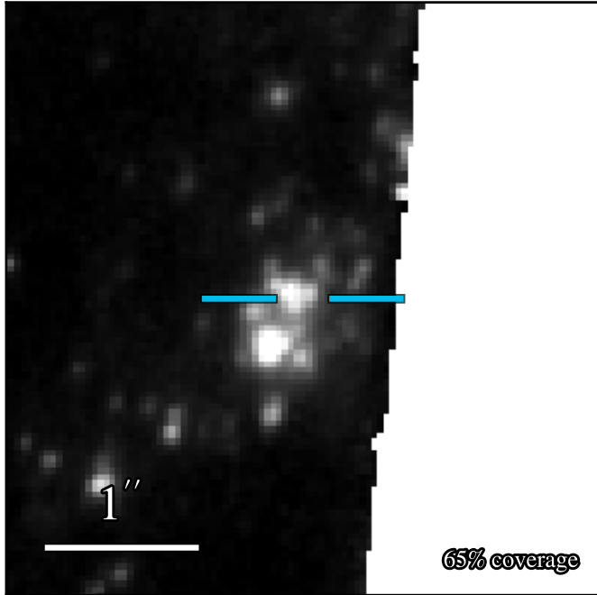
WFC3 F336W 21.456 ± 0.023
