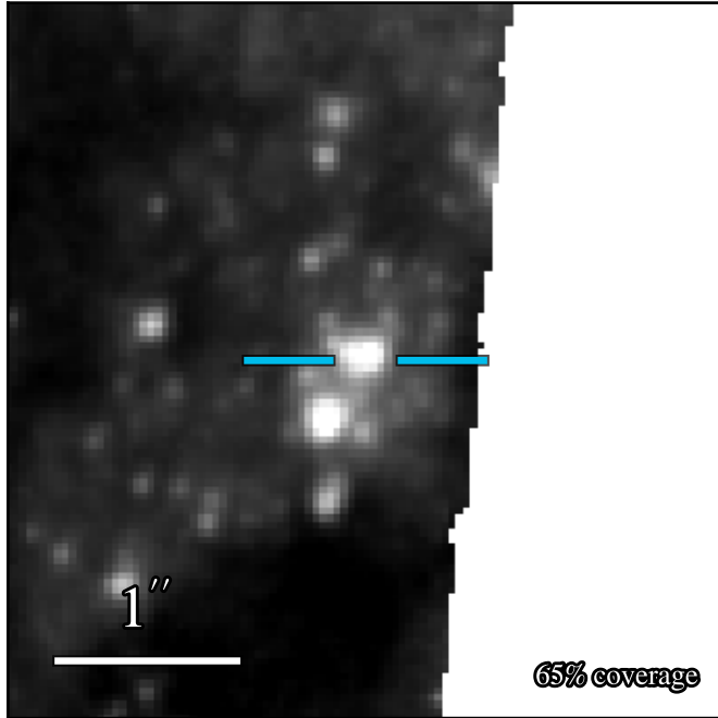
WFC3 F606W 20.962 ± 0.007
