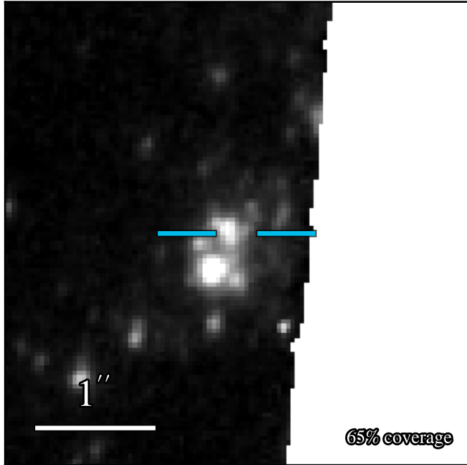
WFC3 F275W 22.412 ± 0.067 (flagged)
