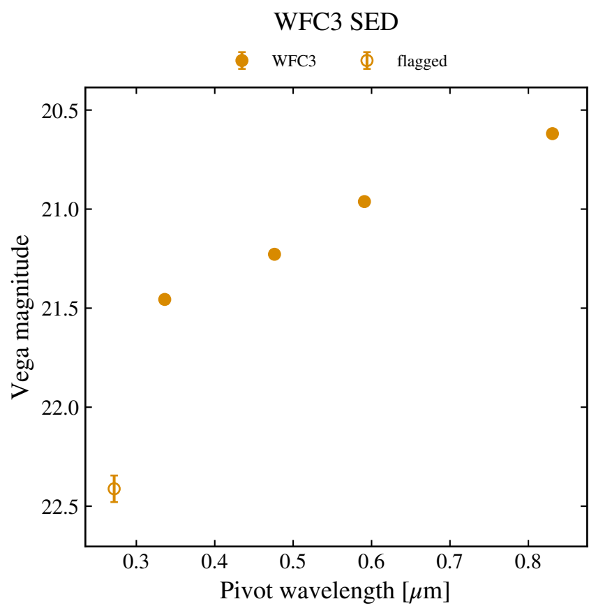
WFC3 F606W 20.962 ± 0.007
