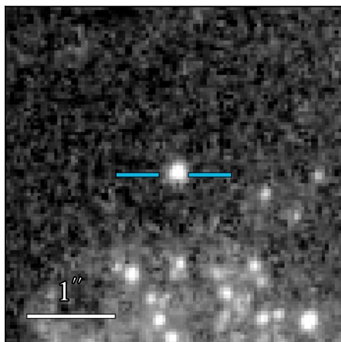
WFC3 F275W 22.164 ± 0.032
