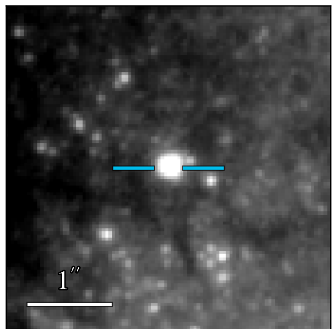
WFC3 F814W 19.622 ± 0.004
