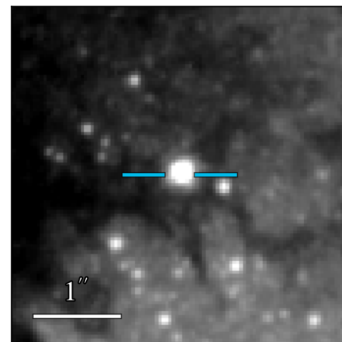
WFC3 F606W 20.491 ± 0.004
