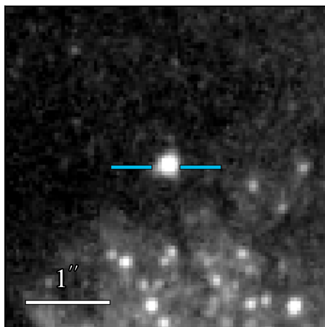
WFC3 F336W 21.219 ± 0.011
