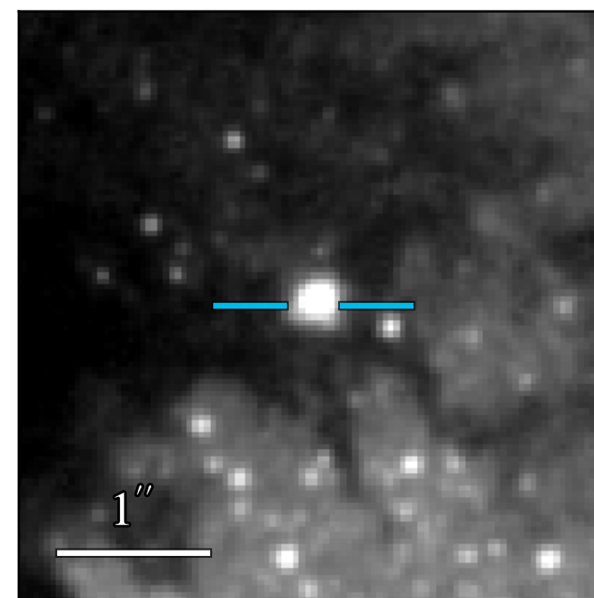
WFC3 F475W 21.122 ± 0.004
