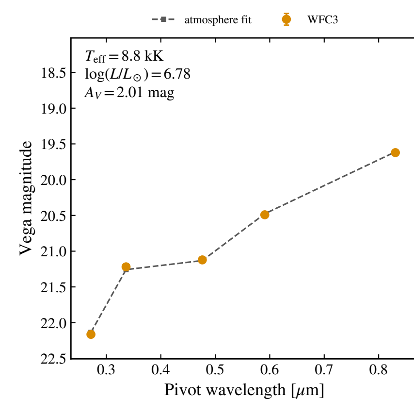
WFC3 SED
