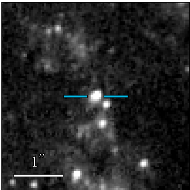
WFC3 F336W 21.950 \pm 0.019
