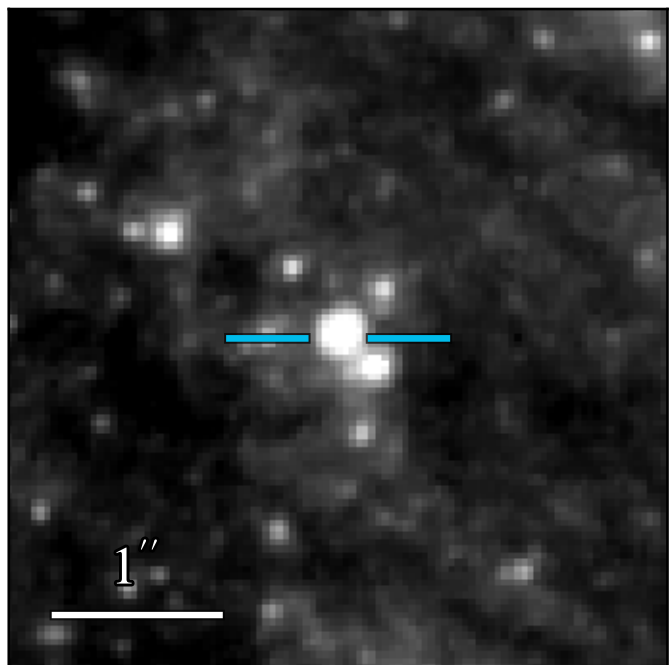
WFC3 F814W 19.408 \pm 0.004
