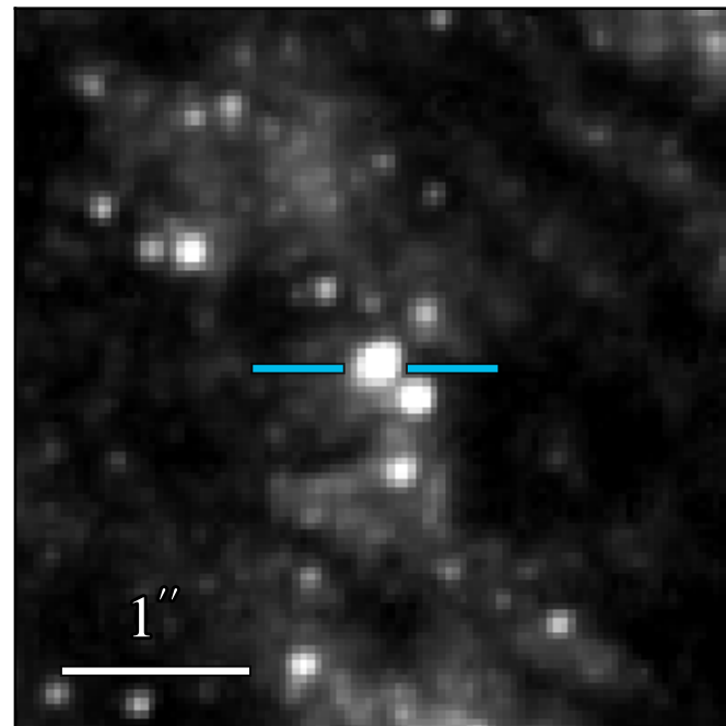
WFC3 F475W 21.311 \pm 0.006
