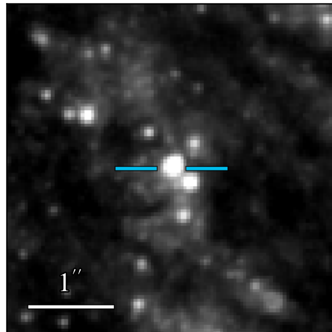
WFC3 F606W 20.406 \pm 0.004
