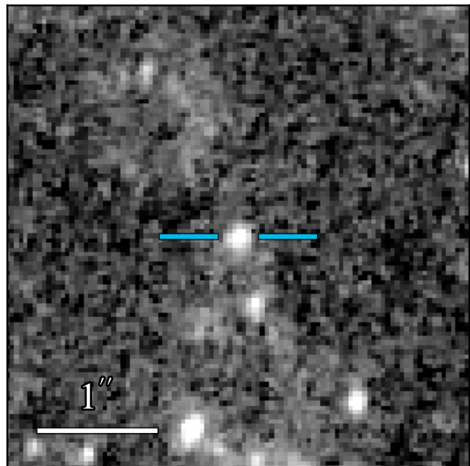
WFC3 F275W 23.852 \pm 0.114
