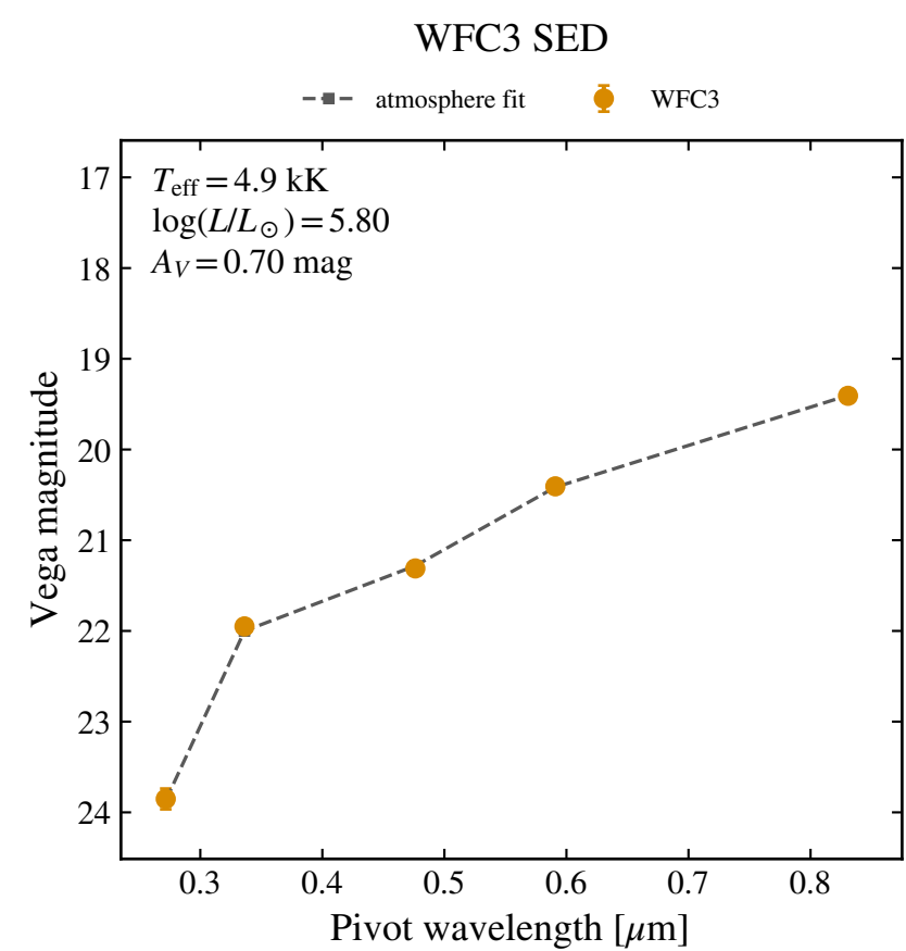
WFC3 F606W 20.406 \pm 0.004
