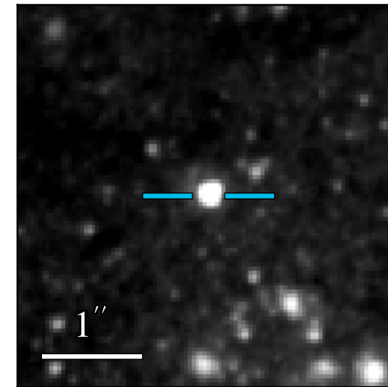
WFC3 F606W 20.408 \pm 0.002
