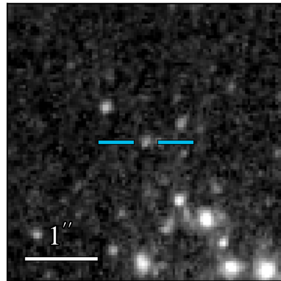
WFC3 F275W 24.115 \pm 0.107
