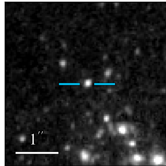
WFC3 F336W 22.409 \pm 0.021
