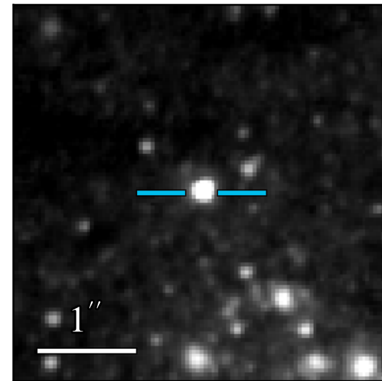
WFC3 F475W 21.009 \pm 0.003
