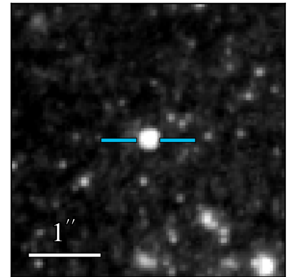
WFC3 F814W 19.843 \pm 0.003
