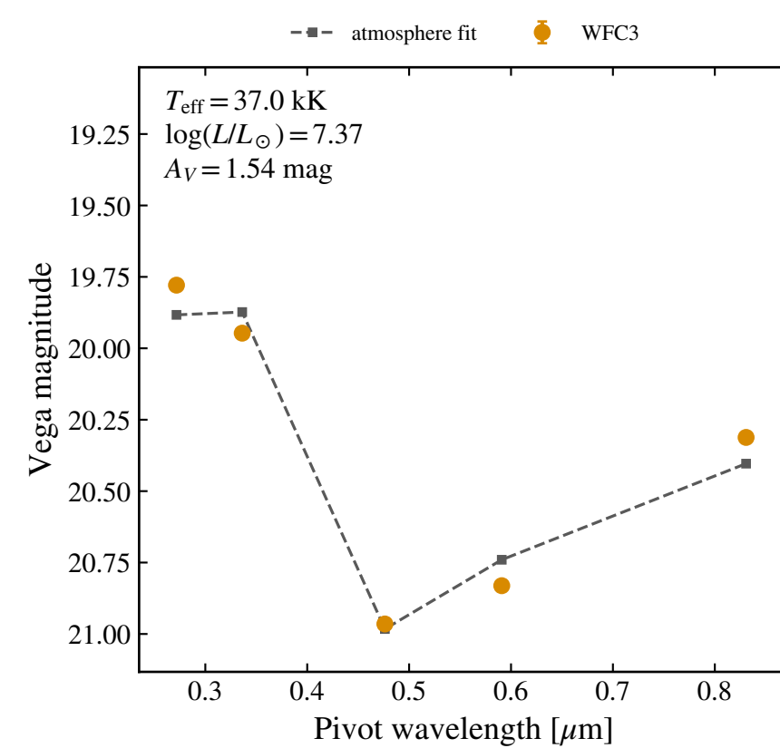
WFC3 SED
