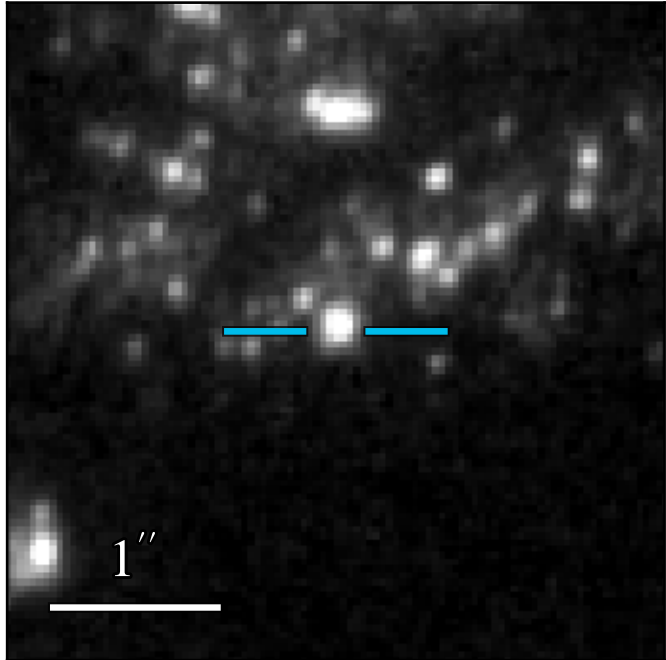
WFC3 F275W 20.346 ± 0.015
