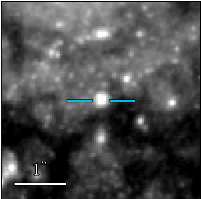
WFC3 F814W 20.225 ± 0.008
