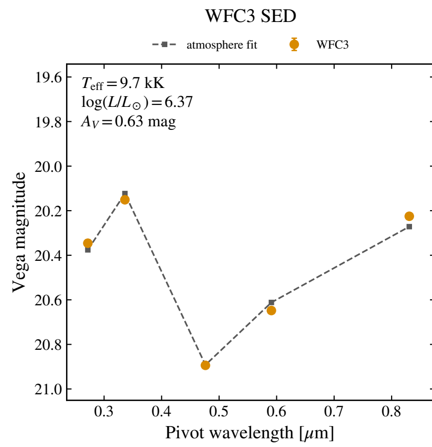
WFC3 F606W 20.648 ± 0.007
