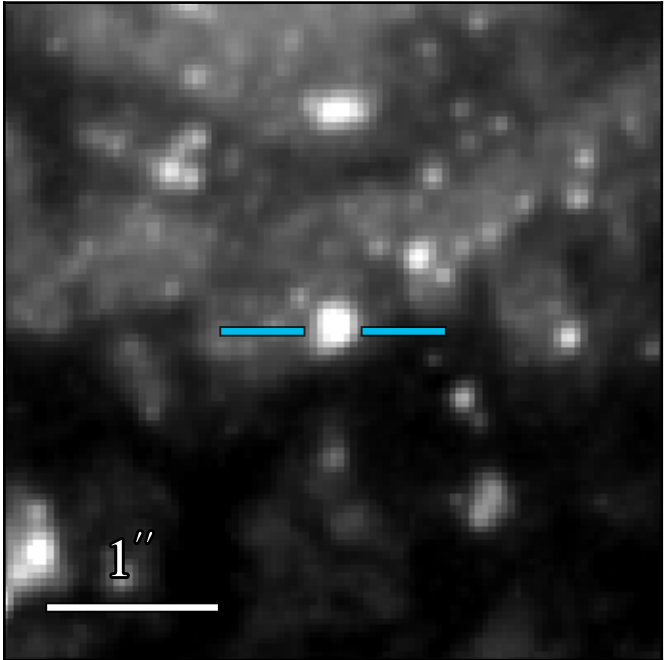
WFC3 F606W 20.648 ± 0.007
