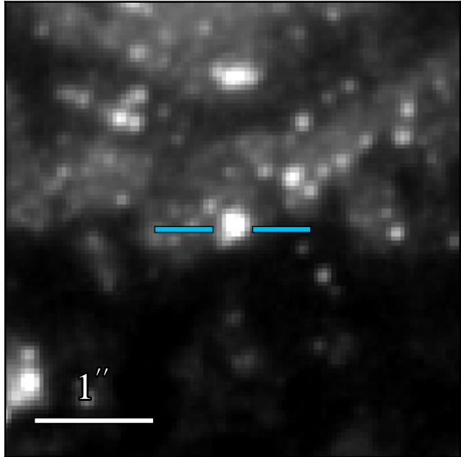
WFC3 F475W 20.894 ± 0.007
