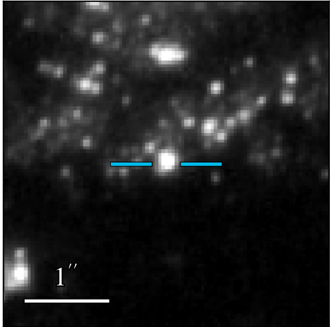
WFC3 F336W 20.151 ± 0.010
