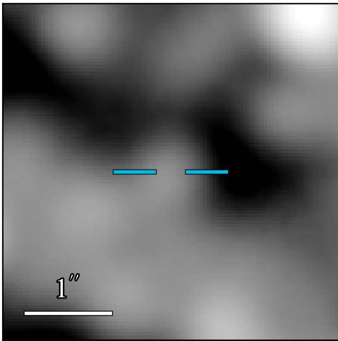
JWST/MIRI F2100W
