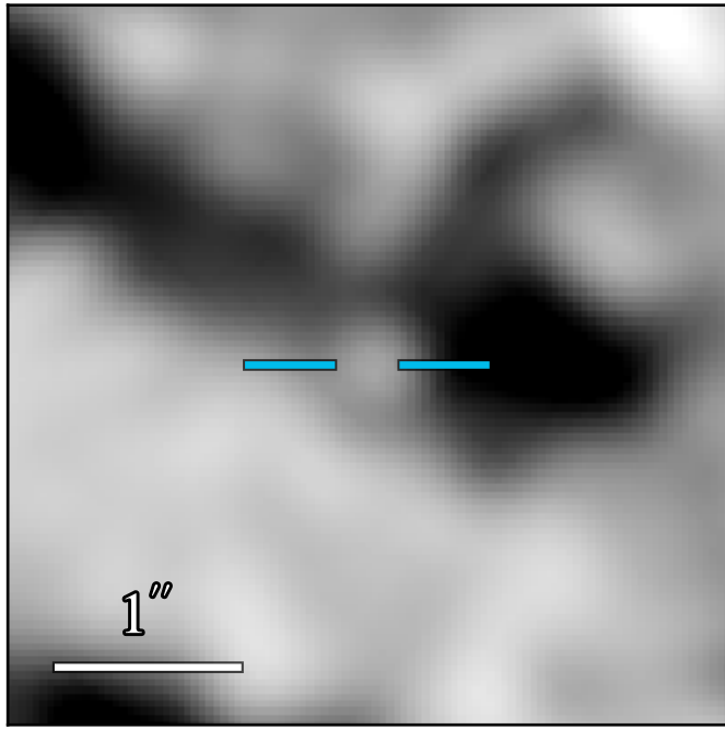
JWST/MIRI F1130W
