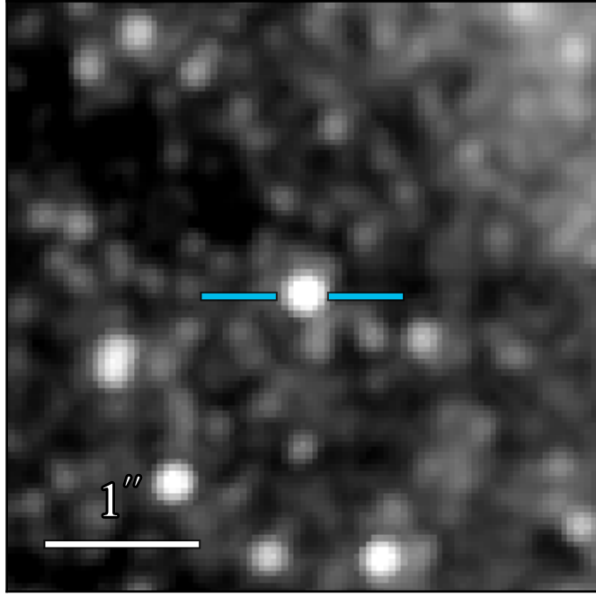
JWST/NIRCam F430M
