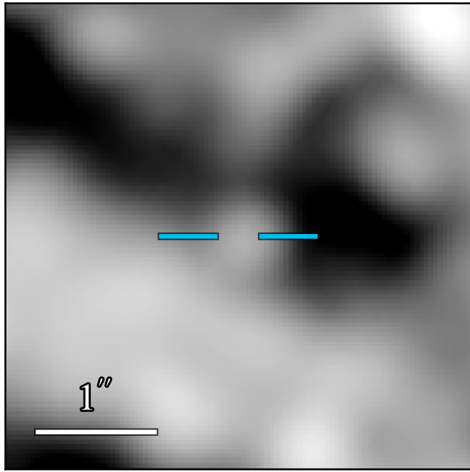
JWST/MIRI F1500W
