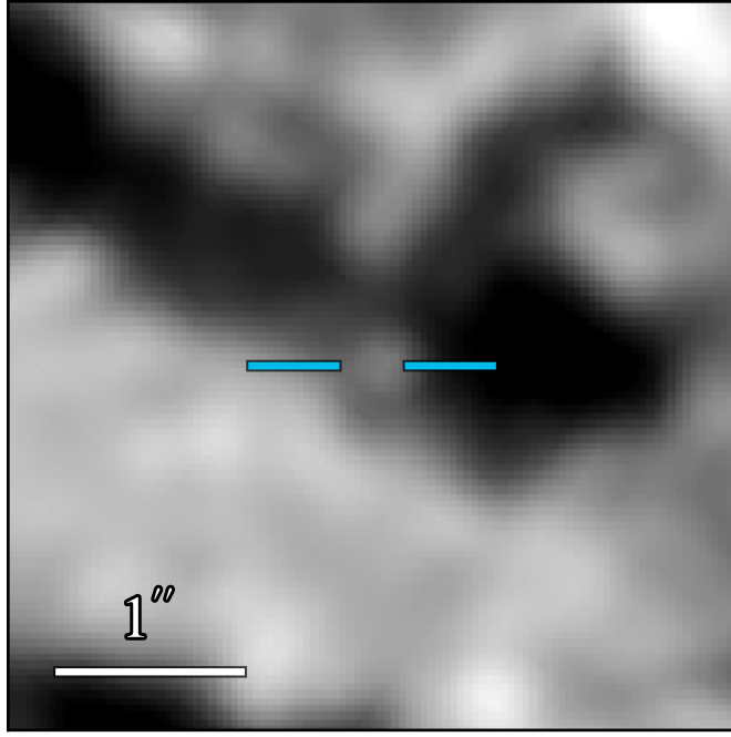
JWST/MIRI F770W
