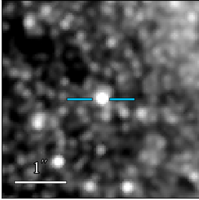
JWST/NIRCam F360M
