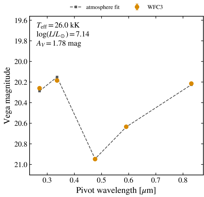
WFC3 SED
