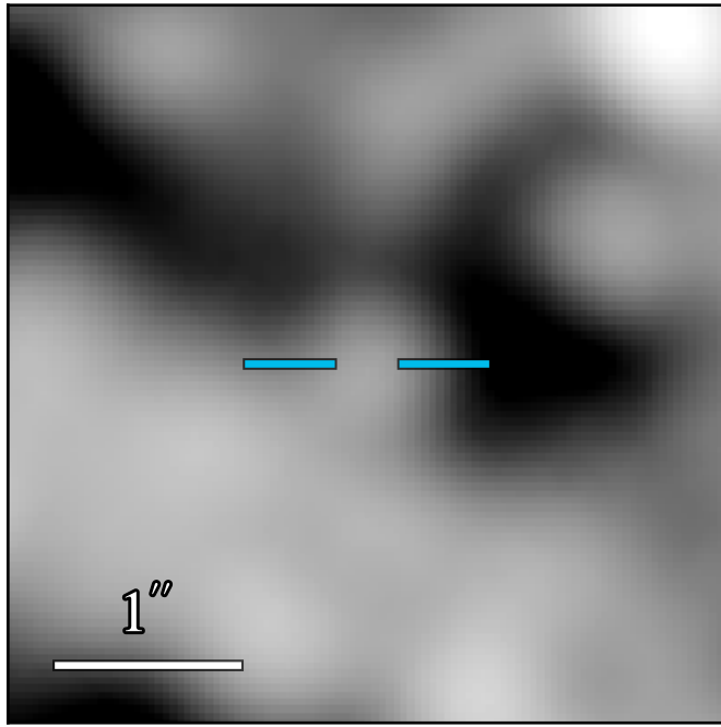
JWST/MIRI F1800W
