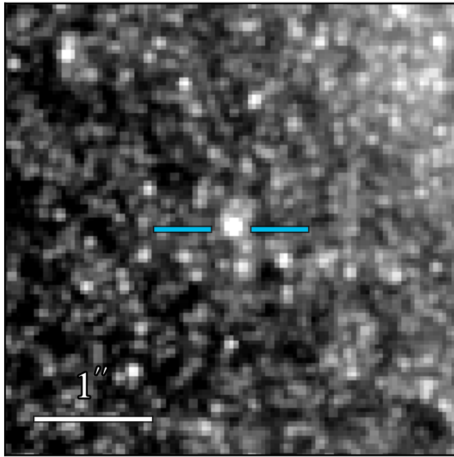
JWST/NIRCam F210M
