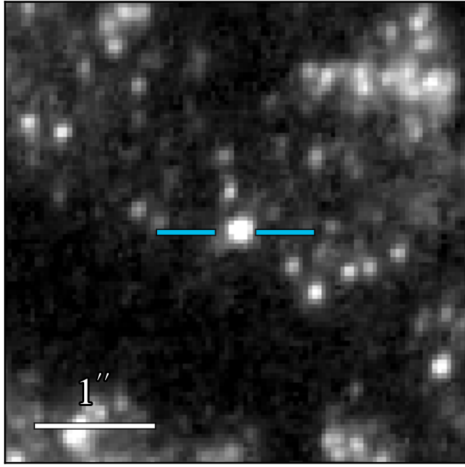
WFC3 F275W 20.260 ± 0.011
