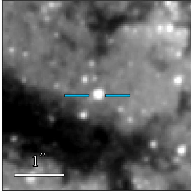
WFC3 F606W 20.634 ± 0.003
