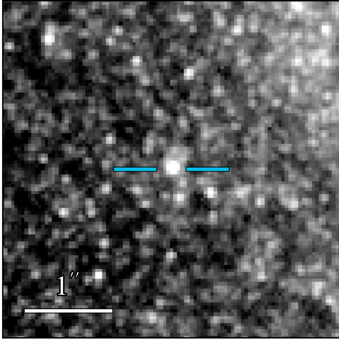
JWST/NIRCam F212N
