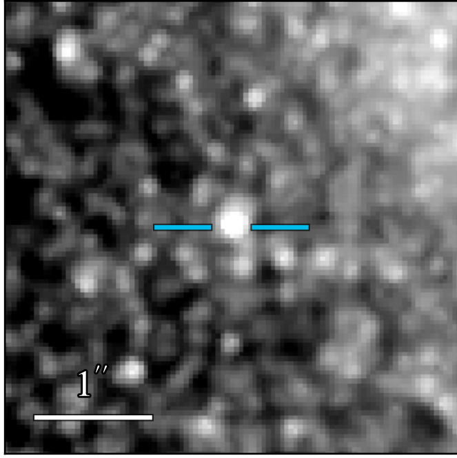
JWST/NIRCam F250M
