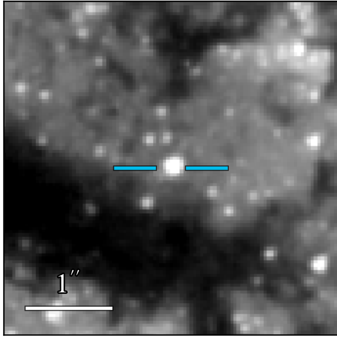
WFC3 F475W 20.948 ± 0.004
