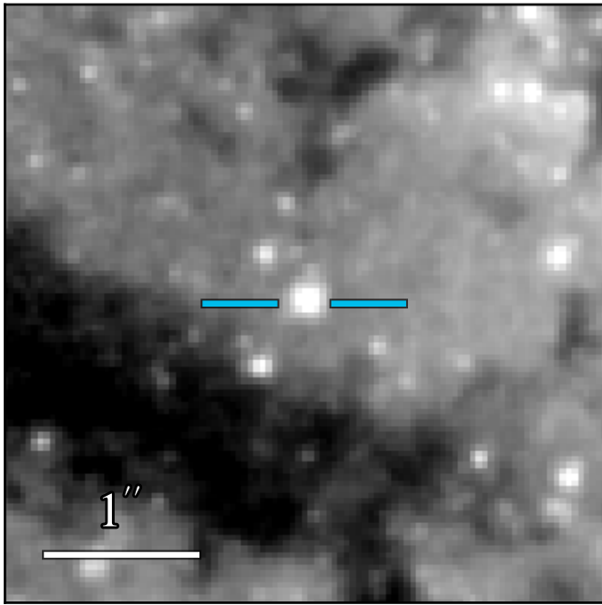
WFC3 F814W 20.215 ± 0.005
