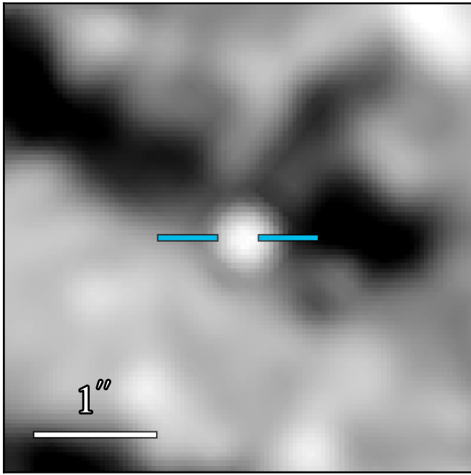
JWST/MIRI F1000W
