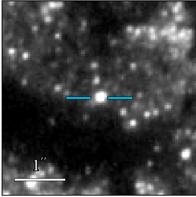
WFC3 F336W 20.185 ± 0.007
