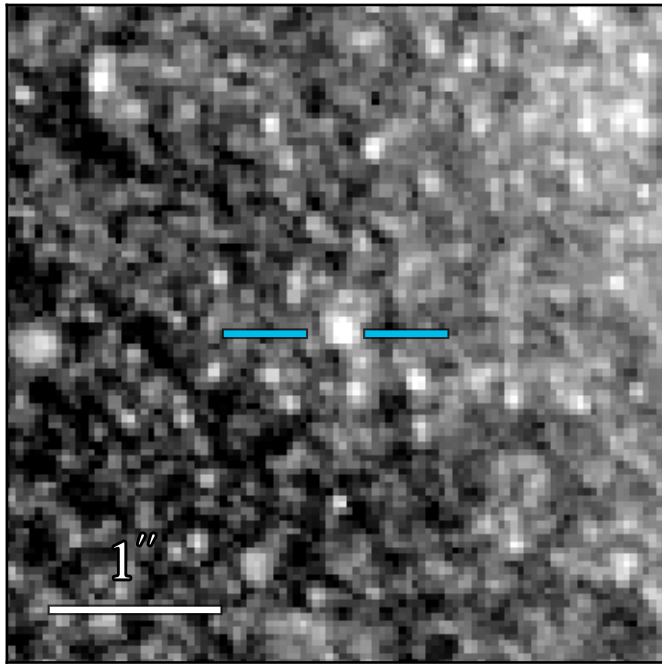
JWST/NIRCam F164N
