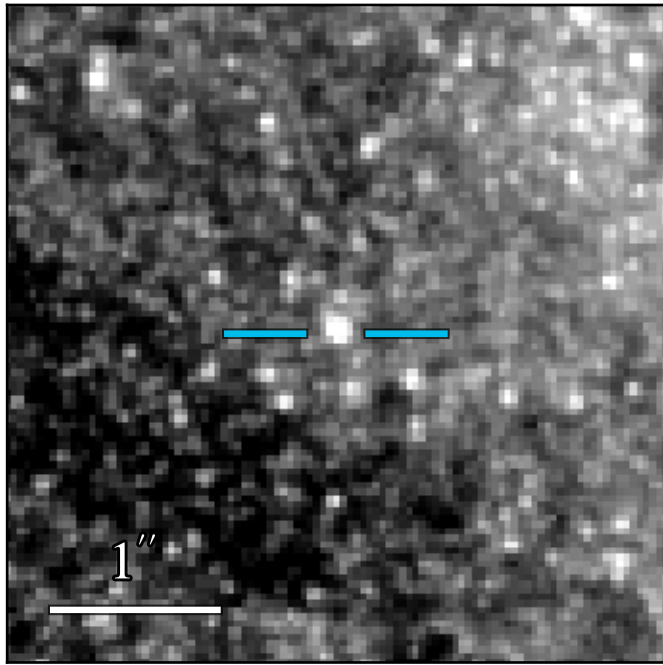
JWST/NIRCam F140M
