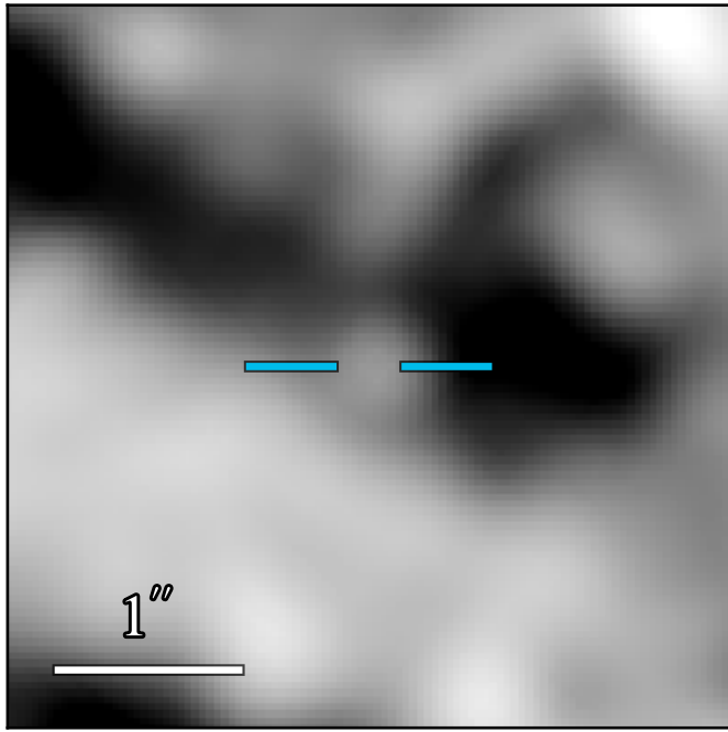
JWST/MIRI F1280W
