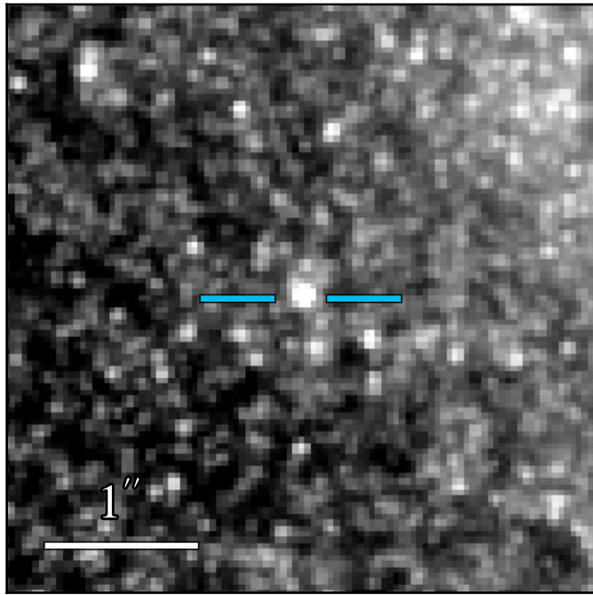
JWST/NIRCam F182M
