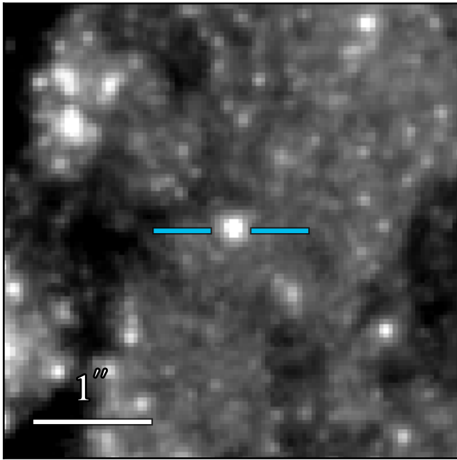
WFC3 F814W 20.928 ± 0.006
