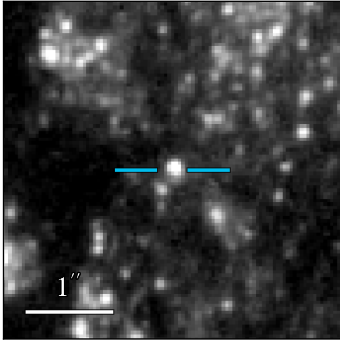
WFC3 F336W 21.502 ± 0.014
