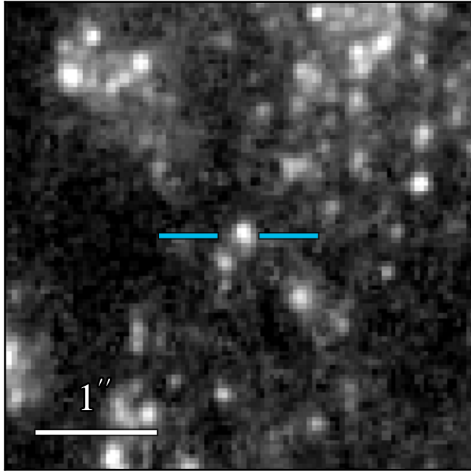
WFC3 F275W 22.375 ± 0.036
