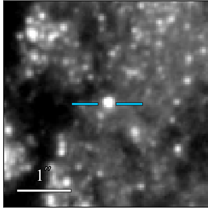
WFC3 F475W 21.580 ± 0.005
