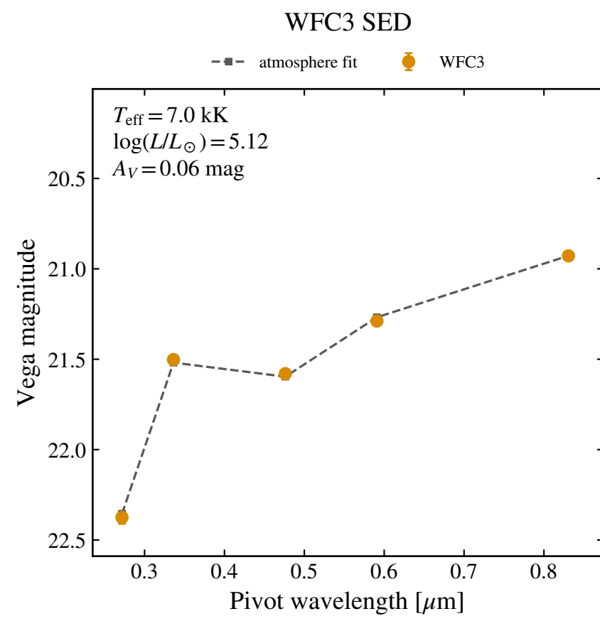
WFC3 F606W 21.289 ± 0.004
