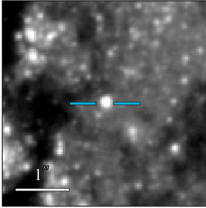
WFC3 F606W 21.289 ± 0.004
