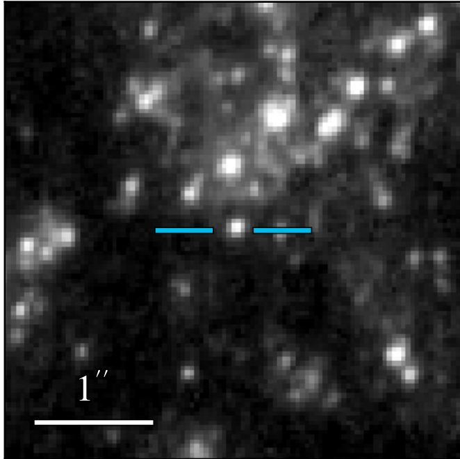
WFC3 F336W 22.349 ± 0.021
