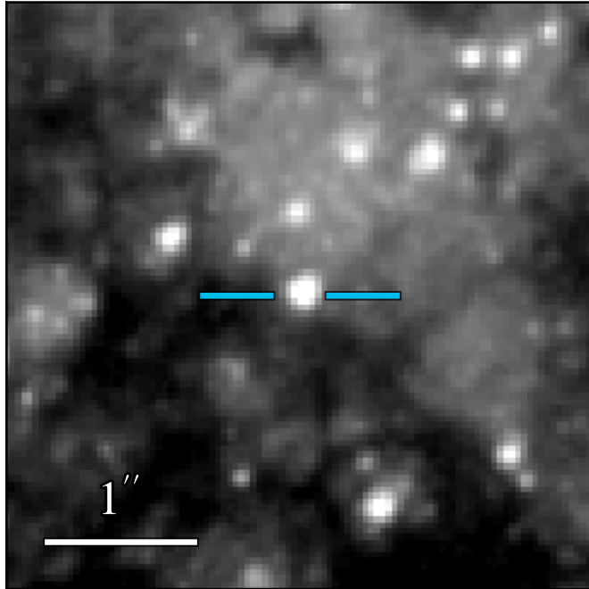
WFC3 F606W 21.183 ± 0.004
