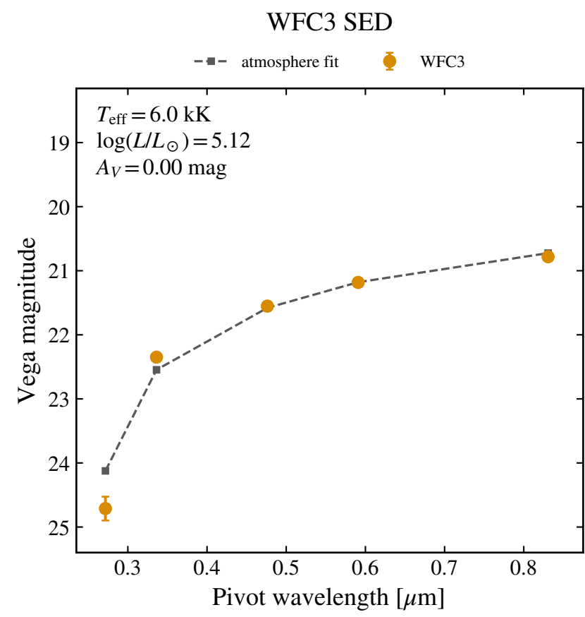
WFC3 F606W 21.183 ± 0.004
