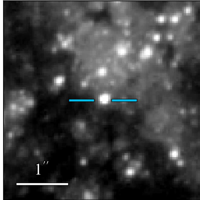
WFC3 F475W 21.552 ± 0.005
