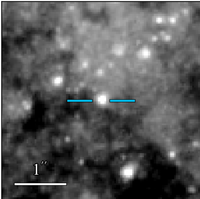
WFC3 F814W 20.782 ± 0.006
