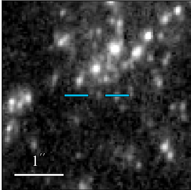
WFC3 F275W 24.712 ± 0.186
