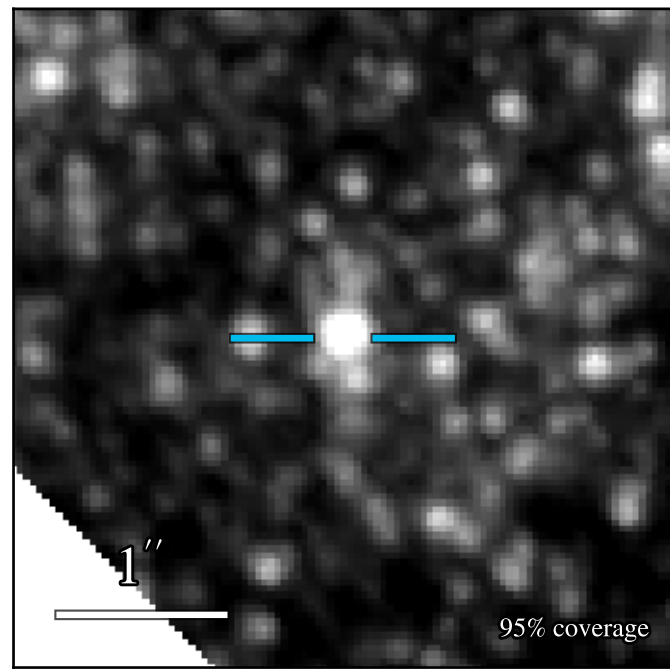
JWST/NIRCam F250M
