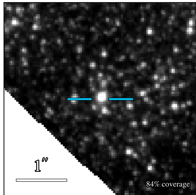
JWST/NIRCam F140M
