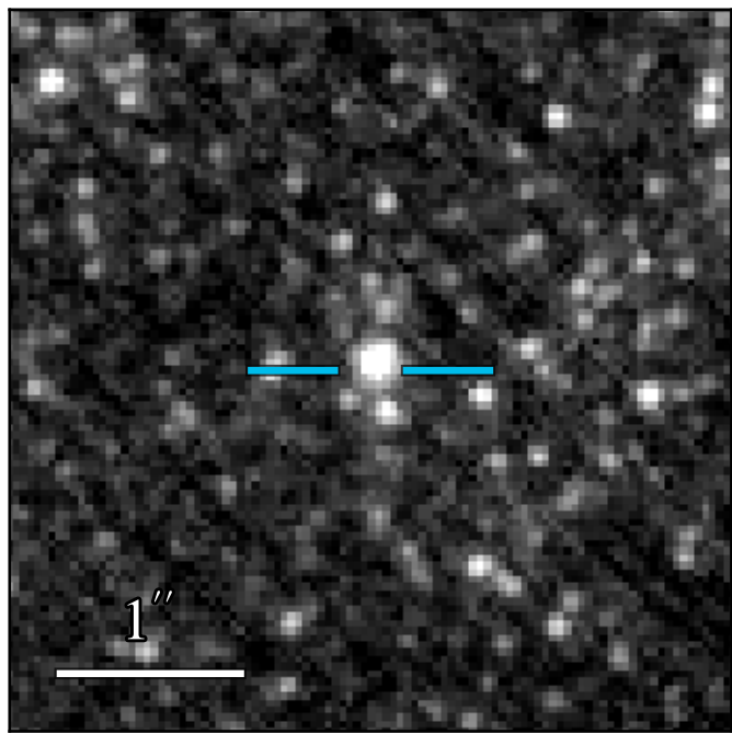
JWST/NIRCam F212N
