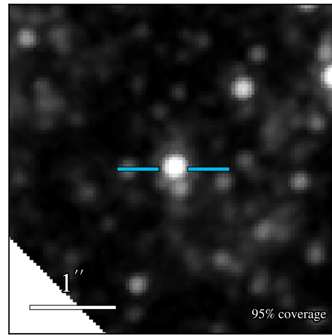
JWST/NIRCam F430M
