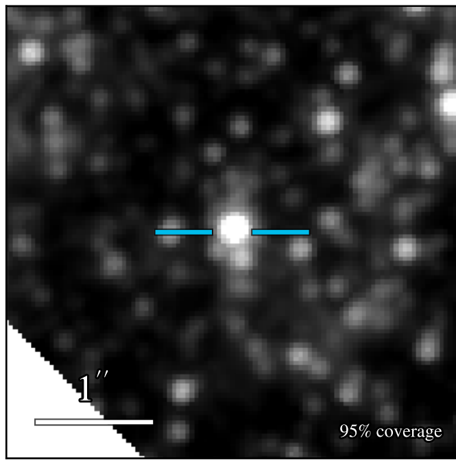
JWST/NIRCam F360M
