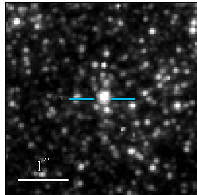
JWST/NIRCam F210M
