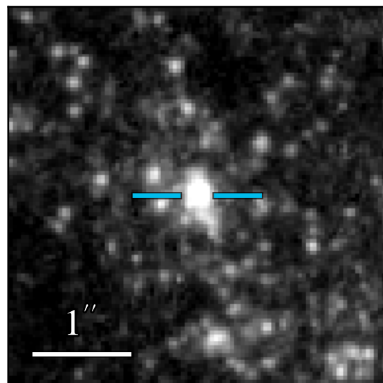
WFC3 F336W 20.908 \pm 0.016
