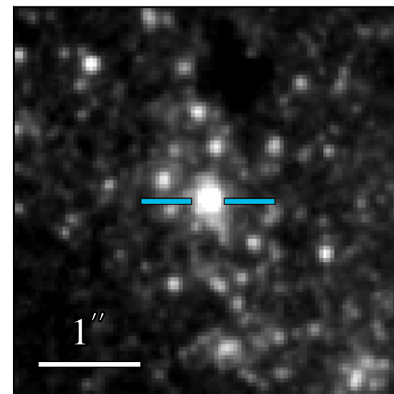
WFC3 F475W 21.561 \pm 0.010
