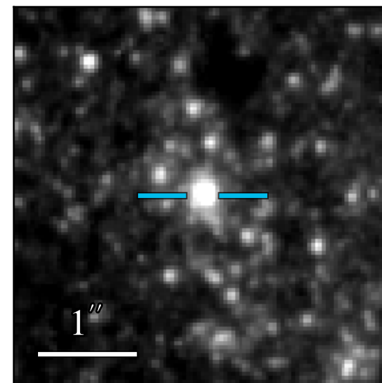
WFC3 F606W 21.361 \pm 0.009
