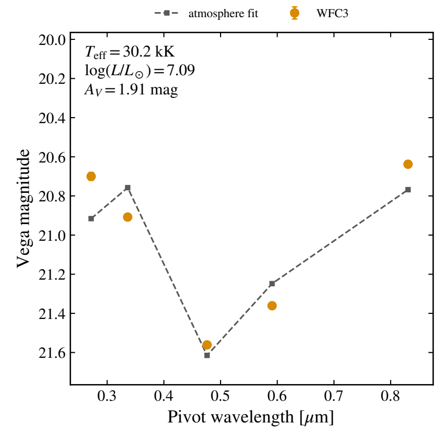
WFC3 SED
