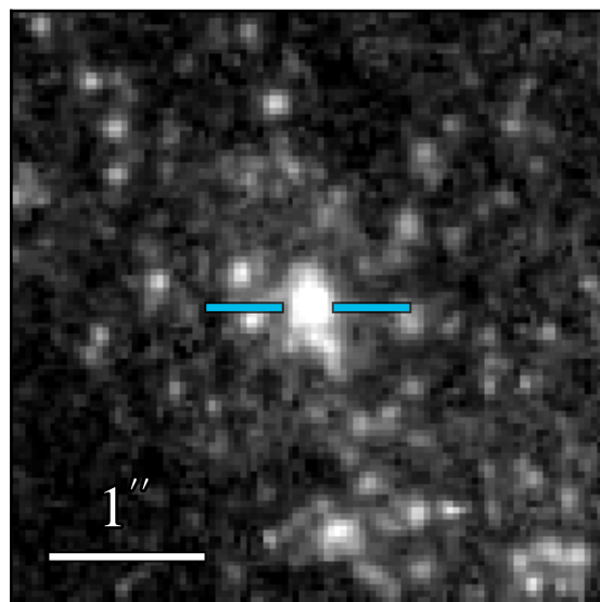
WFC3 F275W 20.700 \pm 0.020
