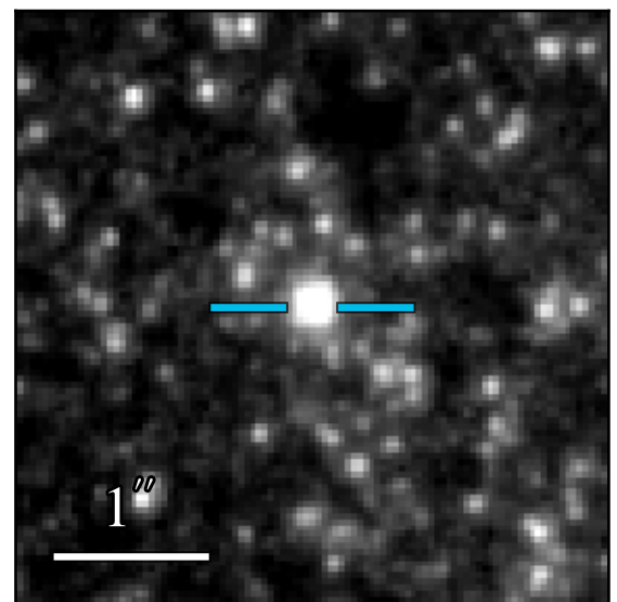
WFC3 F814W 20.638 \pm 0.009
