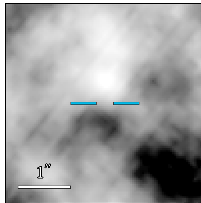
JWST/MIRI F1800W
