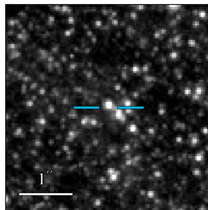
JWST/NIRCam F182M
