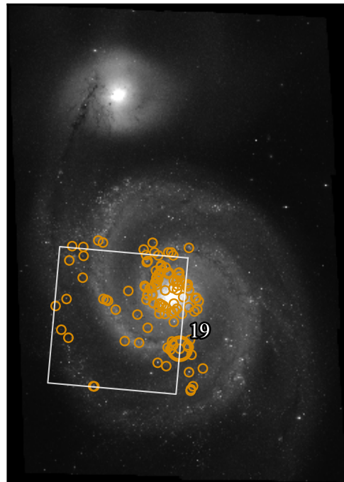
M51 / WFC3 footprint
