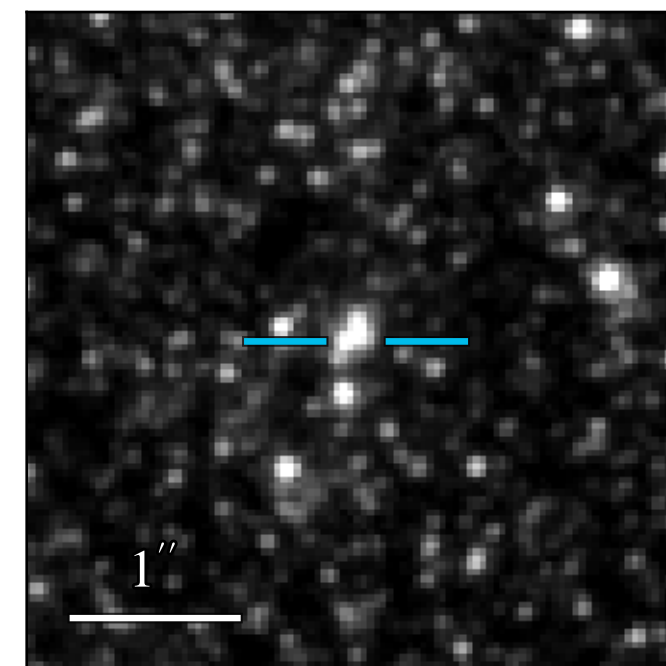
JWST/NIRCam F210M
