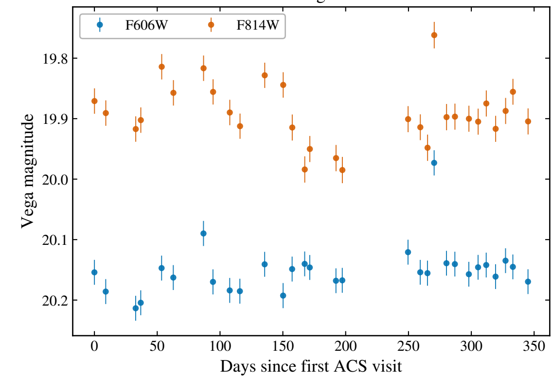
ACS visit light curves
