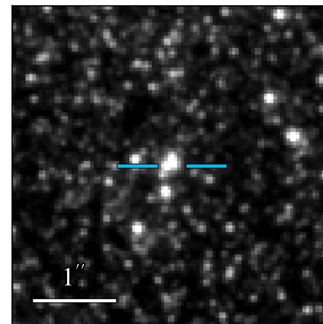
JWST/NIRCam F182M
