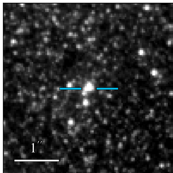
JWST/NIRCam F140M
