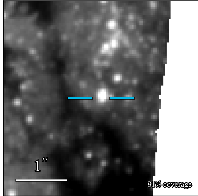
WFC3 F475W 21.018 ± 0.008
