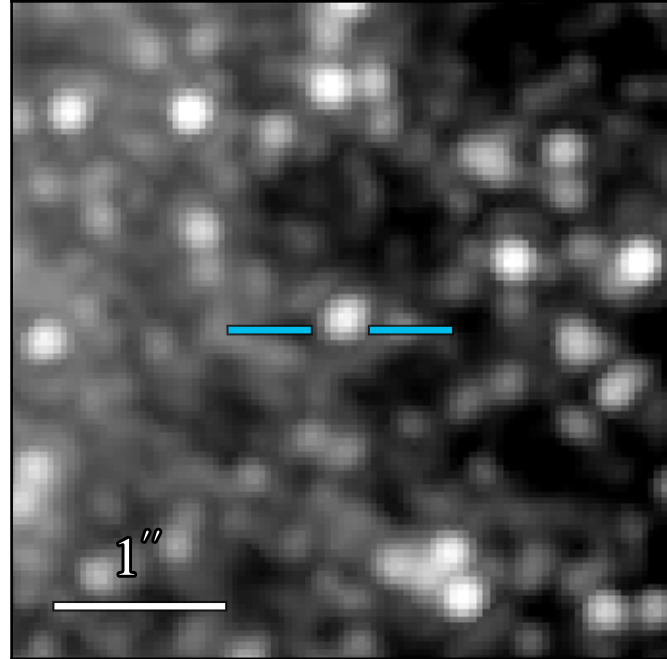
JWST/NIRCam F430M
