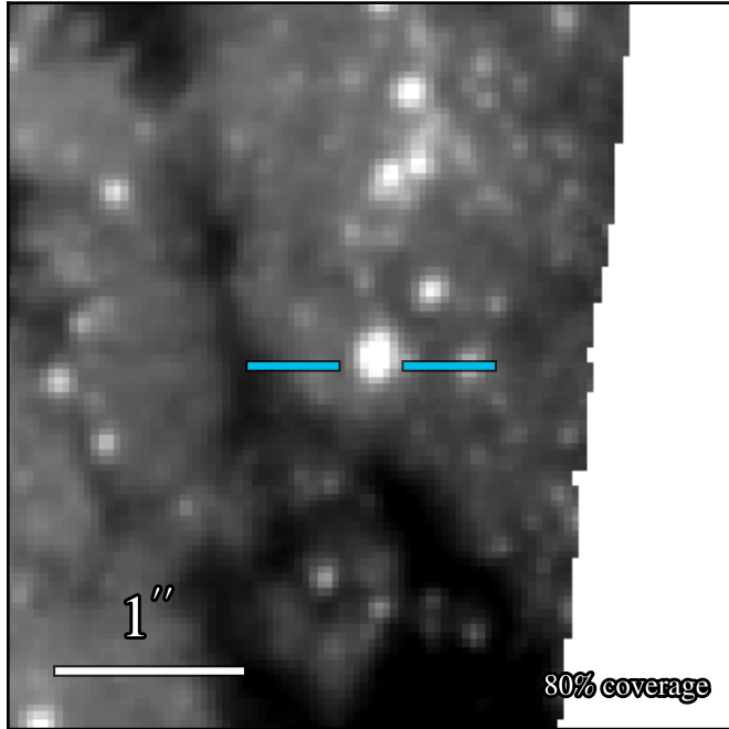
WFC3 F606W 20.620 ± 0.008
