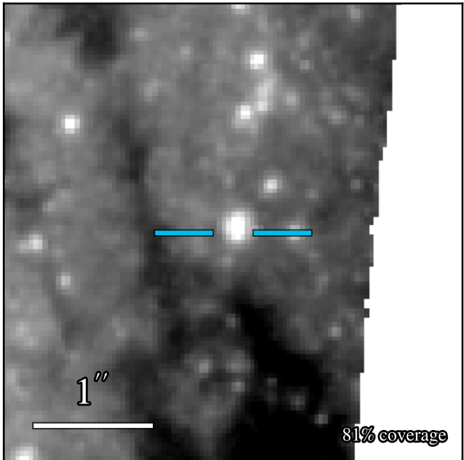
WFC3 F814W 20.253 ± 0.009
