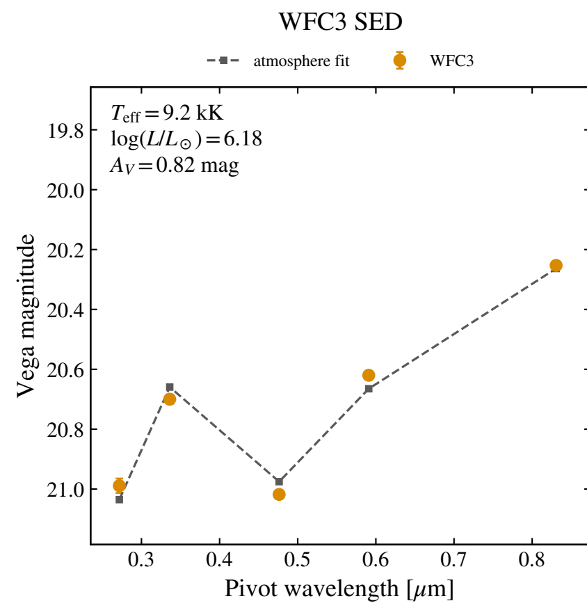
WFC3 F606W 20.620 ± 0.008
