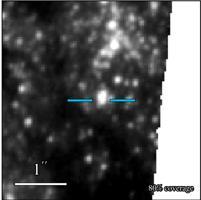
WFC3 F336W 20.700 ± 0.016
