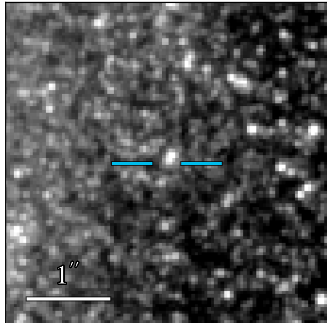
JWST/NIRCam F182M
