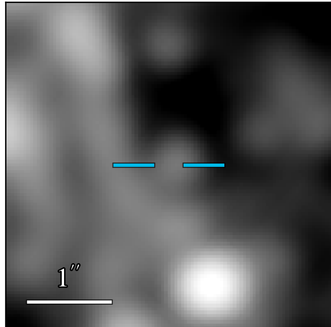
JWST/MIRI F1500W
