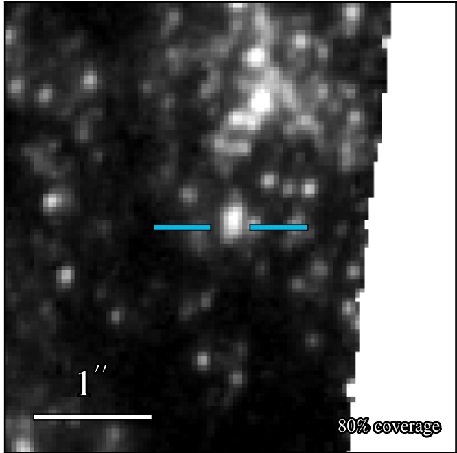
WFC3 F275W 20.989 ± 0.024
