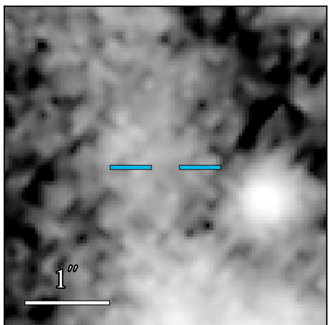
JWST/MIRI F2100W
