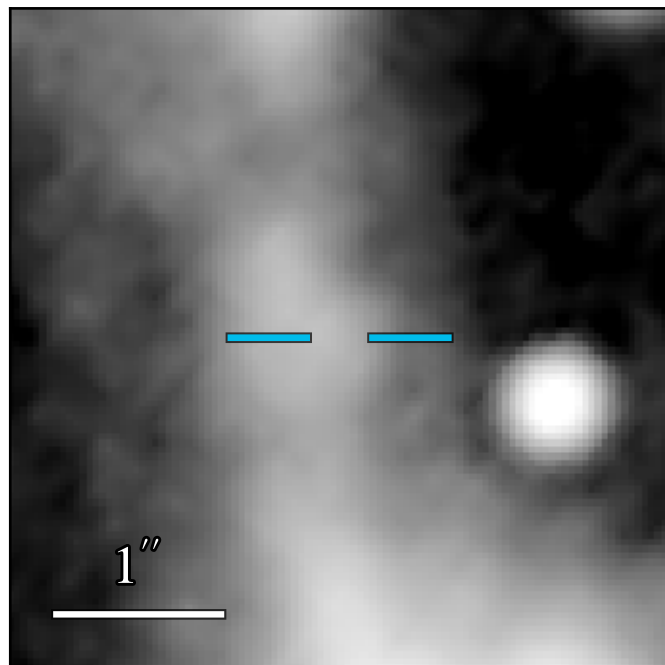
JWST/MIRI F1280W
