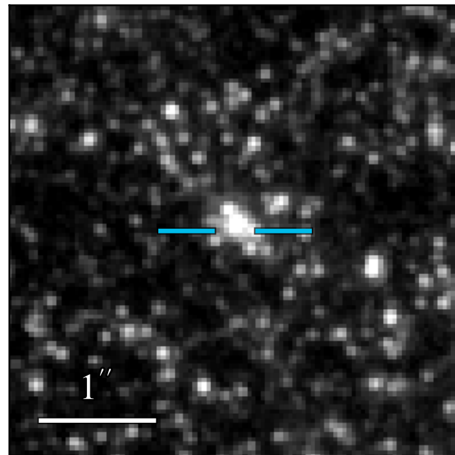
JWST/NIRCam F210M
