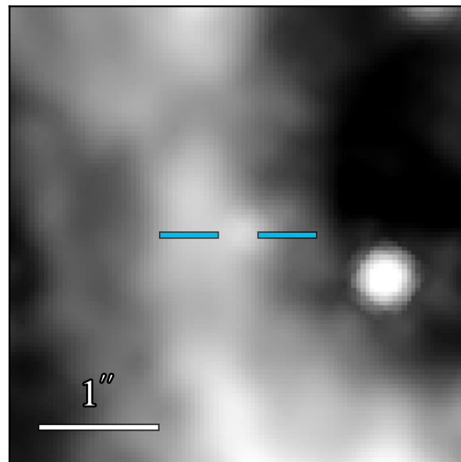
JWST/MIRI F770W
