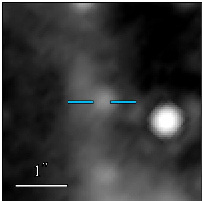
JWST/MIRI F1000W
