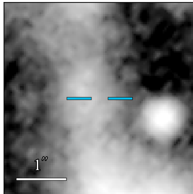
JWST/MIRI F1800W
