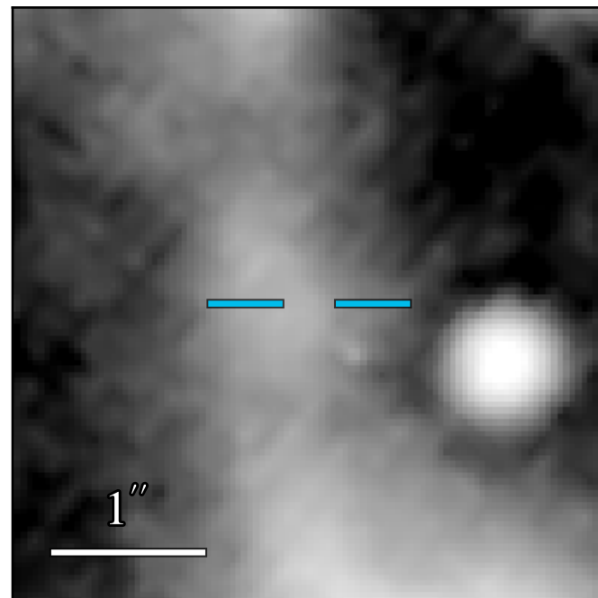
JWST/MIRI F1500W
