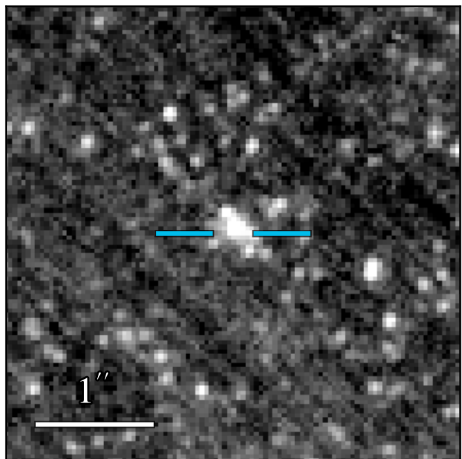
JWST/NIRCam F212N
