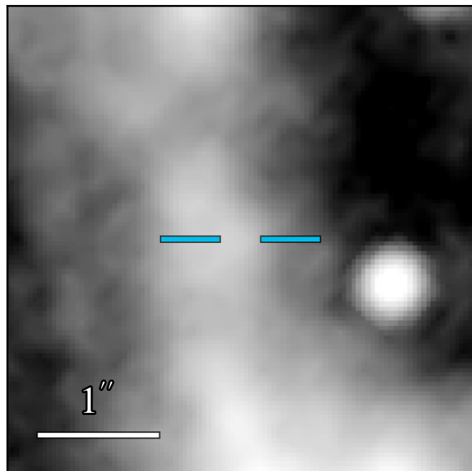
JWST/MIRI F1130W
