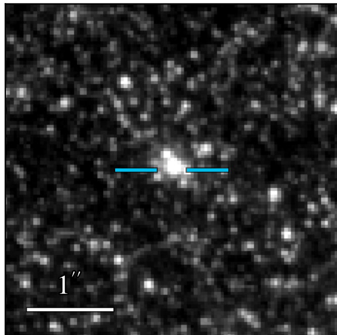
JWST/NIRCam F140M
