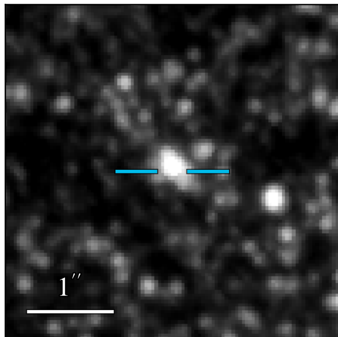
JWST/NIRCam F250M
