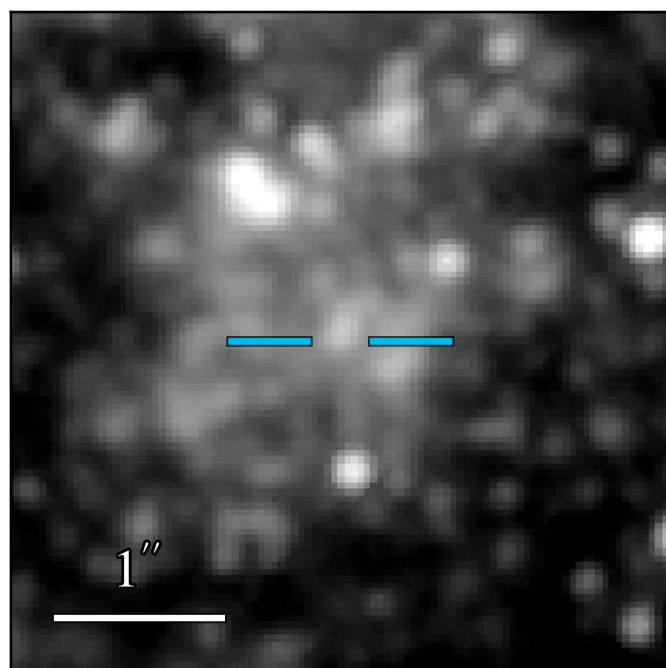
JWST/NIRCam F430M
