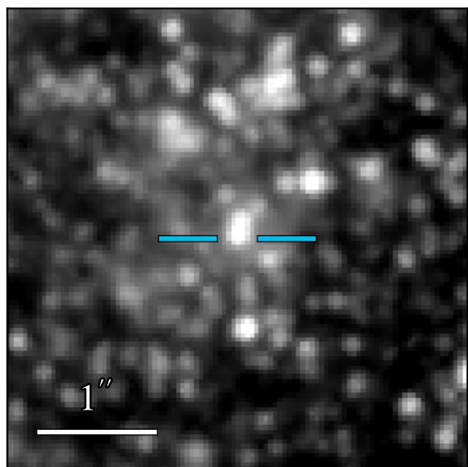
JWST/NIRCam F250M
