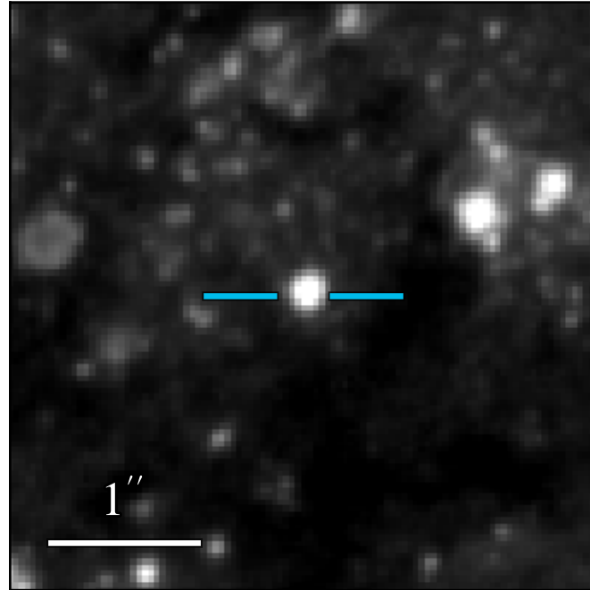
WFC3 F606W 20.953 ± 0.006
