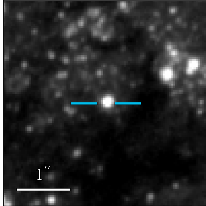
WFC3 F475W 21.381 ± 0.006
