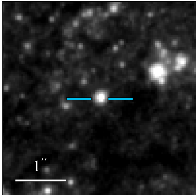
WFC3 F814W 20.435 ± 0.005
