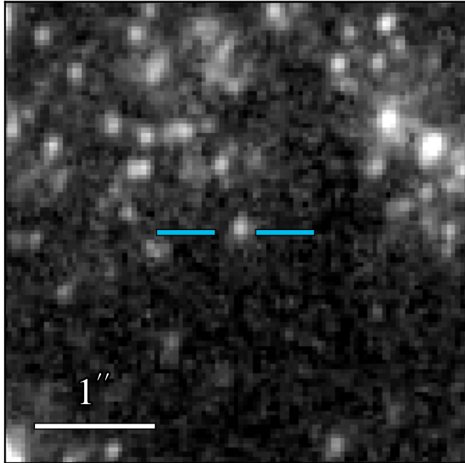
WFC3 F275W 23.398 ± 0.066
