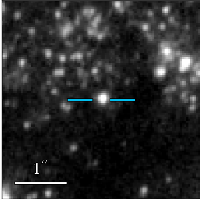
WFC3 F336W 21.525 ± 0.014
