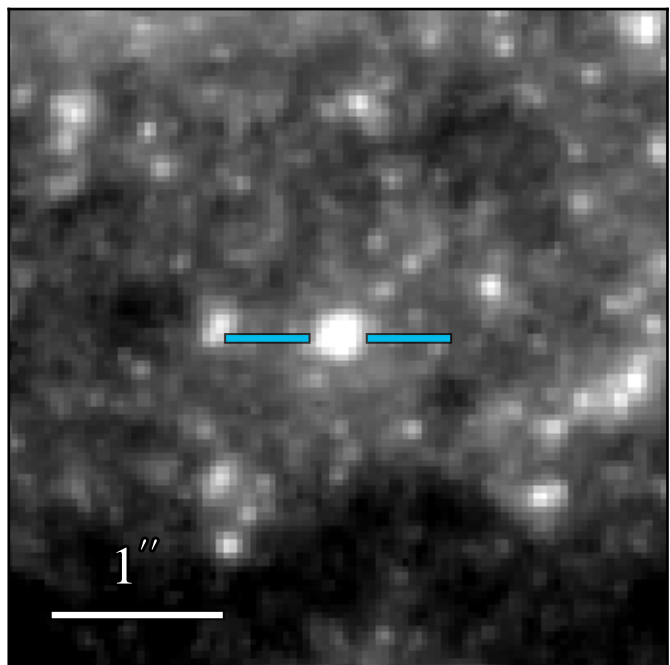
WFC3 F814W 20.353 ± 0.006
