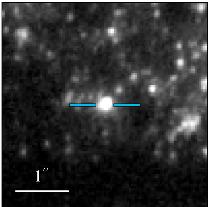
WFC3 F336W 20.005 ± 0.007
