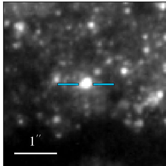
WFC3 F475W 20.971 ± 0.004
