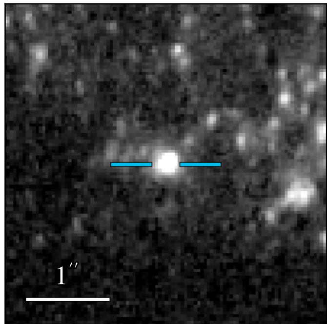
WFC3 F275W 19.959 ± 0.010
