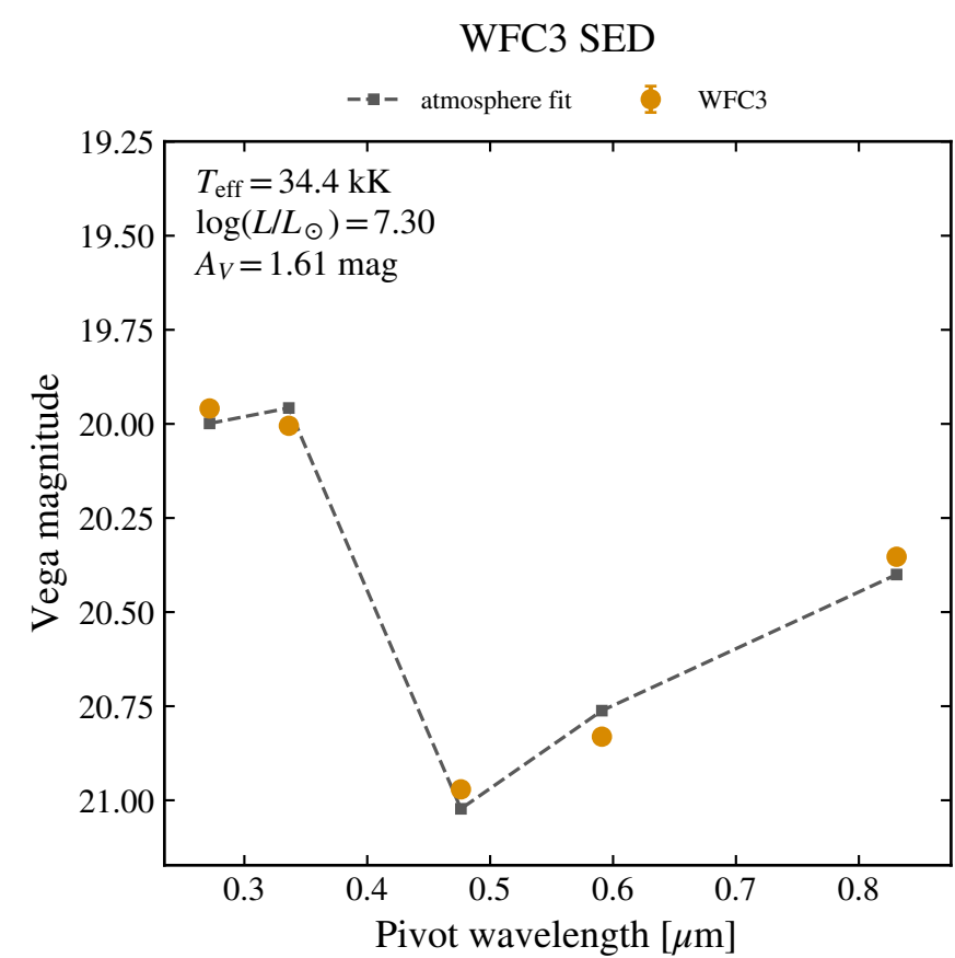
WFC3 F606W 20.831 ± 0.004
