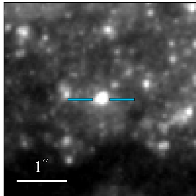
WFC3 F606W 20.831 ± 0.004
