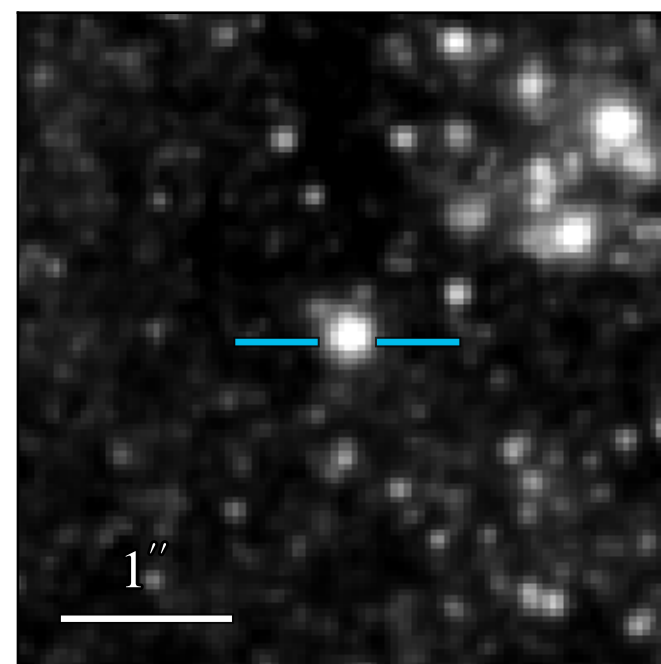
WFC3 F475W 21.776 ± 0.019
