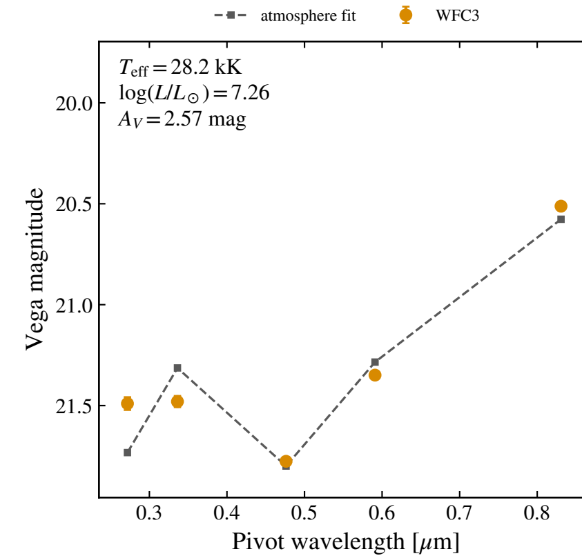
WFC3 SED
