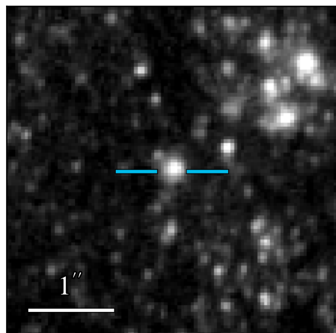
WFC3 F275W 21.490 ± 0.032
