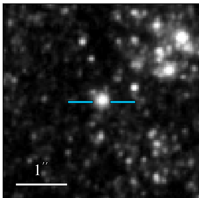
WFC3 F336W 21.480 ± 0.028
