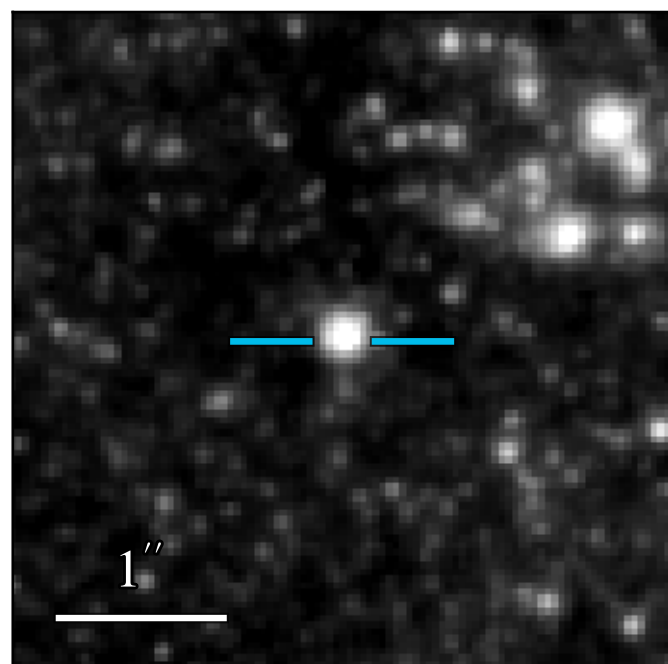
WFC3 F814W 20.512 ± 0.014
