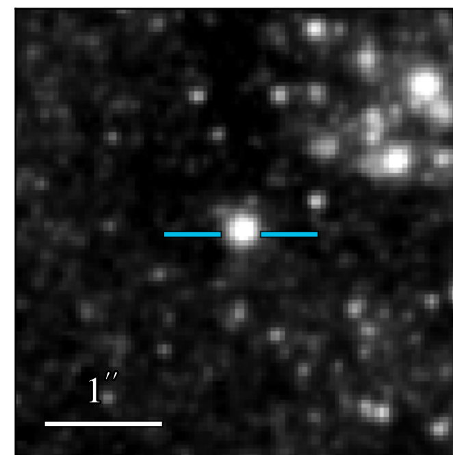
WFC3 F606W 21.349 ± 0.016
