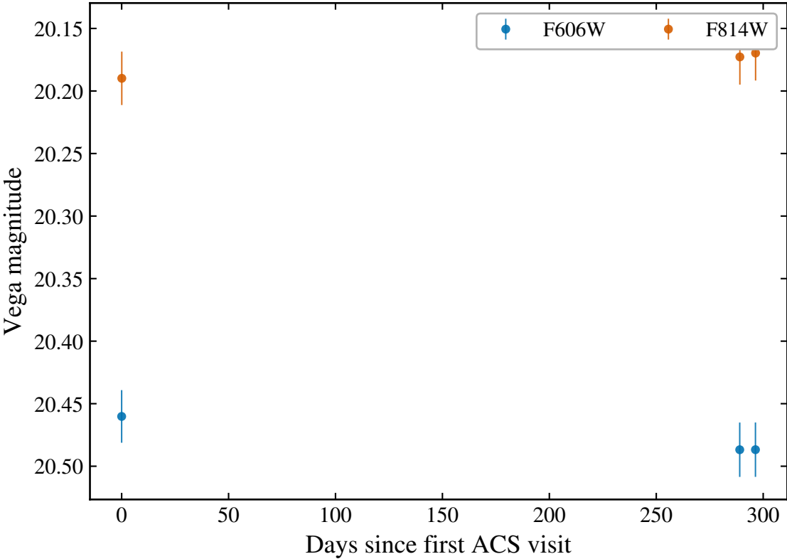
ACS visit light curves
