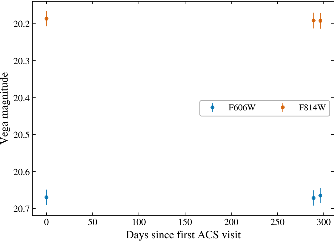
ACS visit light curves
