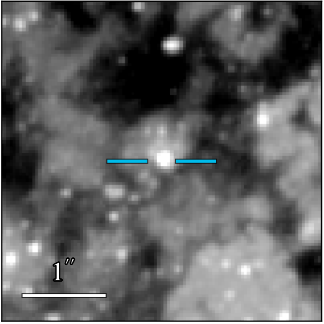
WFC3 F475W 21.347 ± 0.006
