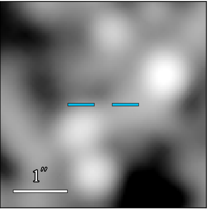
JWST/MIRI F1800W
