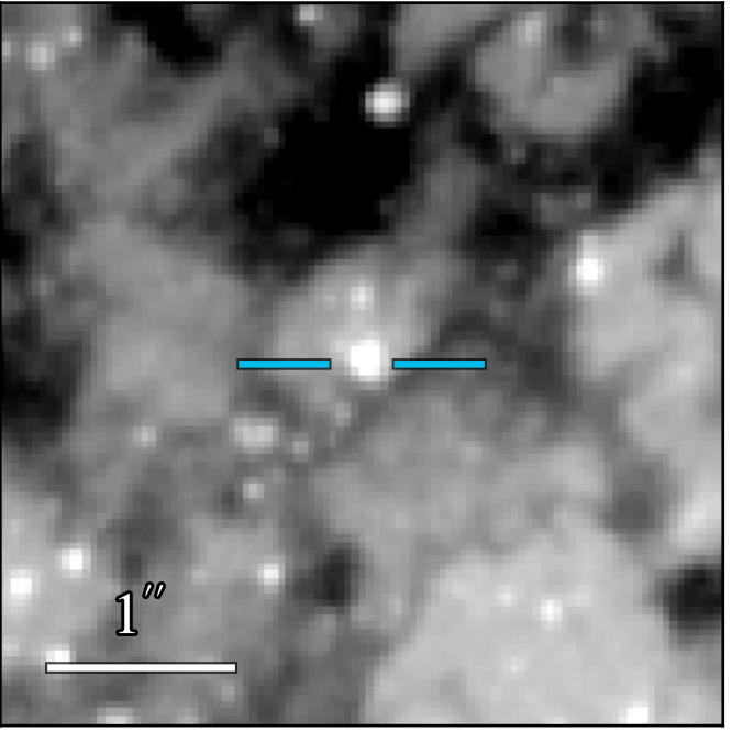
WFC3 F606W 21.022 ± 0.005
