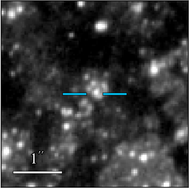
WFC3 F336W 22.038 ± 0.022
