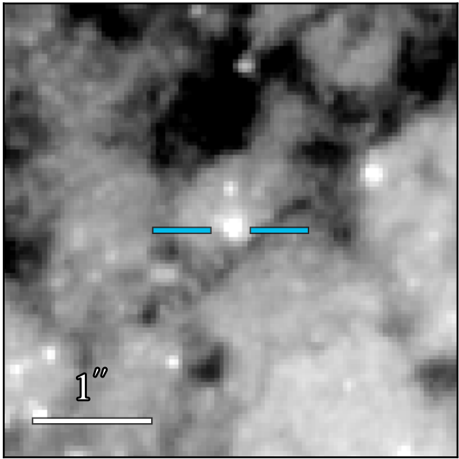
WFC3 F814W 20.681 ± 0.008
