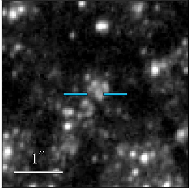
WFC3 F275W 23.381 ± 0.080
