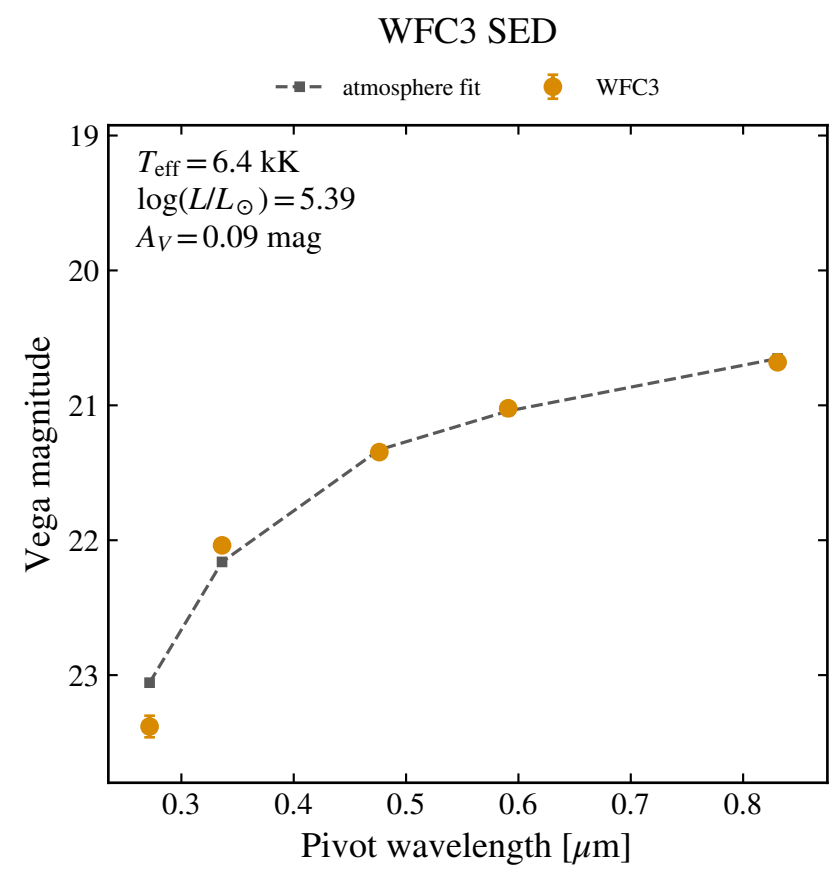
WFC3 F606W 21.022 ± 0.005
