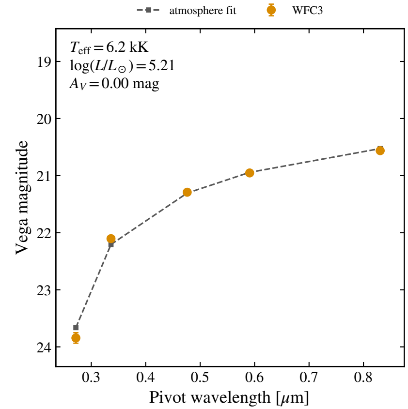
WFC3 SED
