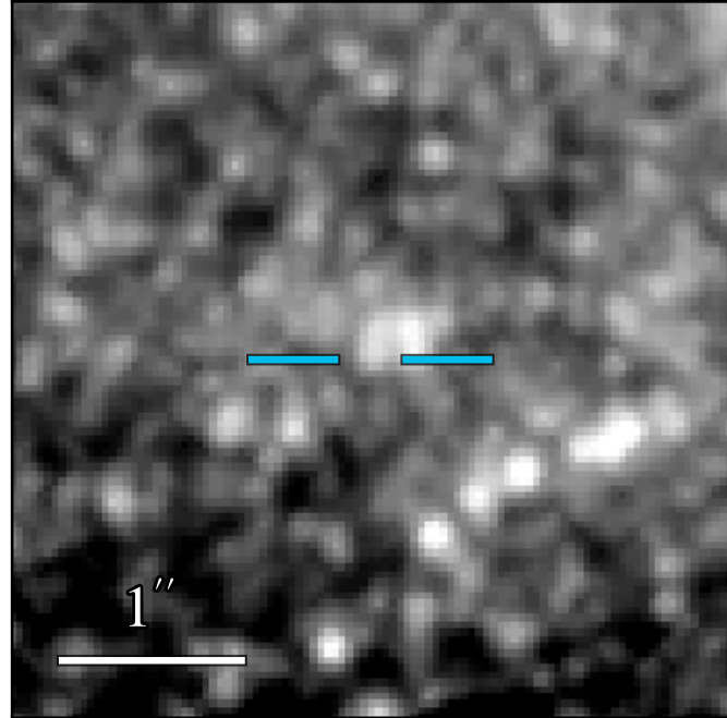
JWST/NIRCam F250M
