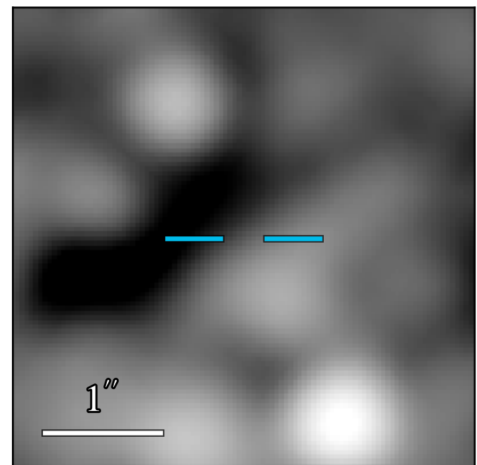
JWST/MIRI F1800W
