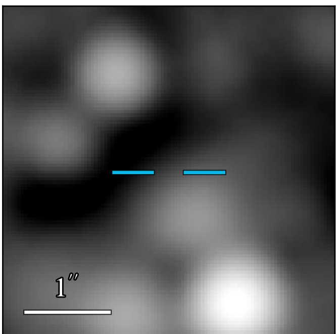
JWST/MIRI F2100W
