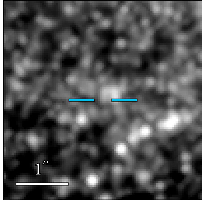
JWST/NIRCam F360M
