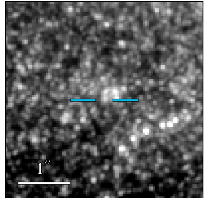
JWST/NIRCam F210M
