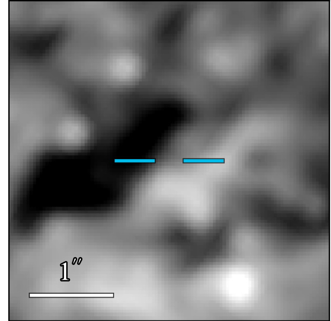
JWST/MIRI F770W
