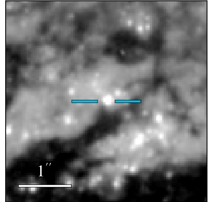
WFC3 F606W 21.114 ± 0.006
