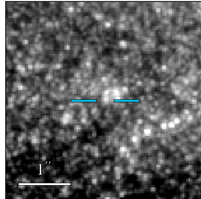
JWST/NIRCam F182M
