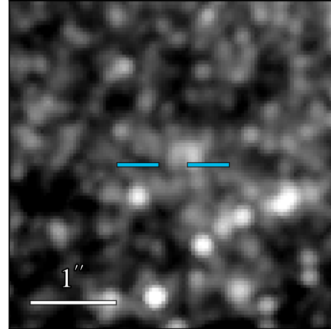
JWST/NIRCam F430M
