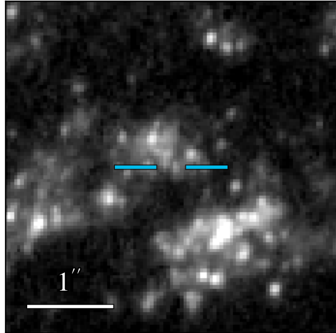
WFC3 F275W 23.710 ± 0.105
