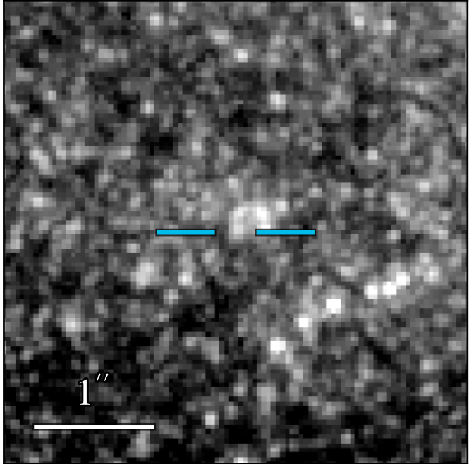
JWST/NIRCam F212N
