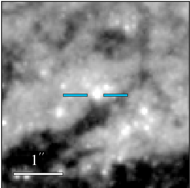
WFC3 F814W 20.613 ± 0.008
