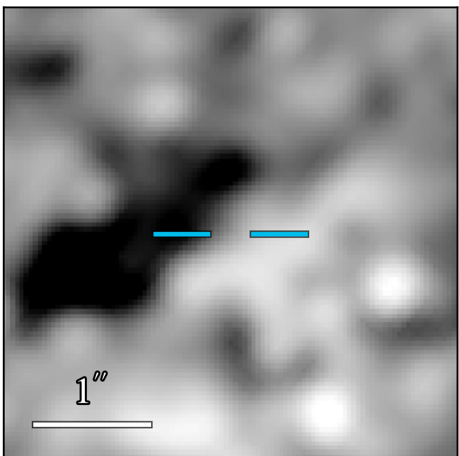
JWST/MIRI F1000W
