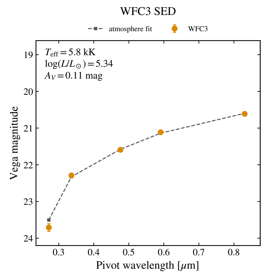
WFC3 F606W 21.114 ± 0.006
