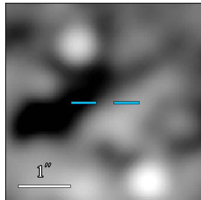
JWST/MIRI F1500W
