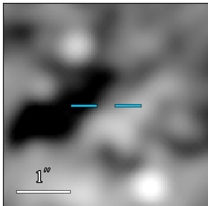
JWST/MIRI F1280W
