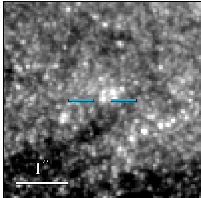
JWST/NIRCam F140M
