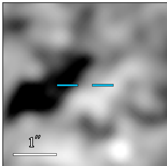
JWST/MIRI F1130W
