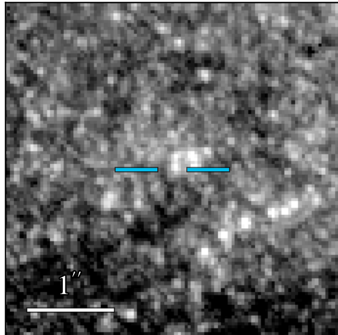
JWST/NIRCam F164N
