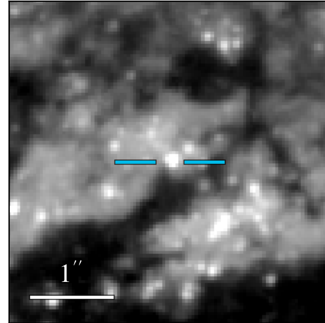
WFC3 F475W 21.592 ± 0.006
