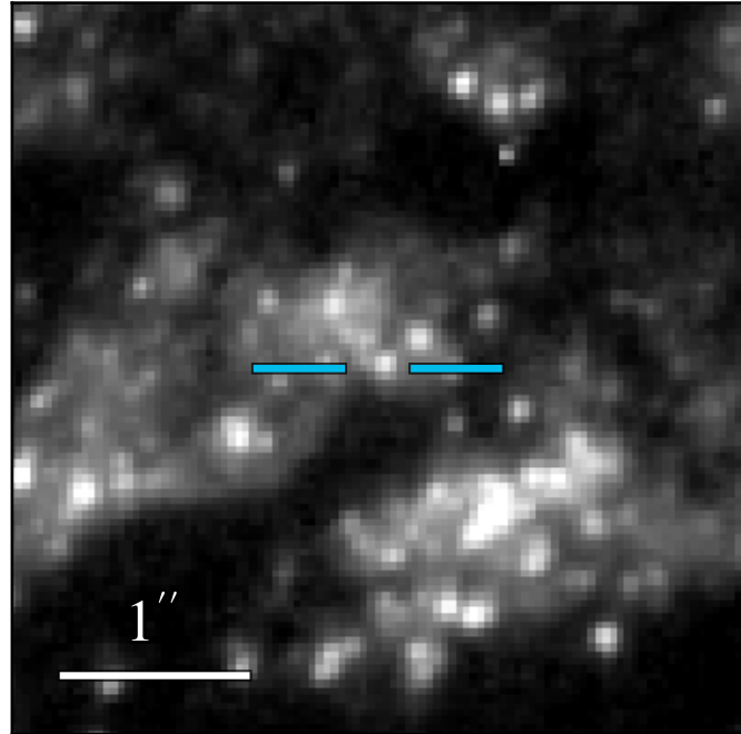
WFC3 F336W 22.290 ± 0.023
