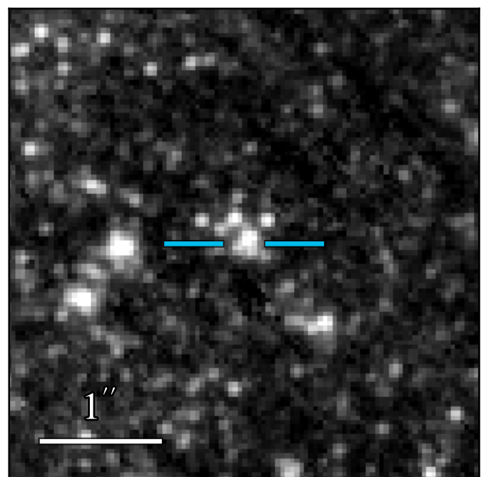
JWST/NIRCam F212N
