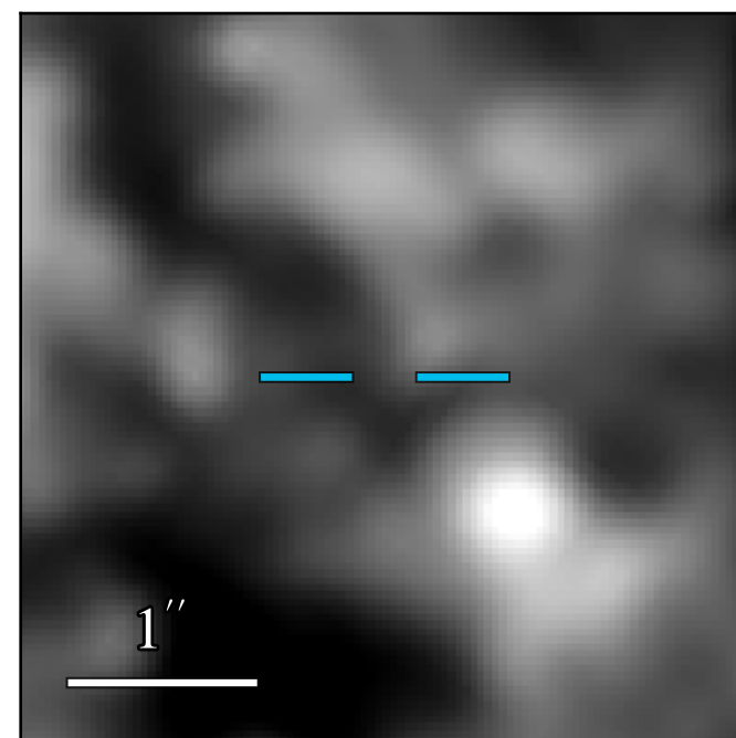
JWST/MIRI F770W
