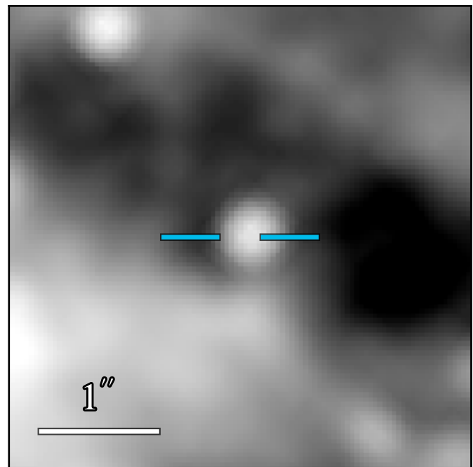
JWST/MIRI F1000W
