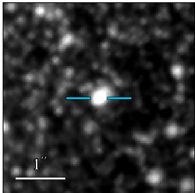
JWST/NIRCam F250M
