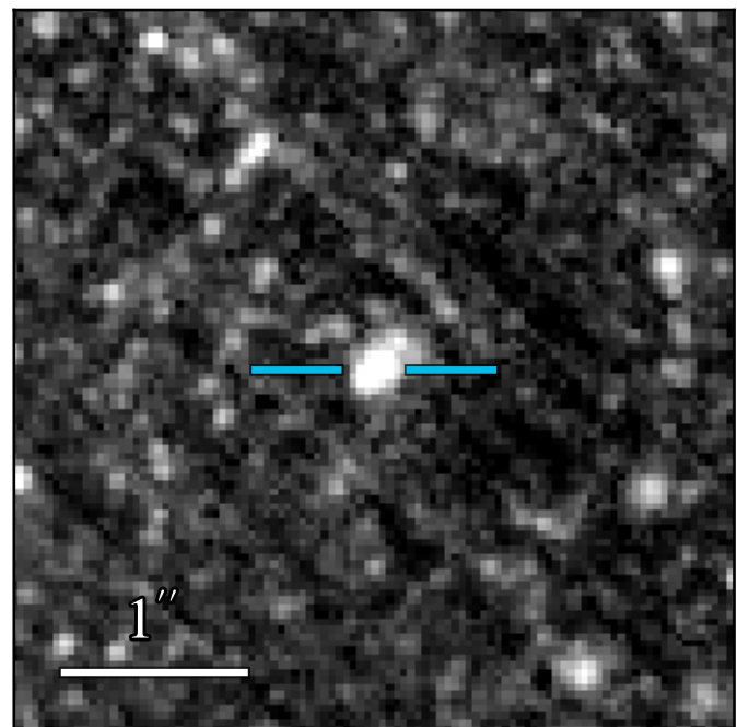
JWST/NIRCam F212N
