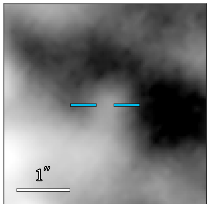
JWST/MIRI F2100W
