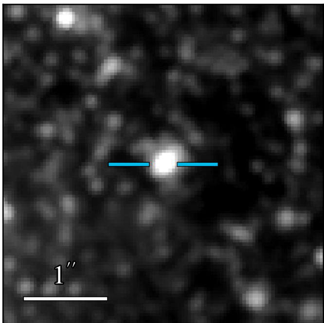
JWST/NIRCam F360M
