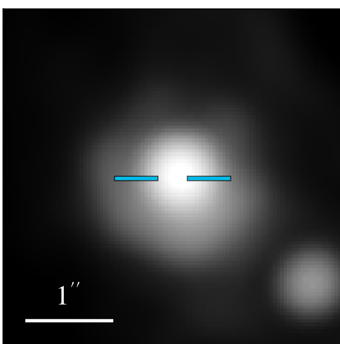
JWST/MIRI F1500W
