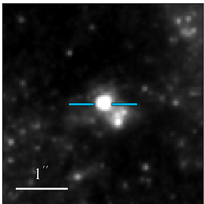
WFC3 F814W 18.487 ± 0.005
