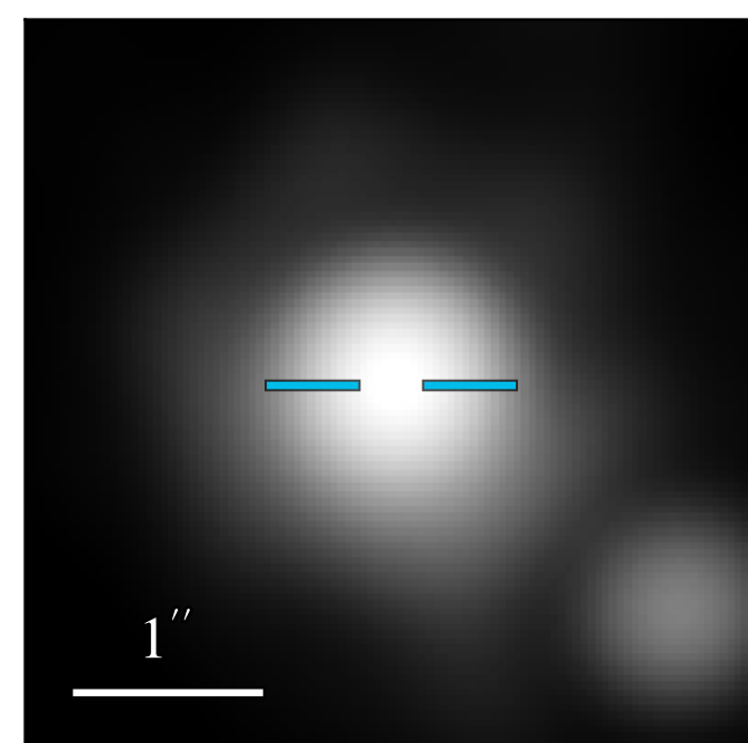
JWST/MIRI F2100W
