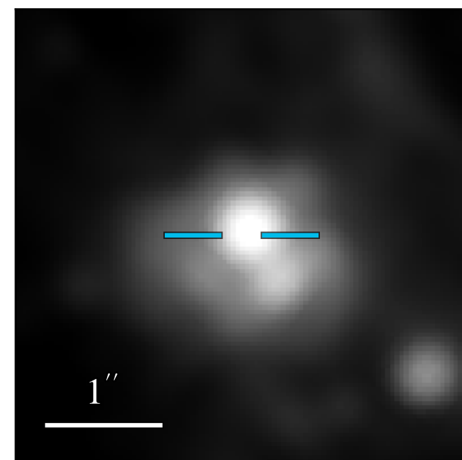
JWST/MIRI F1000W
