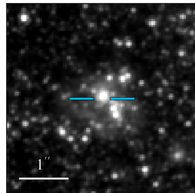
JWST/NIRCam F210M
