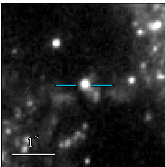
WFC3 F336W 20.534 ± 0.009
