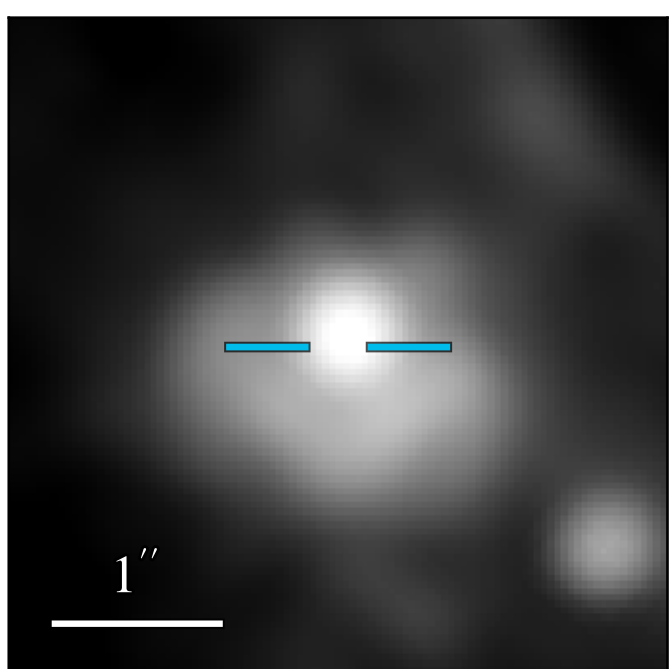
JWST/MIRI F1130W
