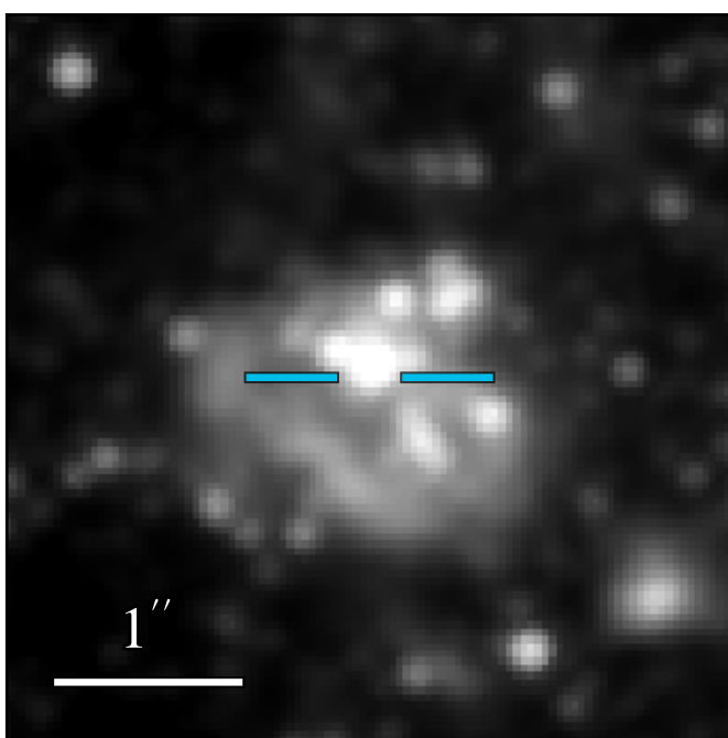
JWST/NIRCam F360M
