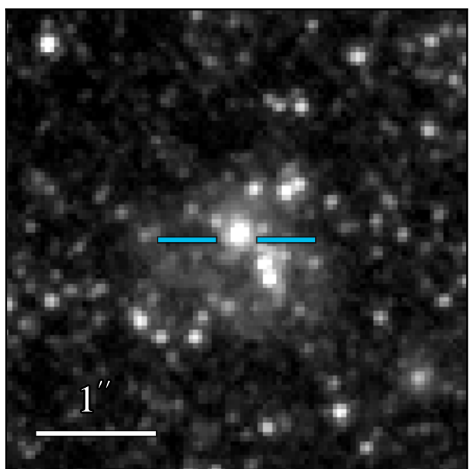
JWST/NIRCam F212N
