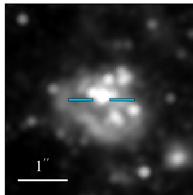
JWST/NIRCam F430M
