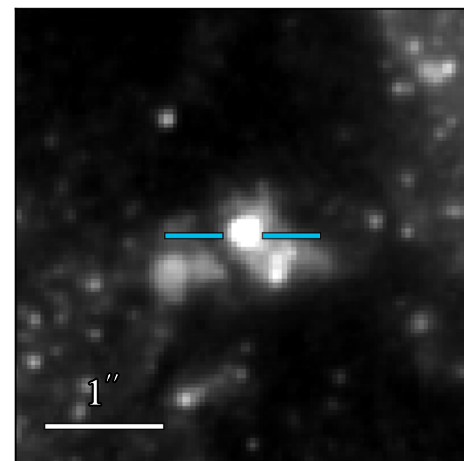
WFC3 F606W 19.296 ± 0.005
