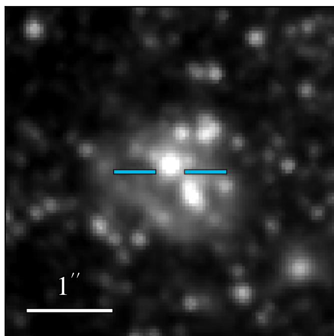
JWST/NIRCam F250M
