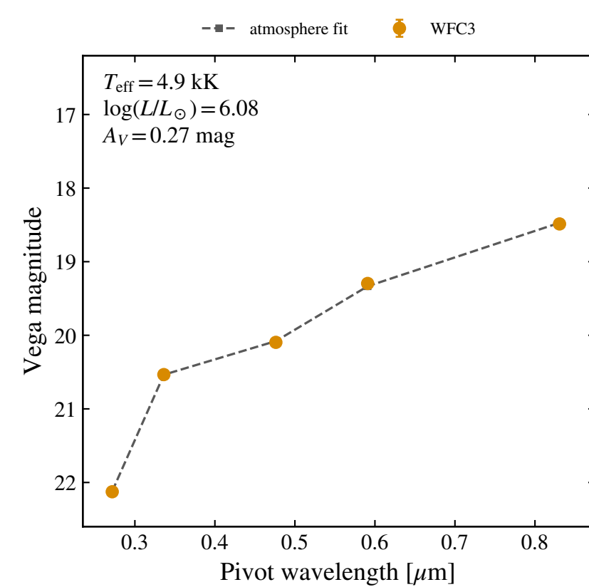
WFC3 SED
