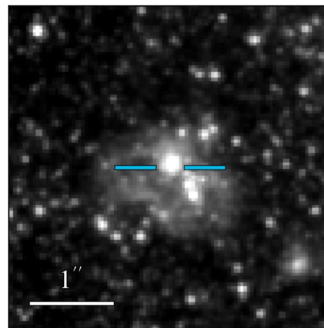
JWST/NIRCam F182M
