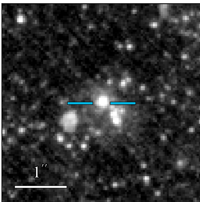
JWST/NIRCam F164N
