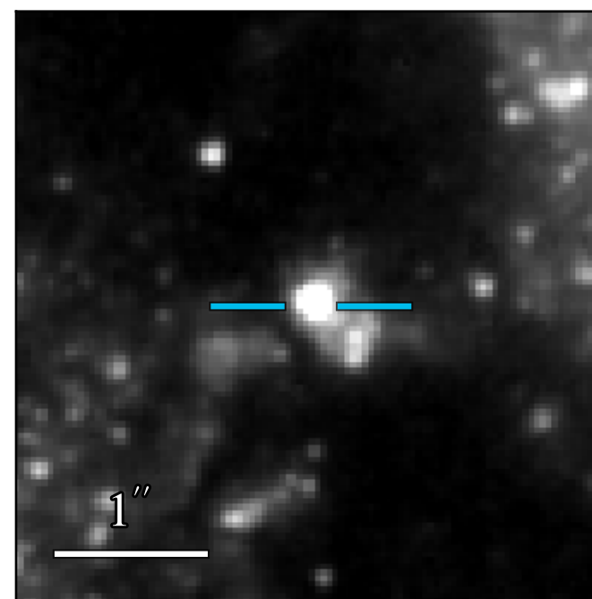
WFC3 F475W 20.096 ± 0.005
