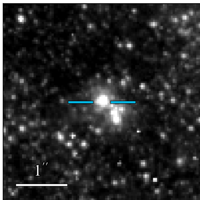
JWST/NIRCam F140M
