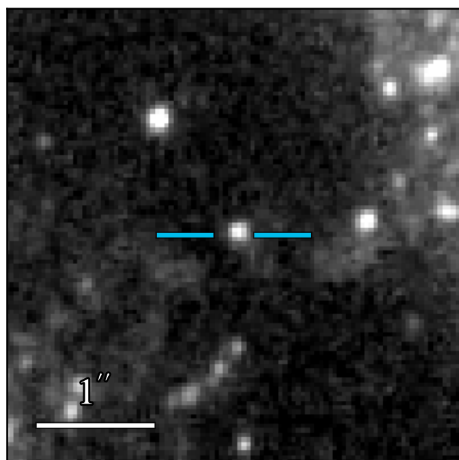
WFC3 F275W 22.126 ± 0.032
