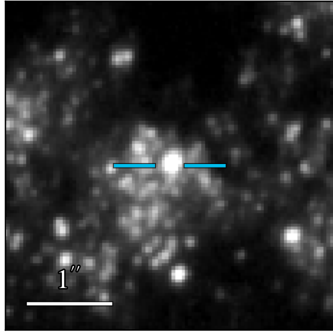
WFC3 F336W 19.049 \pm 0.004
