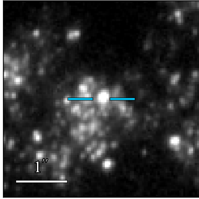
WFC3 F275W 19.212 \pm 0.006
