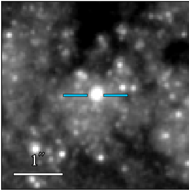
WFC3 F814W 19.227 \pm 0.003
