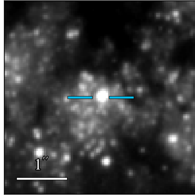
WFC3 F475W 19.824 \pm 0.002
