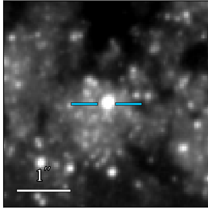
WFC3 F606W 19.569 \pm 0.002
