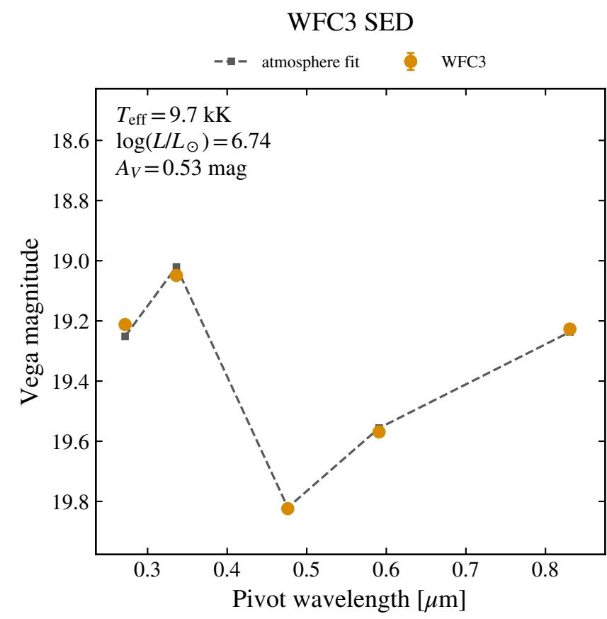
WFC3 F606W 19.569 \pm 0.002
