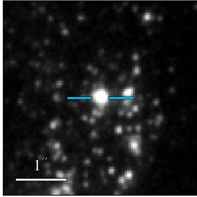
WFC3 F336W 19.121 \pm 0.004
