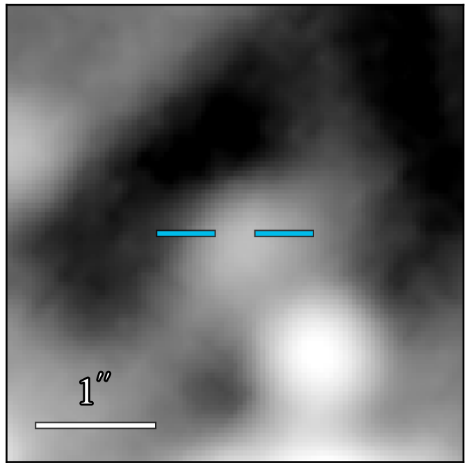
JWST/MIRI F2100W
