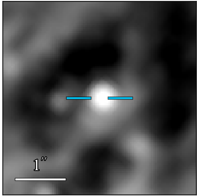
JWST/MIRI F1000W
