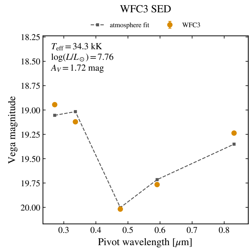
WFC3 F606W 19.766 \pm 0.002
