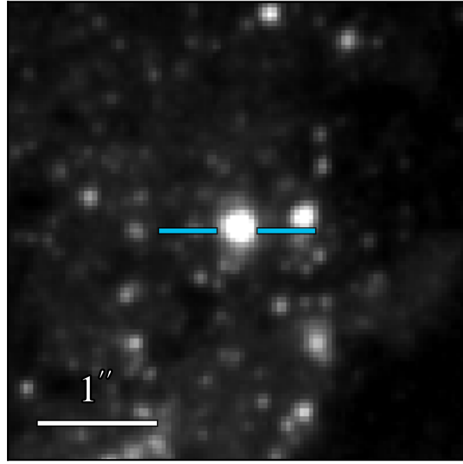
WFC3 F606W 19.766 \pm 0.002
