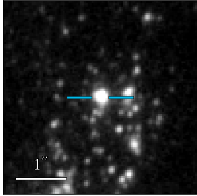
WFC3 F275W 18.945 \pm 0.005
