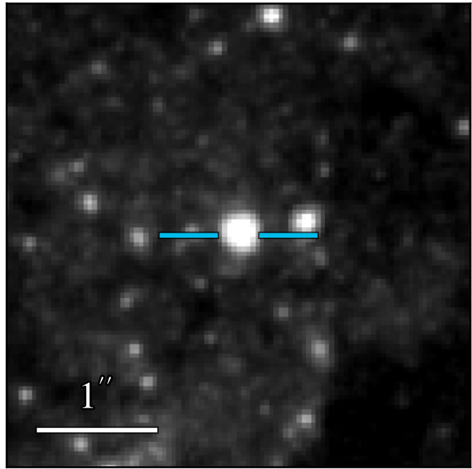
WFC3 F814W 19.237 \pm 0.003
