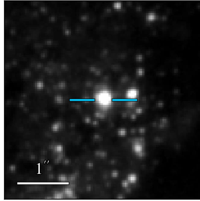
WFC3 F475W 20.018 \pm 0.002
