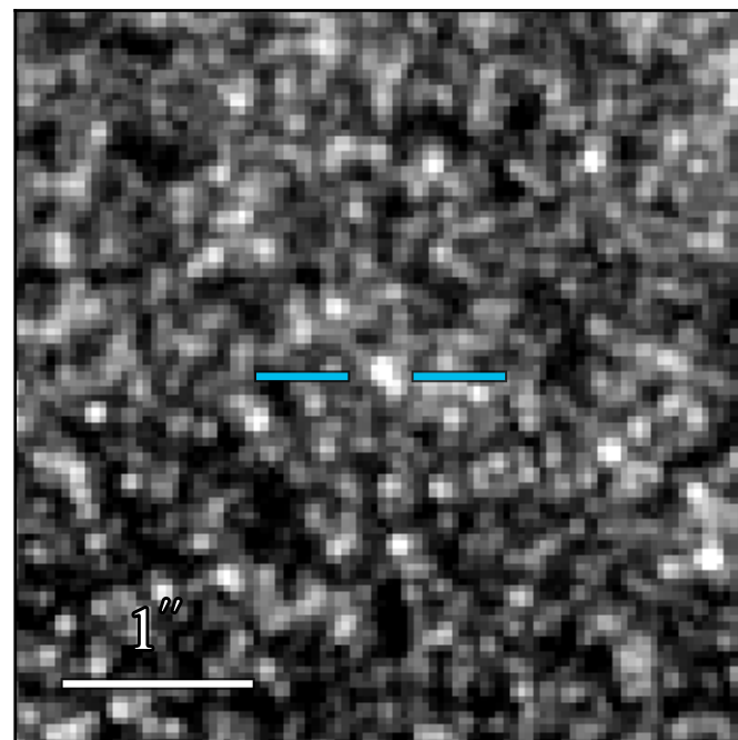
JWST/NIRCam F210M
