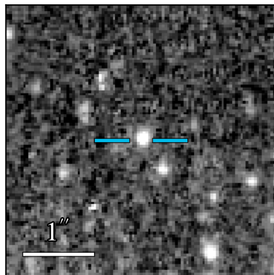
WFC3 F336W 22.477 \pm 0.025
