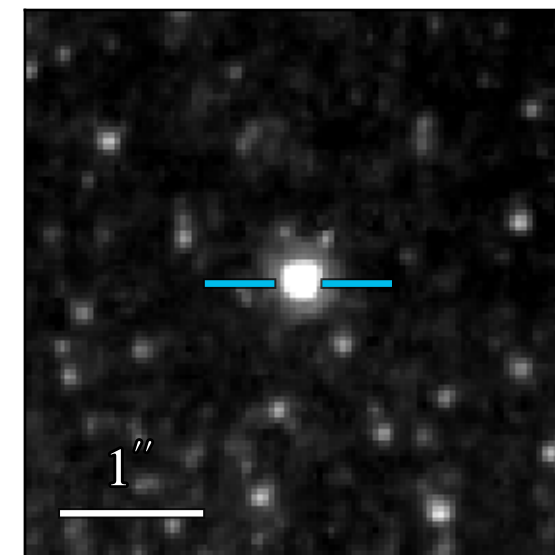
WFC3 F606W 20.380 \pm 0.003
