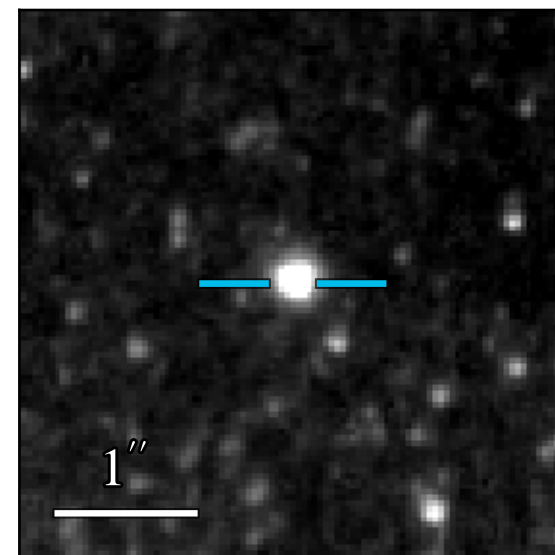
WFC3 F475W 20.953 \pm 0.004
