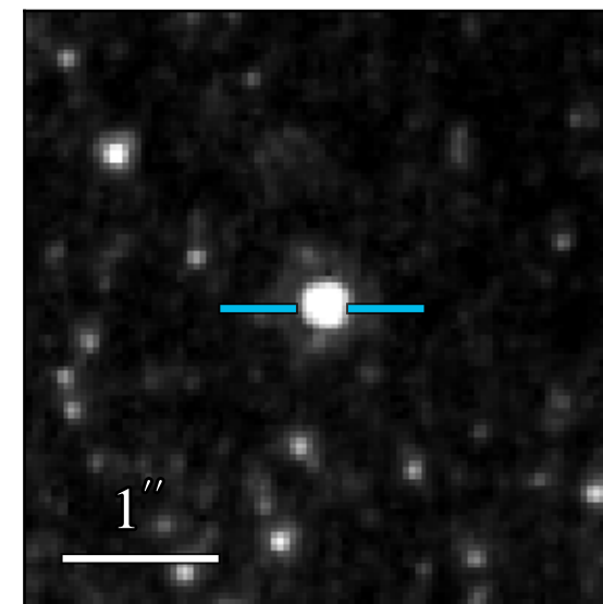
WFC3 F814W 19.796 \pm 0.004
