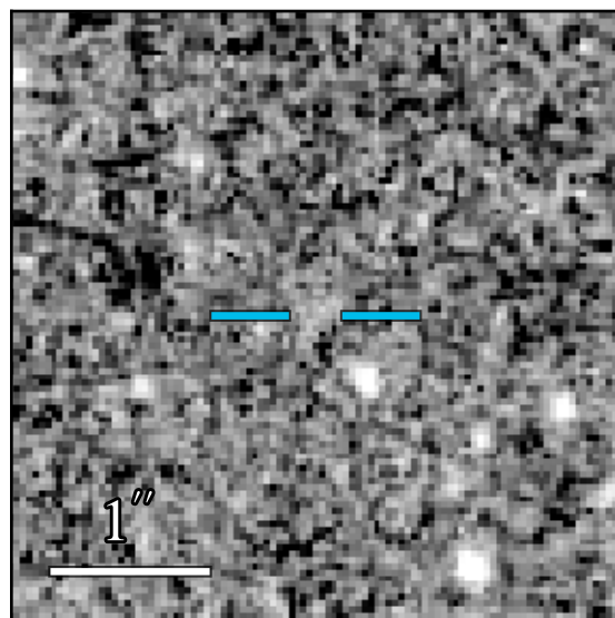
WFC3 F275W 25.718 \pm 0.466 (flagged)
