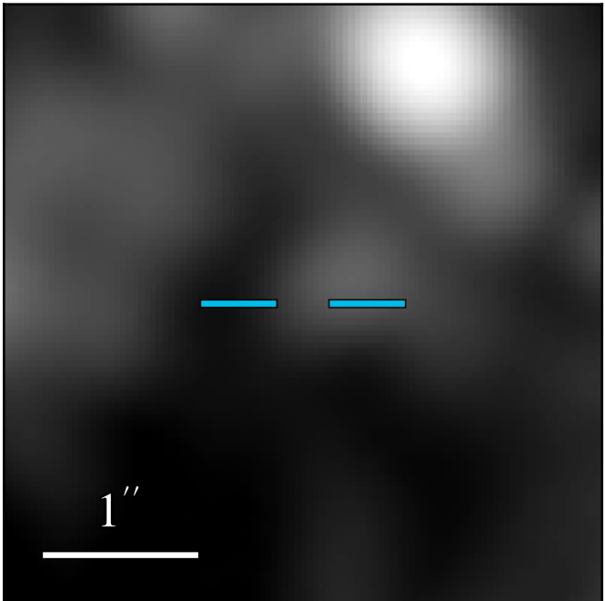
JWST/MIRI F1800W
