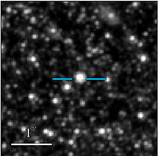
JWST/NIRCam F210M
