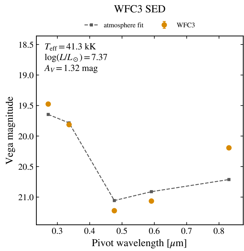
WFC3 F606W 21.065 \pm 0.015
