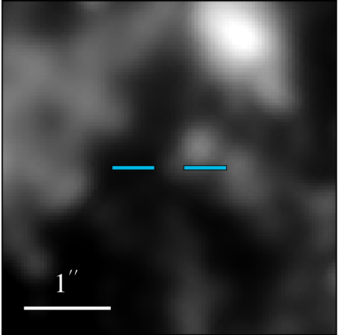
JWST/MIRI F770W
