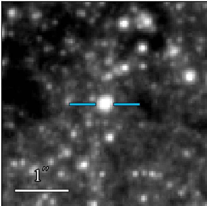
WFC3 F814W 20.193 \pm 0.010
