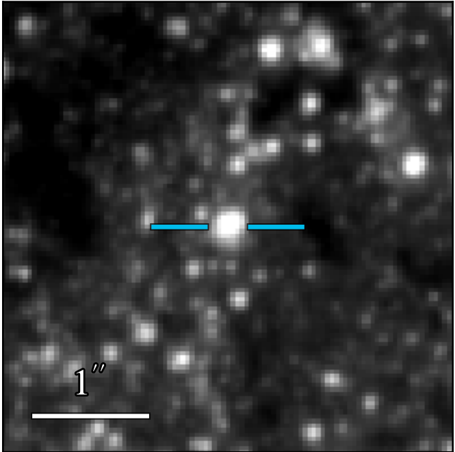
WFC3 F606W 21.065 \pm 0.015
