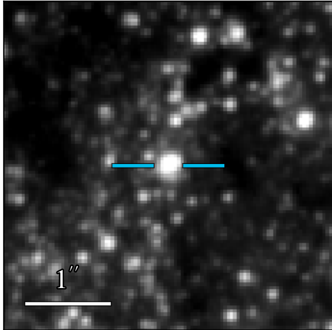
WFC3 F475W 21.223 \pm 0.017
