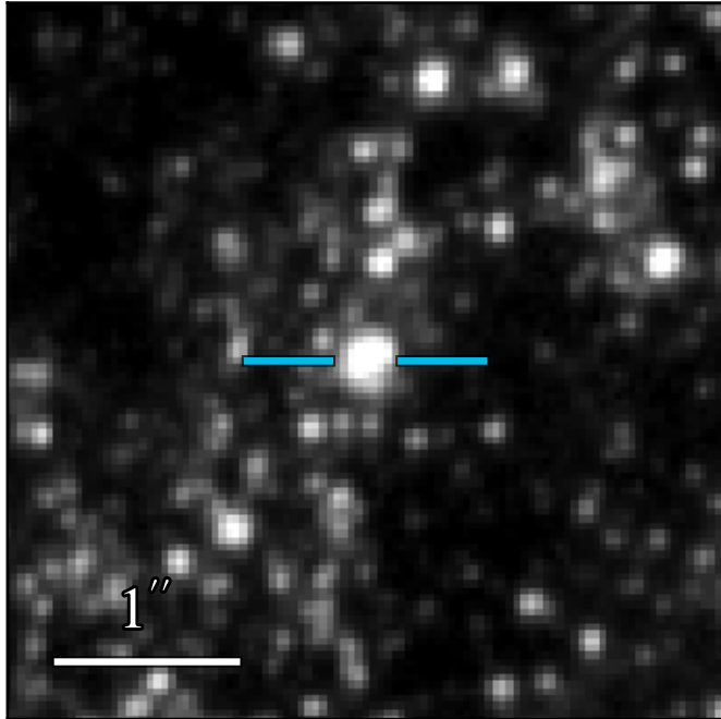
WFC3 F336W 19.813 \pm 0.017
