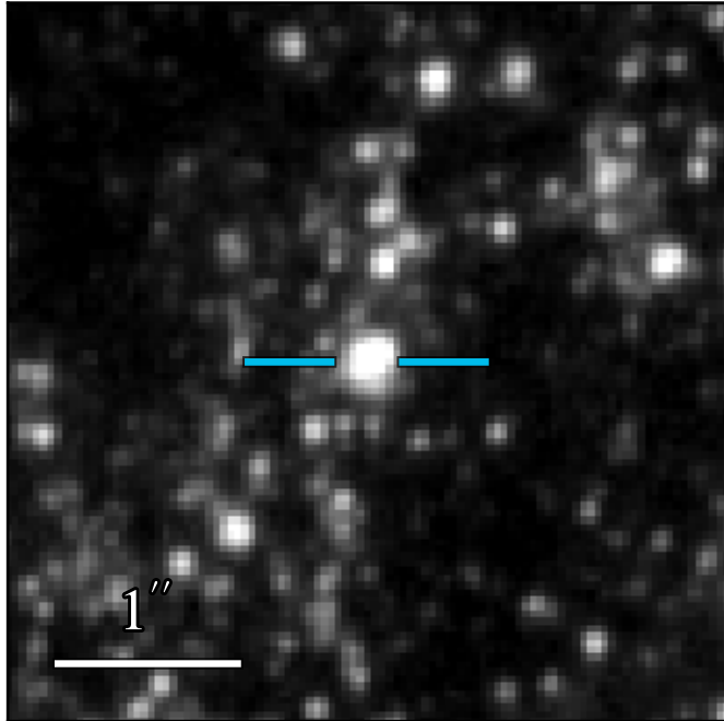
WFC3 F275W 19.476 \pm 0.018
