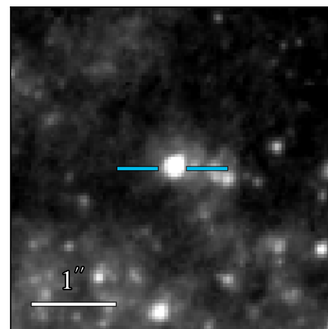
WFC3 F606W 21.182 \pm 0.004
