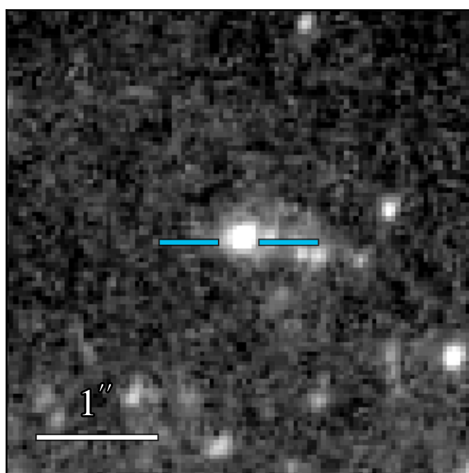
WFC3 F336W 21.319 \pm 0.011
