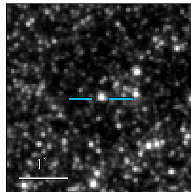
JWST/NIRCam F182M
