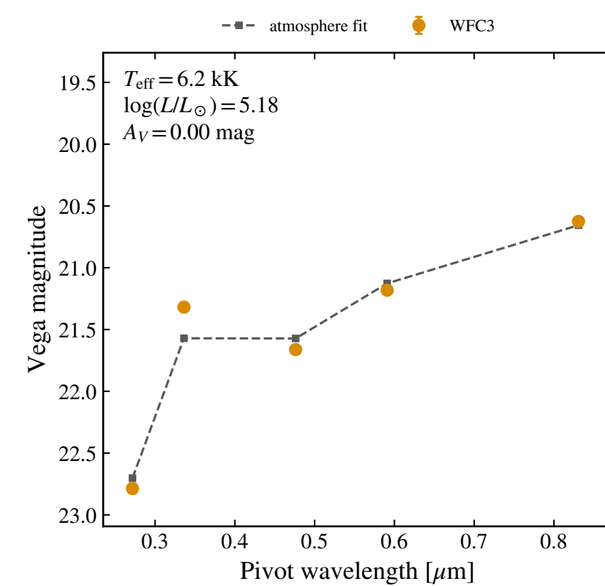
WFC3 SED
