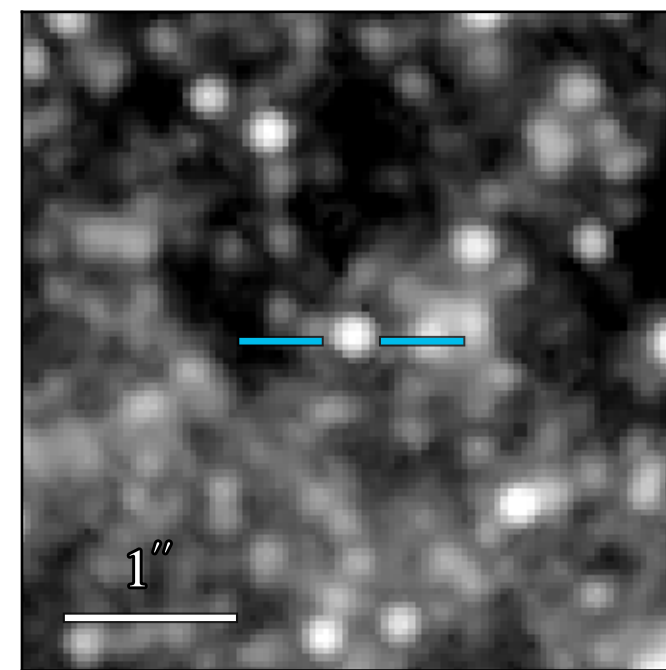
JWST/NIRCam F430M
