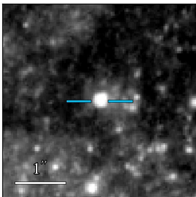
WFC3 F814W 20.625 \pm 0.005
