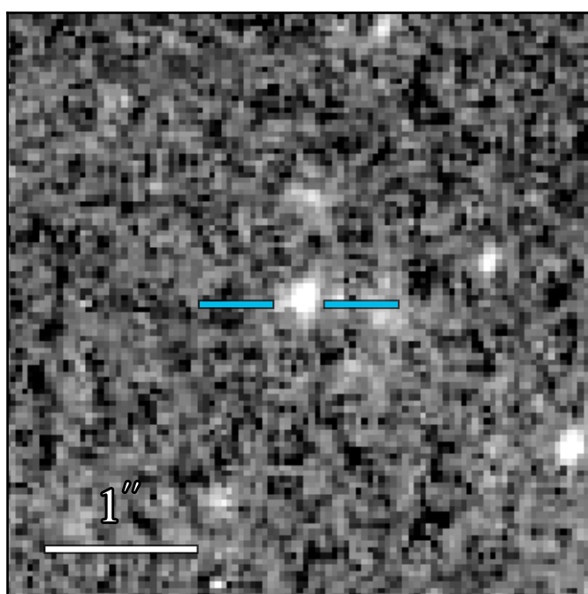
WFC3 F275W 22.787 \pm 0.041
