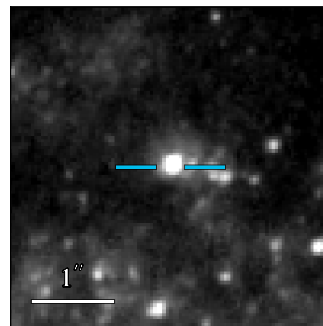
WFC3 F475W 21.662 \pm 0.005
