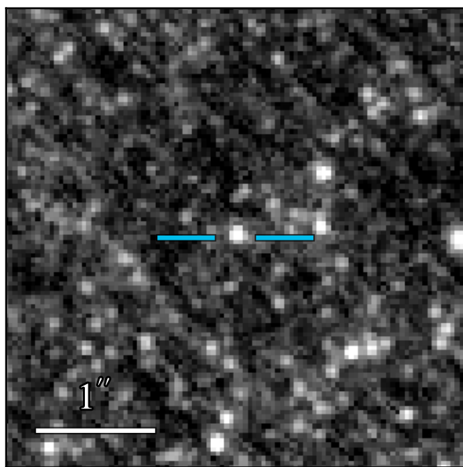
JWST/NIRCam F212N
