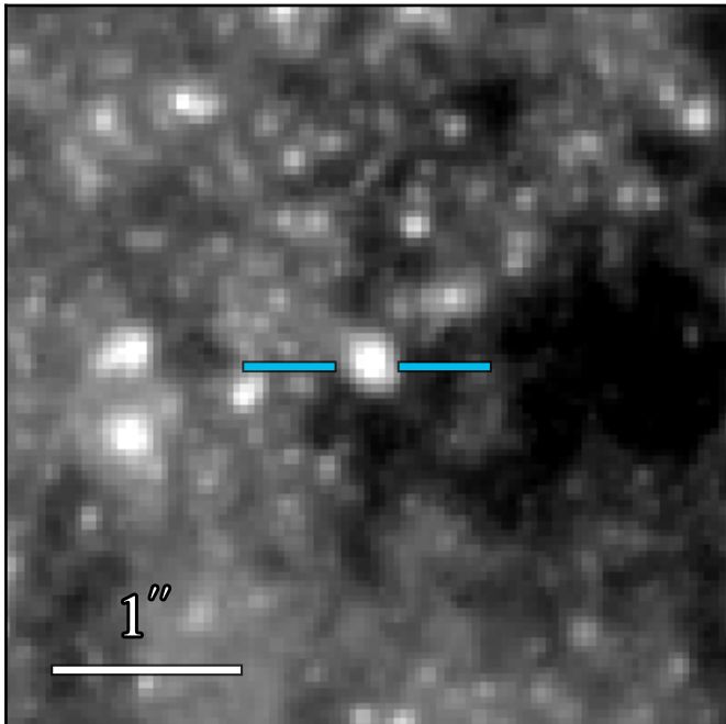
WFC3 F814W 20.281 ± 0.006
