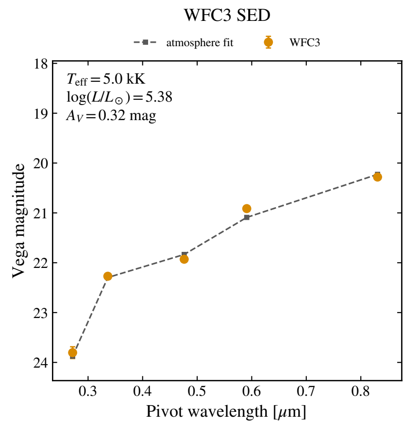
WFC3 F606W 20.914 ± 0.004
