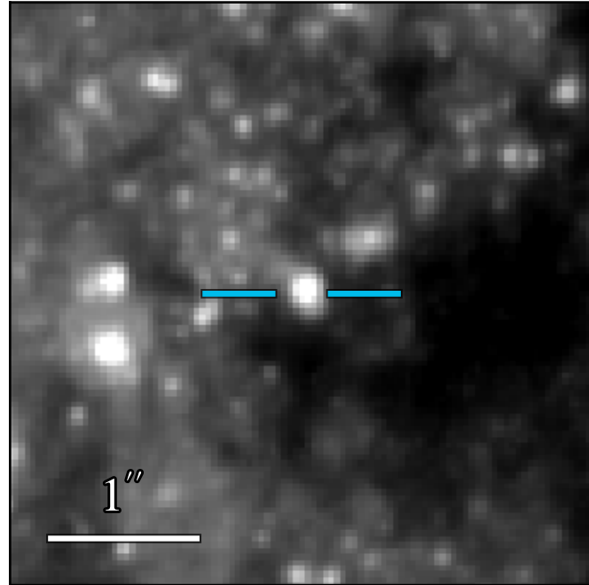
WFC3 F606W 20.914 ± 0.004
