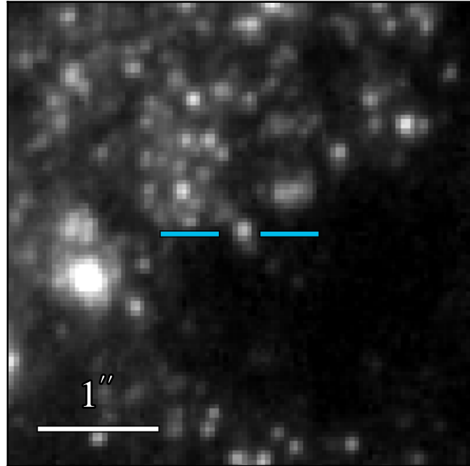
WFC3 F336W 22.271 ± 0.027
