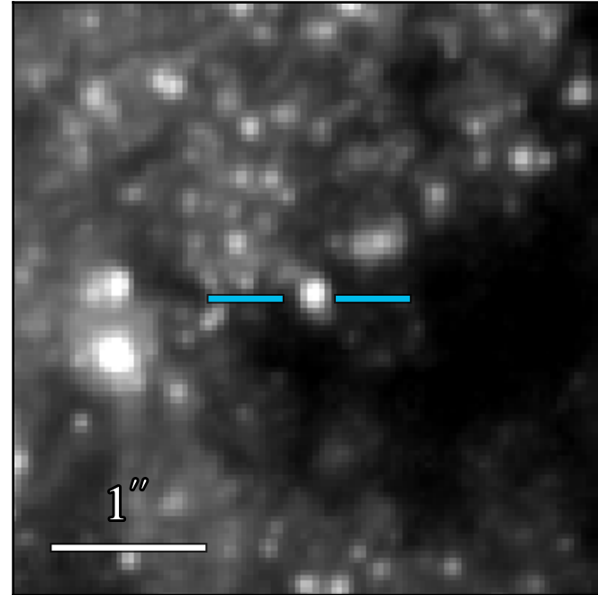
WFC3 F475W 21.930 ± 0.007
