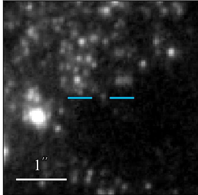
WFC3 F275W 23.804 ± 0.118
