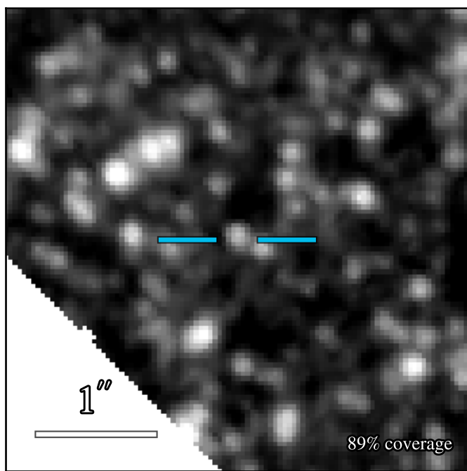
JWST/NIRCam F250M
