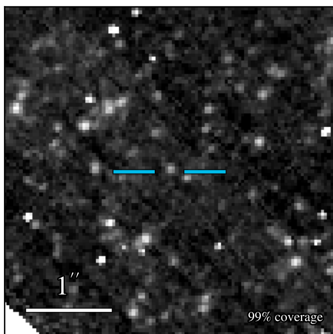
JWST/NIRCam F164N
