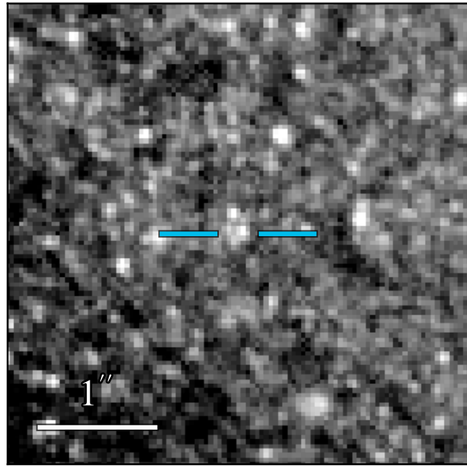
JWST/NIRCam F164N
