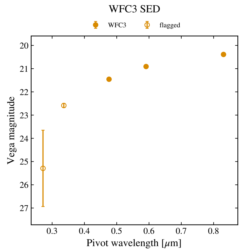
WFC3 F606W 20.909 ± 0.008
