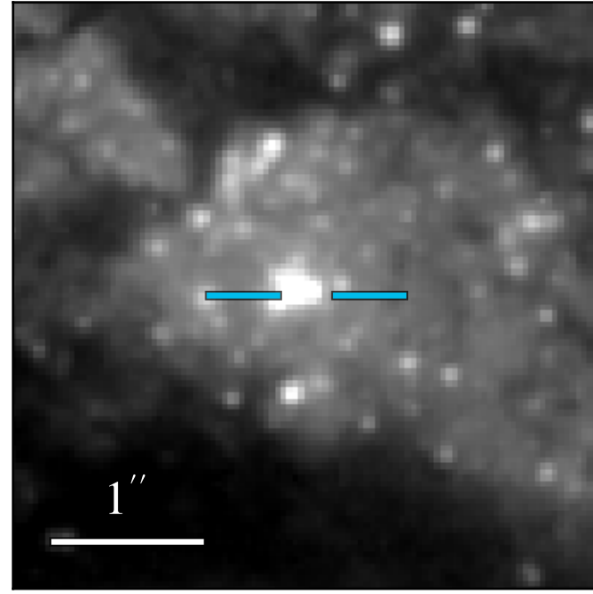
WFC3 F475W 21.456 ± 0.011
