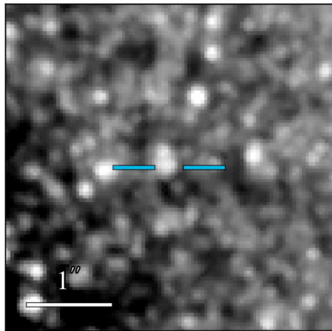
JWST/NIRCam F250M
