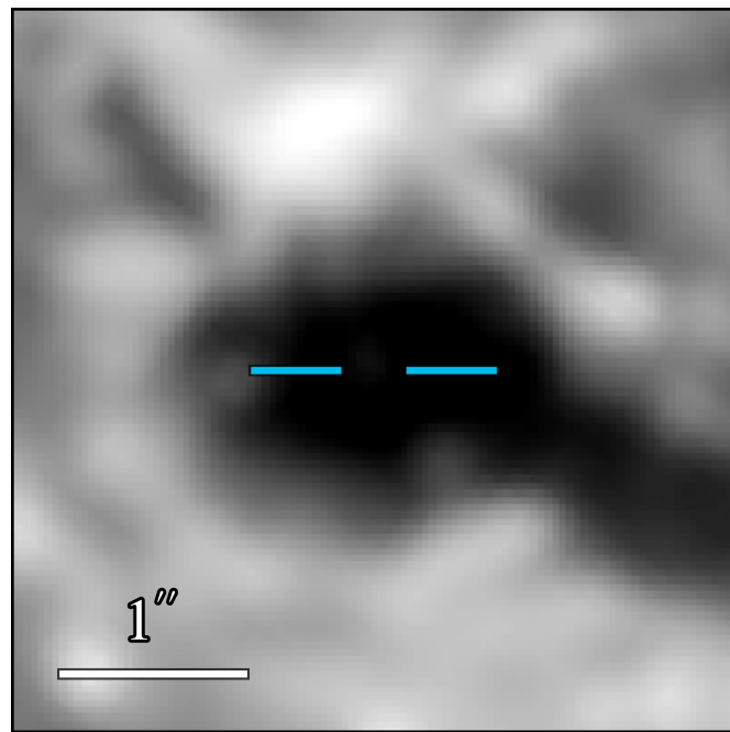
JWST/MIRI F770W
