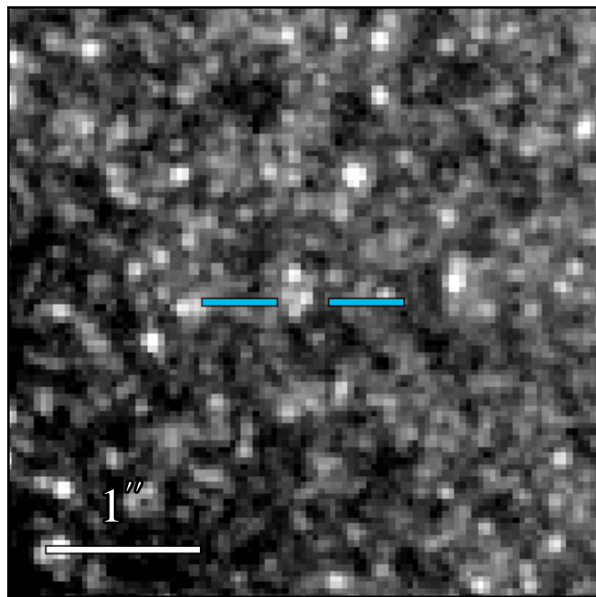
JWST/NIRCam F212N
