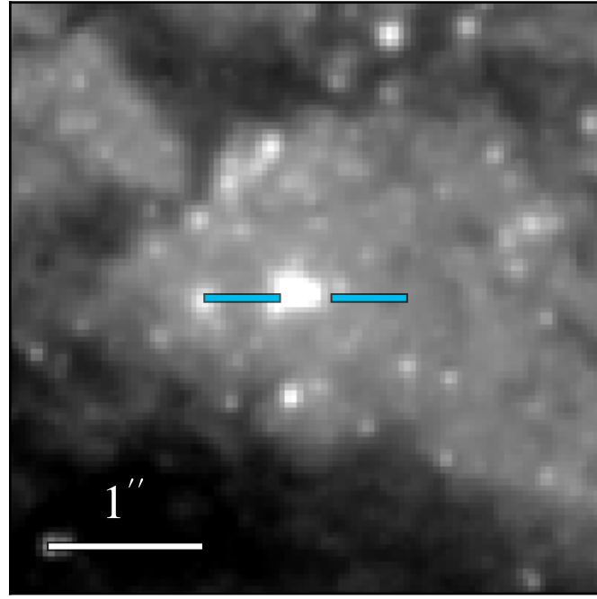
WFC3 F606W 20.909 ± 0.008
