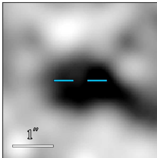
JWST/MIRI F1800W
