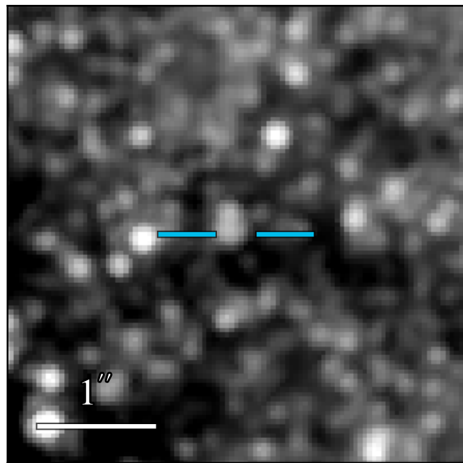
JWST/NIRCam F360M
