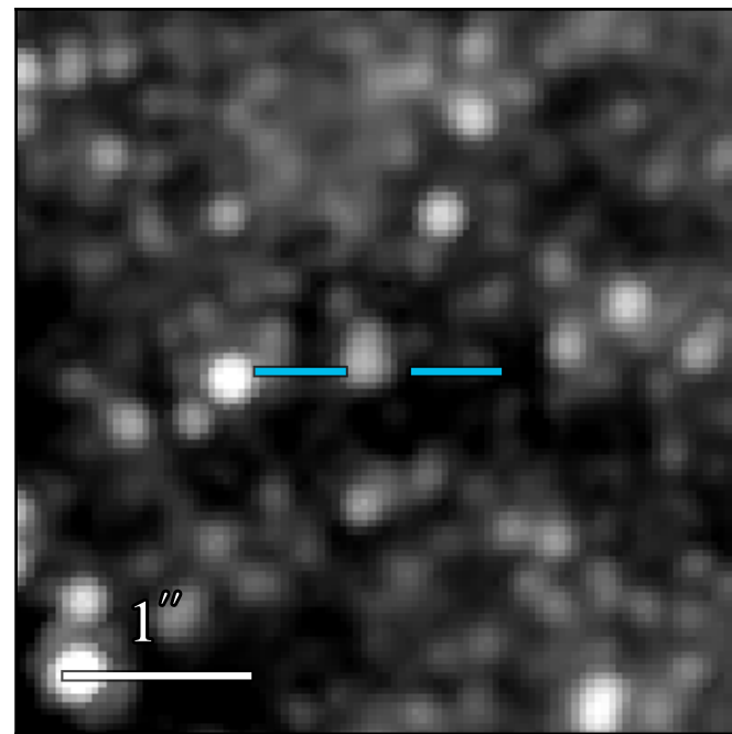
JWST/NIRCam F430M
