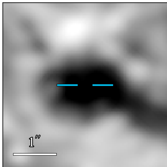
JWST/MIRI F1130W
