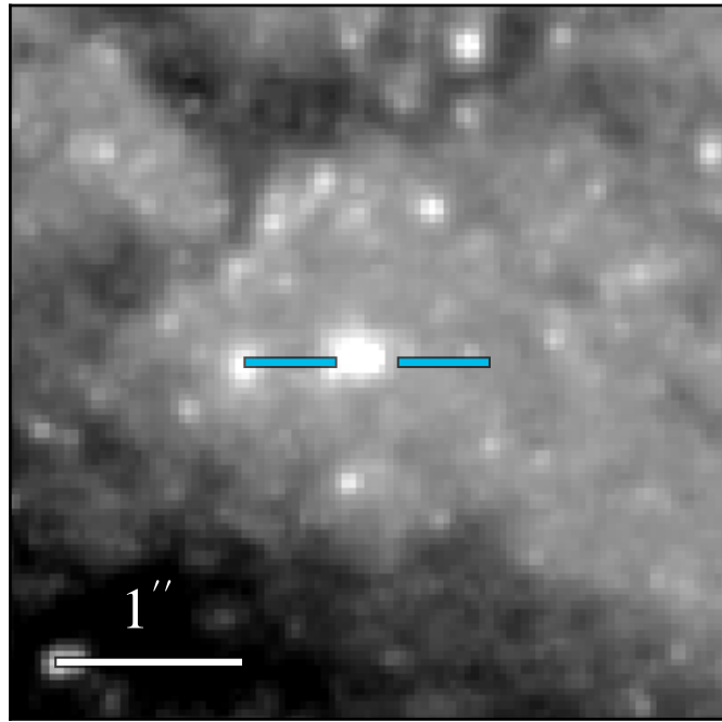
WFC3 F814W 20.389 ± 0.009
