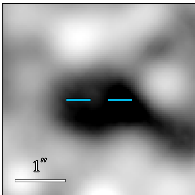
JWST/MIRI F2100W
