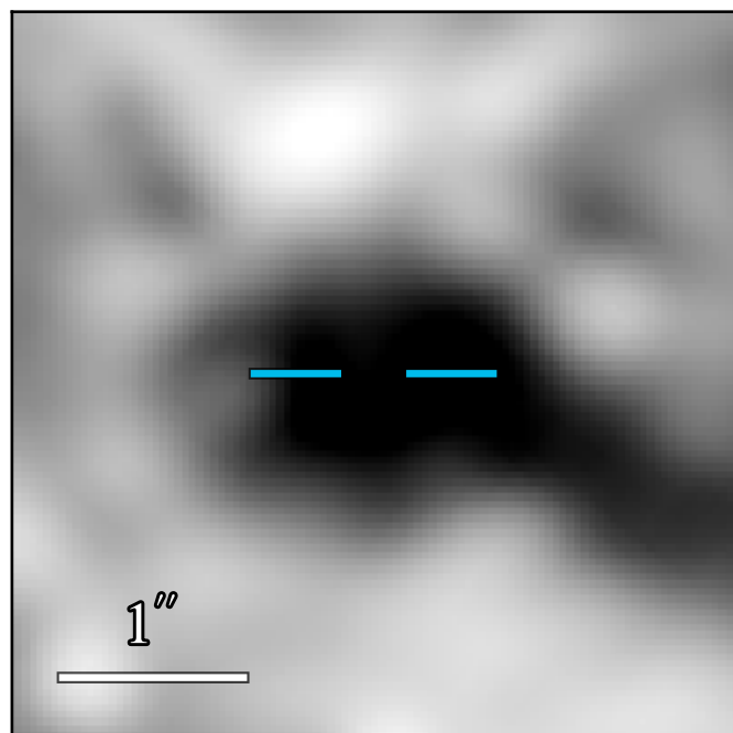
JWST/MIRI F1280W
