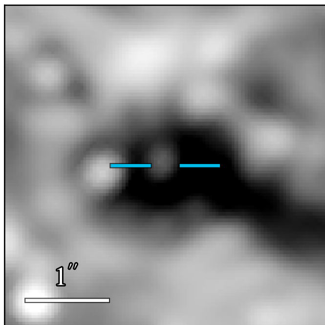
JWST/MIRI F1000W
