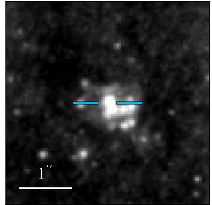
WFC3 F606W 22.289 ± 0.013
