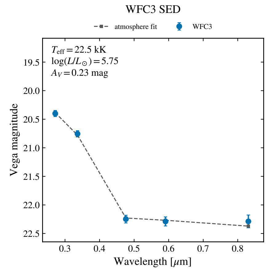
WFC3 F606W 22.289 ± 0.013
