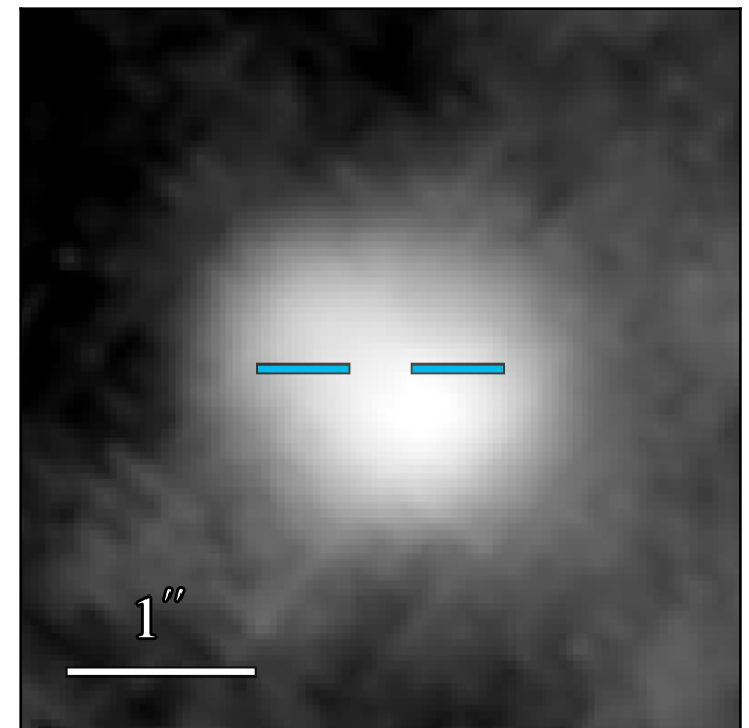
JWST/MIRI F2100W
