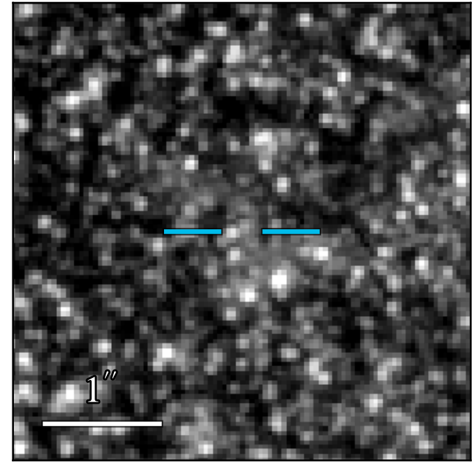
JWST/NIRCam F210M
