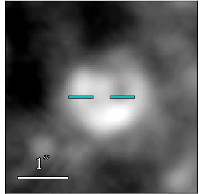
JWST/MIRI F1000W
