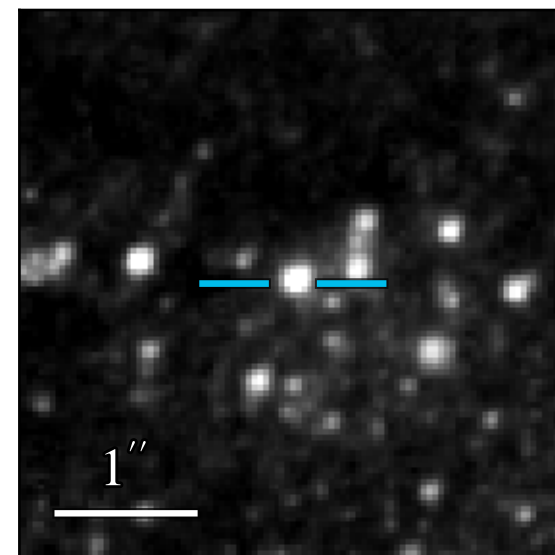
WFC3 F475W 22.218 \pm 0.008
