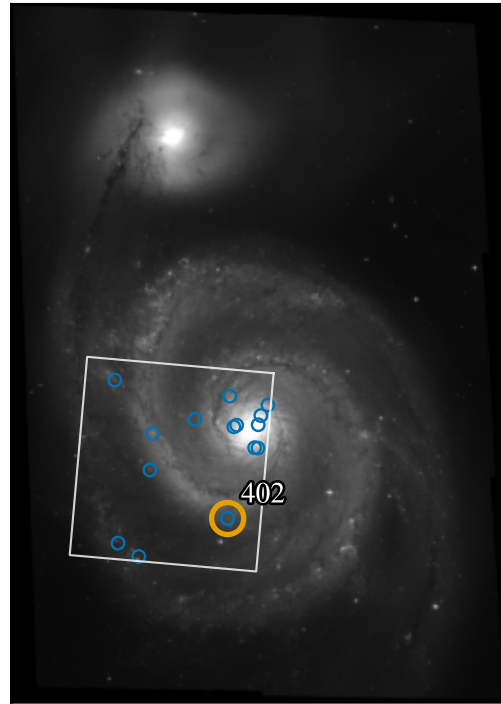
M51 / WFC3 footprint
