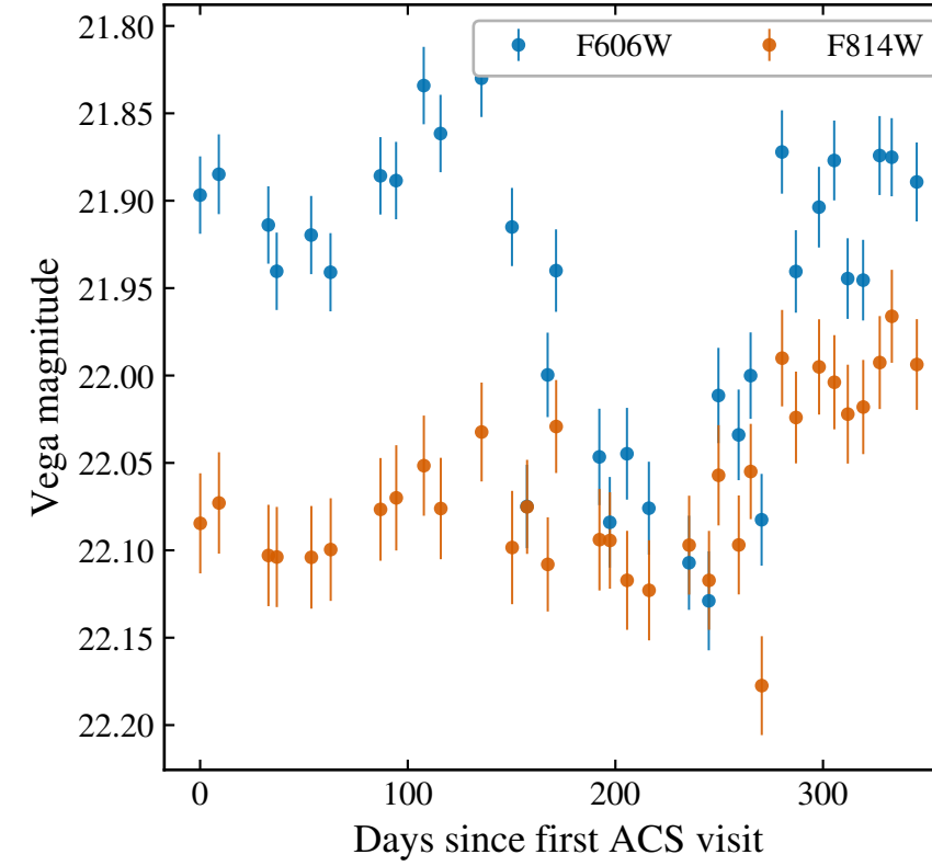
ACS visit light curves
