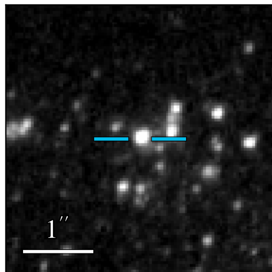
WFC3 F336W 20.676 \pm 0.009
