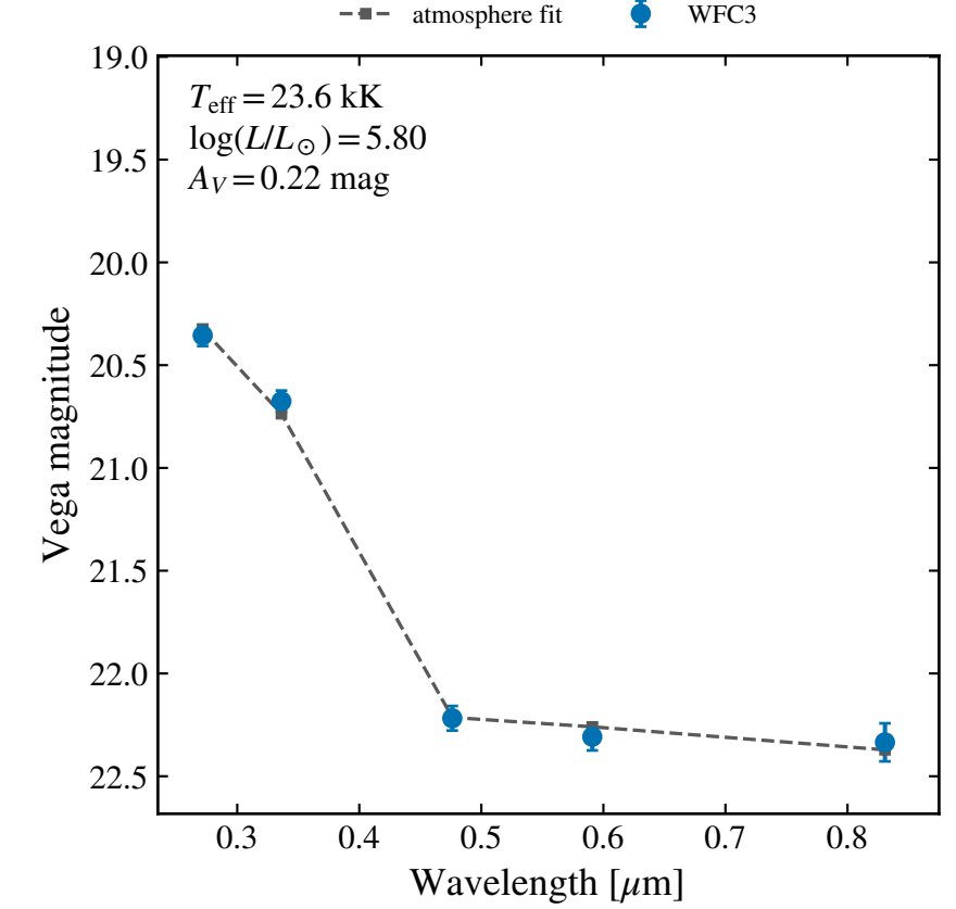
WFC3 SED
