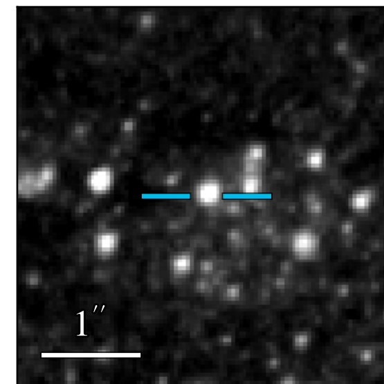
WFC3 F606W 22.308 \pm 0.008
