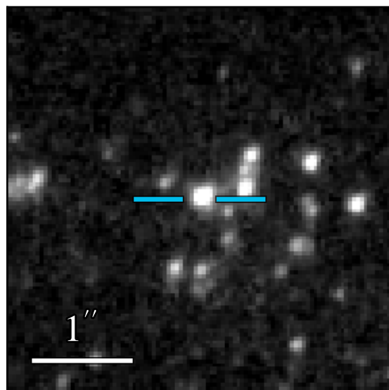
WFC3 F275W 20.355 \pm 0.012
