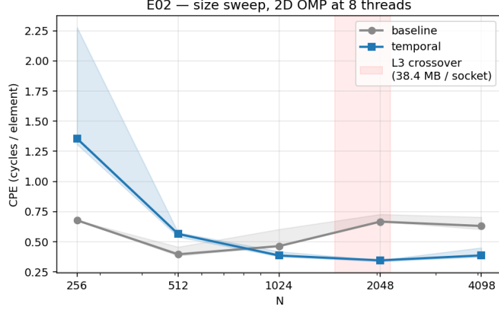
Figure 4: 2D OMP size sweep at 8 threads, B=128 , T=8 , \text{iters}=64 . The L3→DRAM crossover lands between N=1024 and N=2048 : baseline CPE rises from 0.464 to 0.667 as the working set exceeds 38 MB. Temporal stays at \sim 0.35 across N=1024-4098 (L2-resident on its scratch) and wins 1.93\times at N=2048 . Below L3 temporal loses: per-tile malloc + halo work cancel the savings on a working set the baseline already had in cache.
