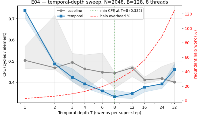
Figure 6: Temporal depth T sweep at N=2048 , B=128 , 8 threads, iters=96. Left axis: CPE. Right axis: redundant halo work, ((B+2T)^2/B^2 - 1) \cdot 100 . Optimum at T=8 , CPE 0.332.
