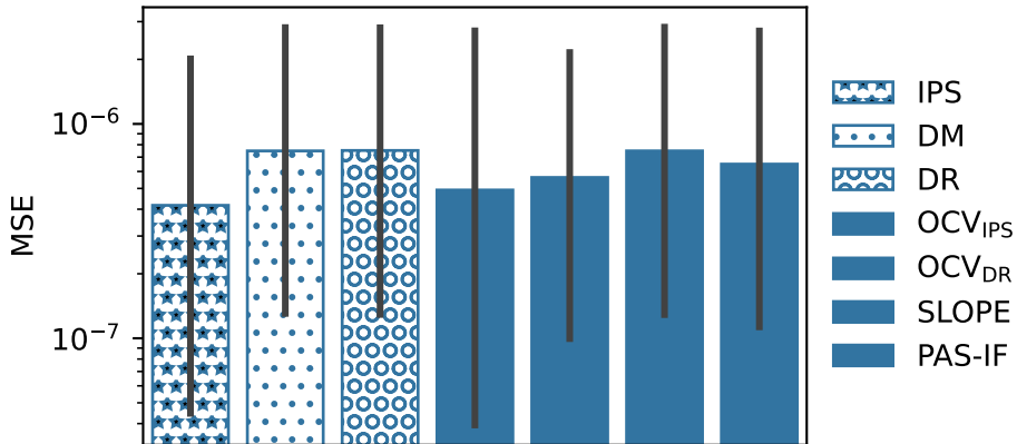
Performance on Open Bandit Dataset
