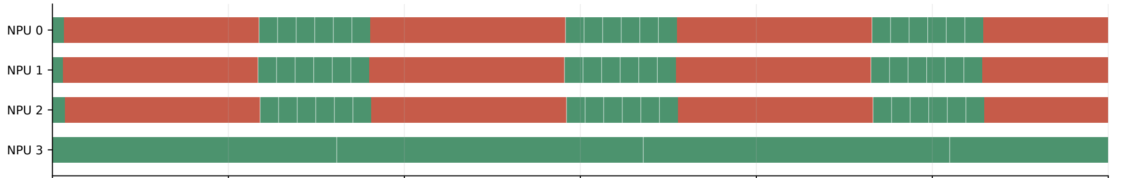
Once (5 ms): actual compute and exposed I/O stall
