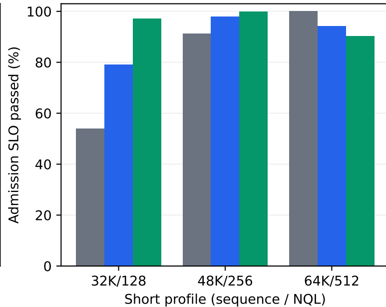
raw_size_varied_rho097_seed7 Same complete request-ID cohorts; synthetic t=0 backlog
