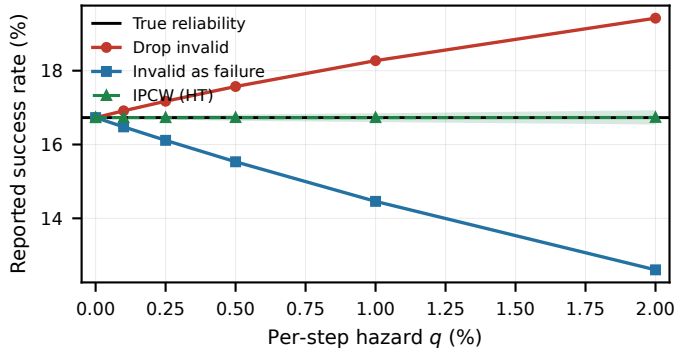
(a) SWE-agent, n=80,036 \bar{H} : 15.2 vs 28.7
