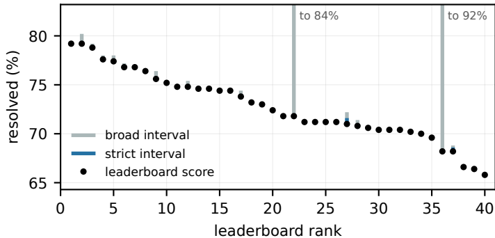
(a) SWE-bench Verified, top 40 of 135
