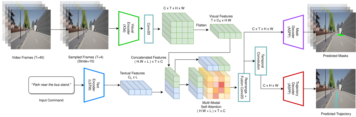
Figure 4.3: Multi-frame Conv3D/X3D model: sampled video frames through X3D, multimodal self-attention with LSTM language features, temporal convolution, and dual ASPP heads.
