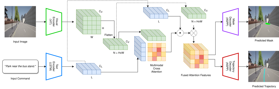
Figure 4.2: Per-frame ViT baseline: Vision Transformer visual encoder, LSTM language encoder, multimodal attention, and dual ASPP heads for navigable-region and trajectory masks.
